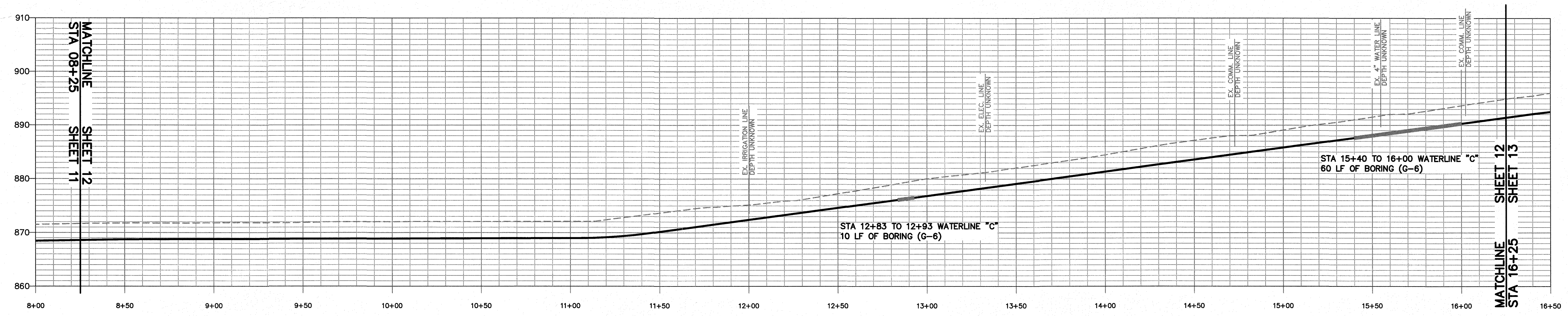
WATERLINE "C" SCALE: VERTICAL: 1" = 10' HORIZONTAL: 1" = 30'
