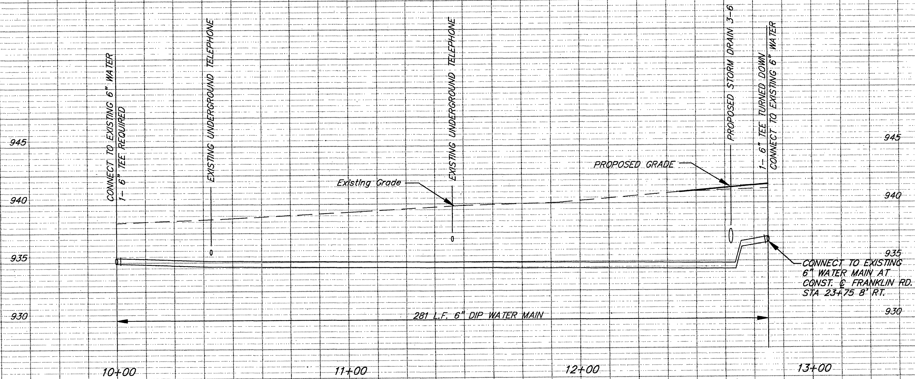
PROPOSED WATER MAIN PROFILE SCALE: 1"=25' H., 1"=5' V.
