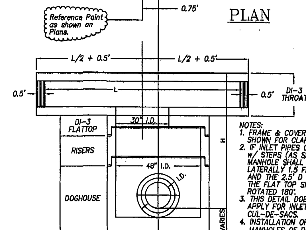
LOCATION DETAIL FOR DI-3A AND DI-3C (PRECAST) NO SCALE
