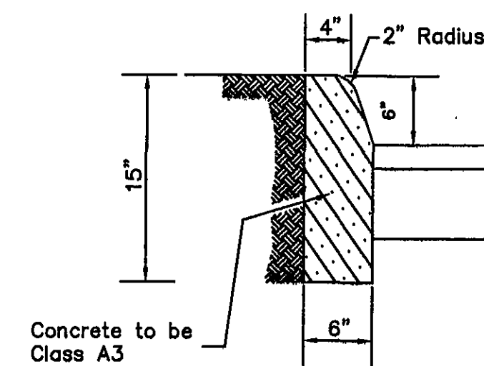
CONCRETE CURB (CG-2) NO SCALE
