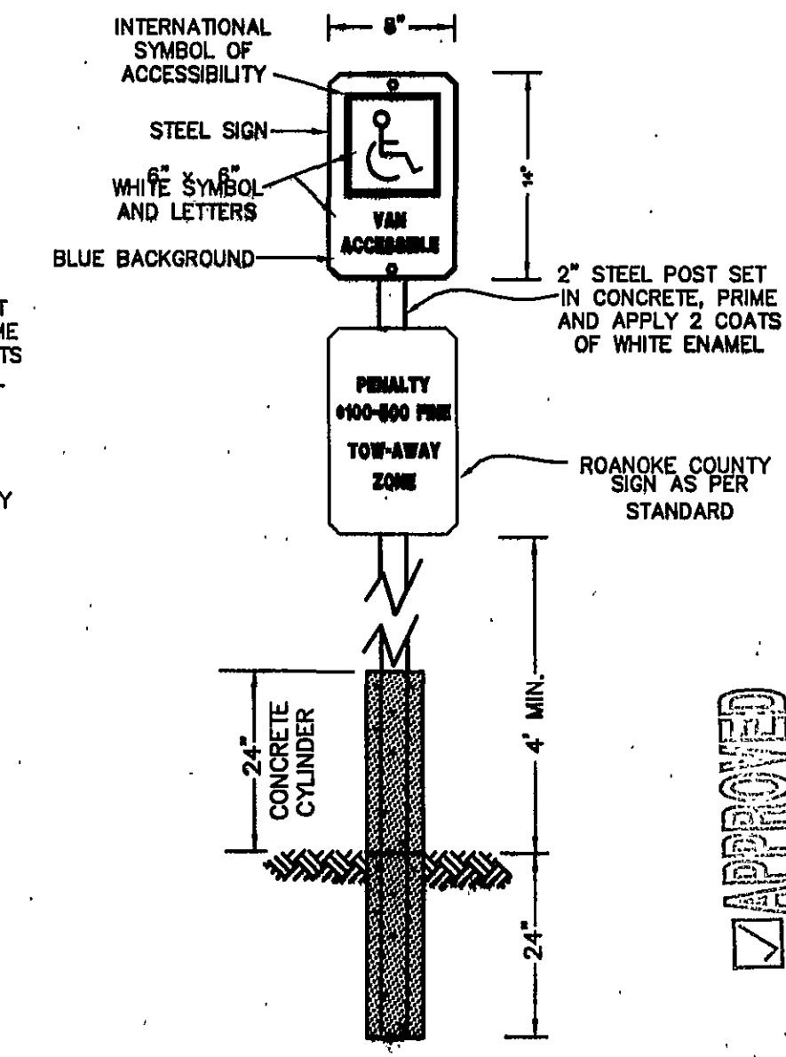
VAN ACCESSIBLE HANDICAP PARKING SIGN (S2) NO SCALE
