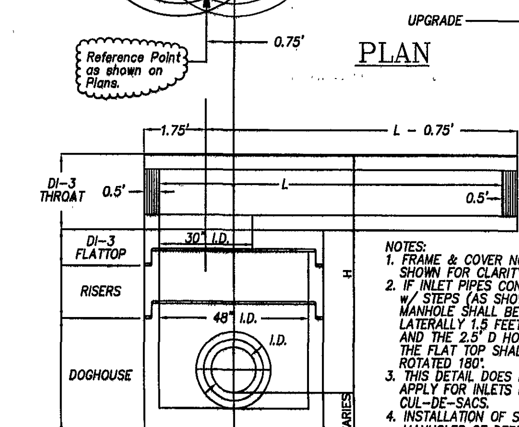
LOCATION DETAIL FOR DI-3B (PRECAST) NO SCALE
