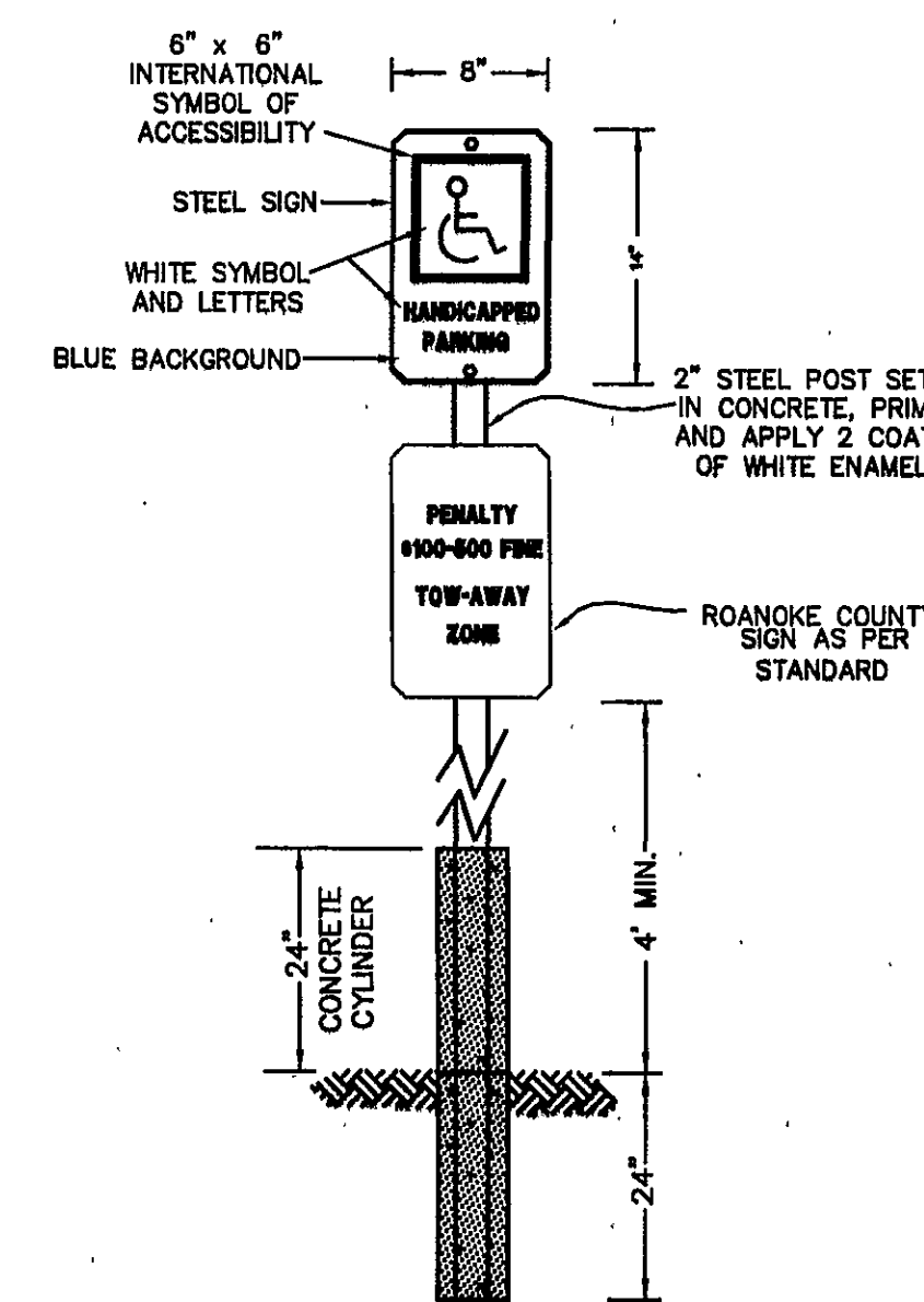
HANDICAP PARKING SIGN (S1) NO SCALE
