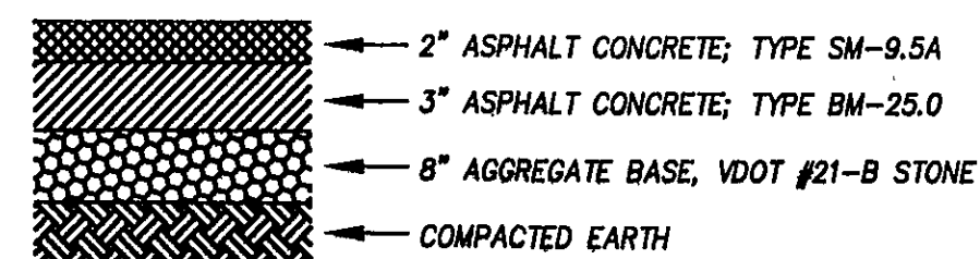
PAVEMENT DETAIL TYP. ALL PAVEMENT NO SCALE
