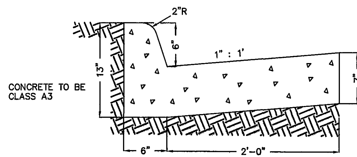
CONCRETE CURB + GUTTER (CG-6) NO SCALE
