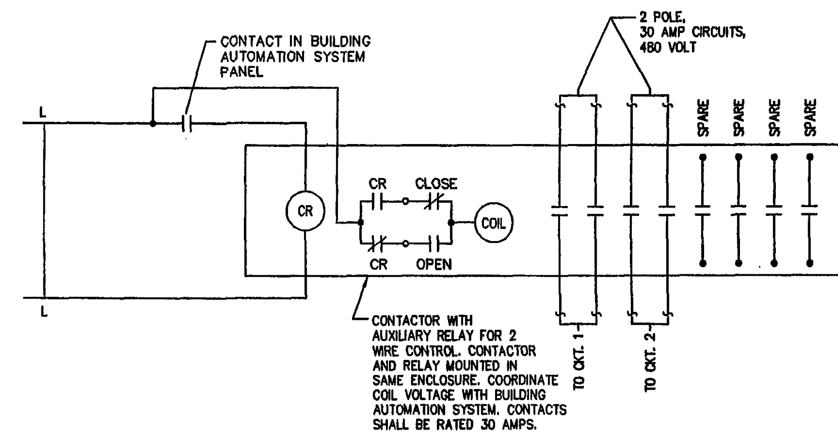
WIRING DIAGRAM FOR LIGHTING CONTACTOR LC-1 NO SCALE
