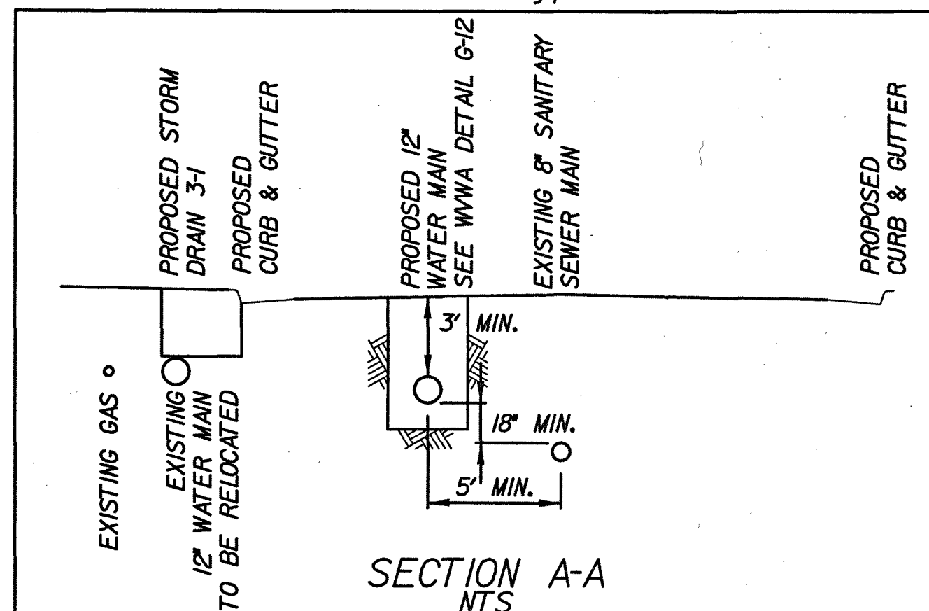
Water Main Relocation Typical Cross-Section
