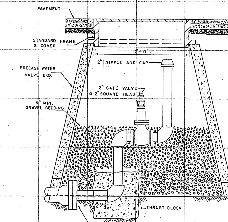
PERMANENT END OF LINE NO SCALE
