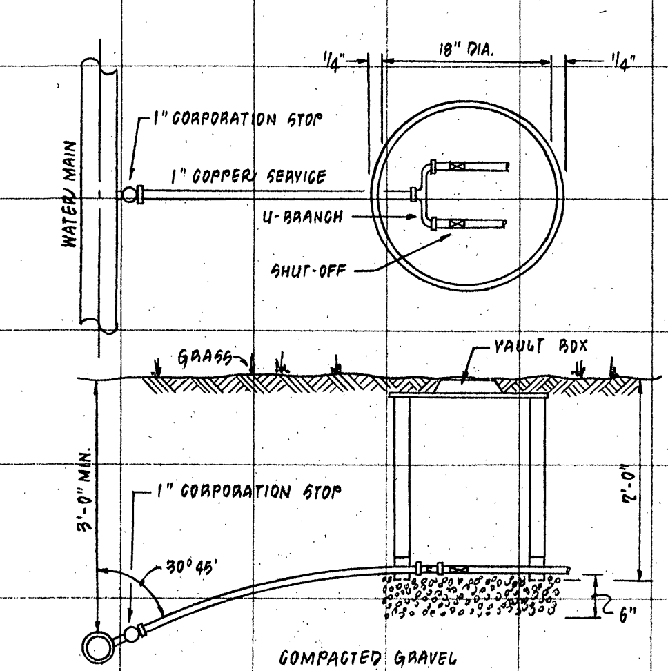
DOUBLE WATER SERVICE NO SCALE
