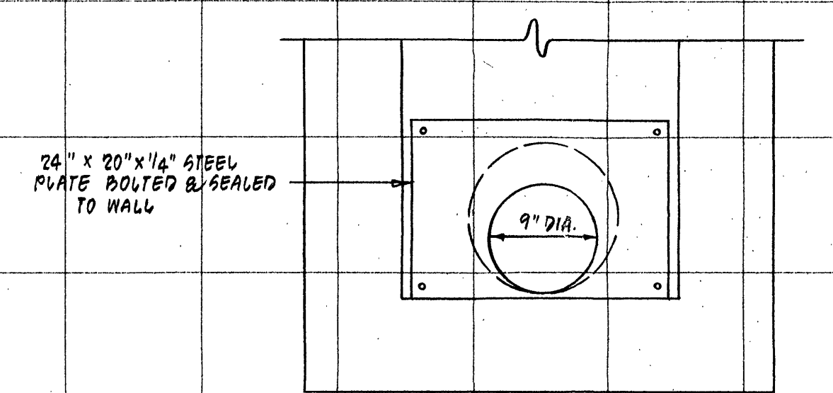
DETAIL OF RESTRICTOR PLATE IN INLET C NO SCALE
