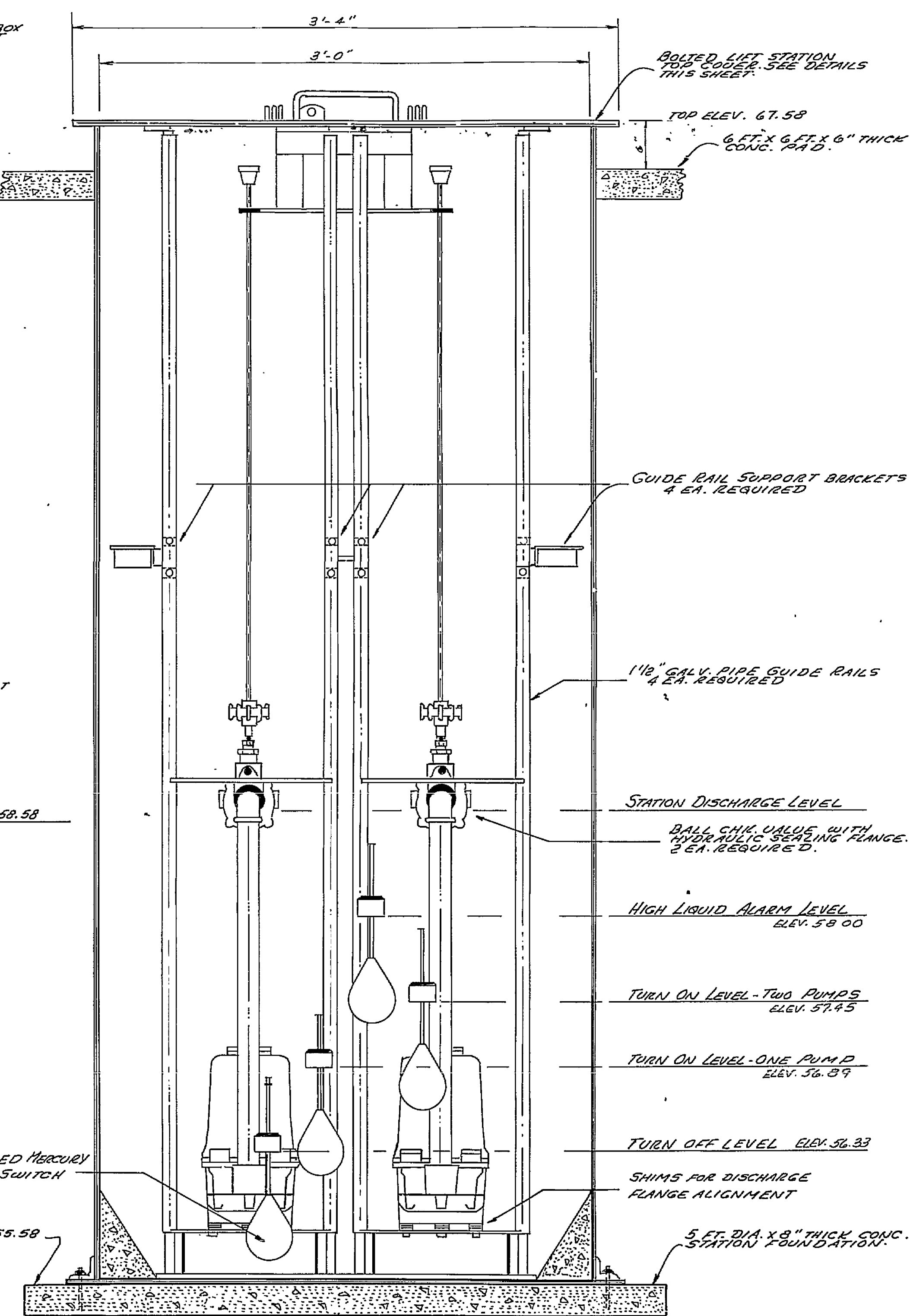
SECTION B-B
