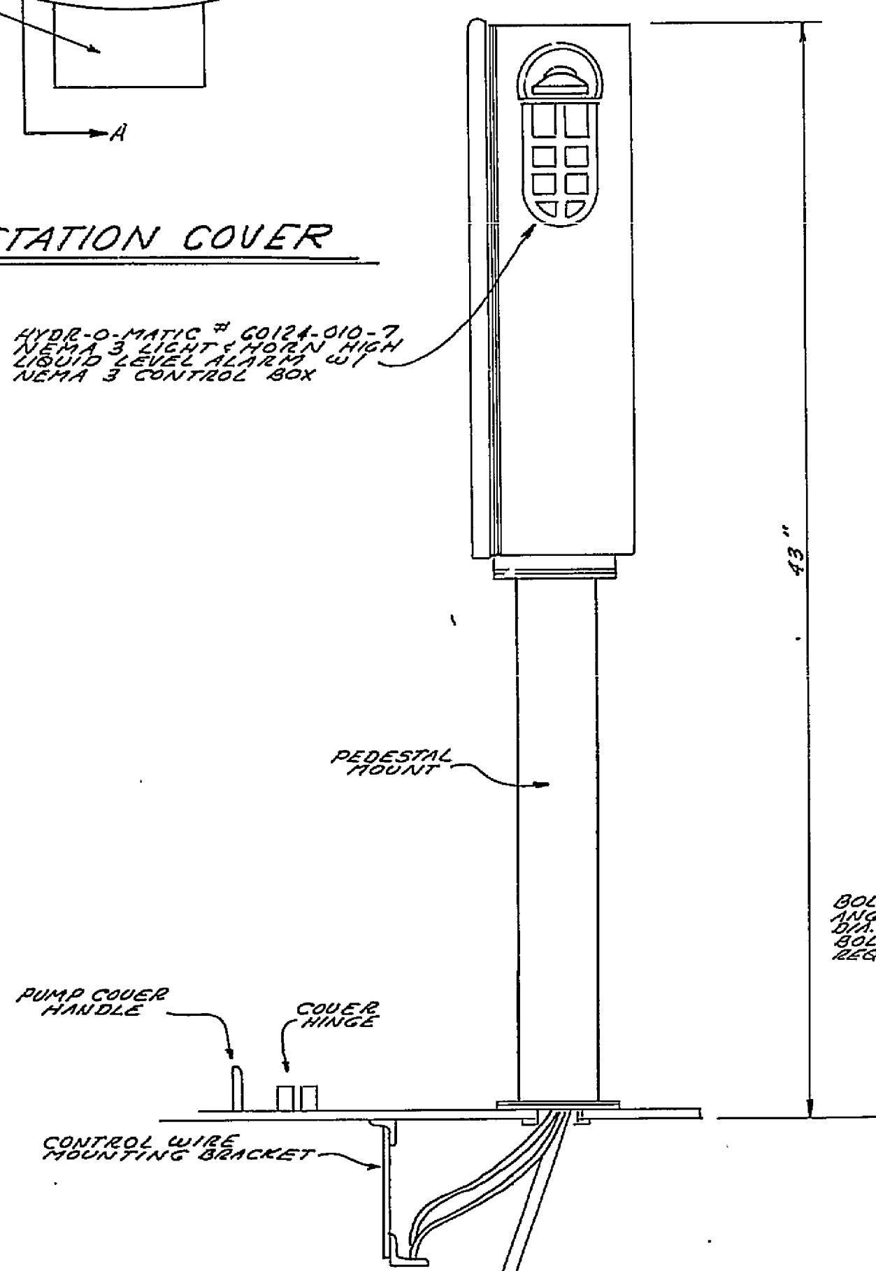
CONTROL BOX & ALARM MOUNT
