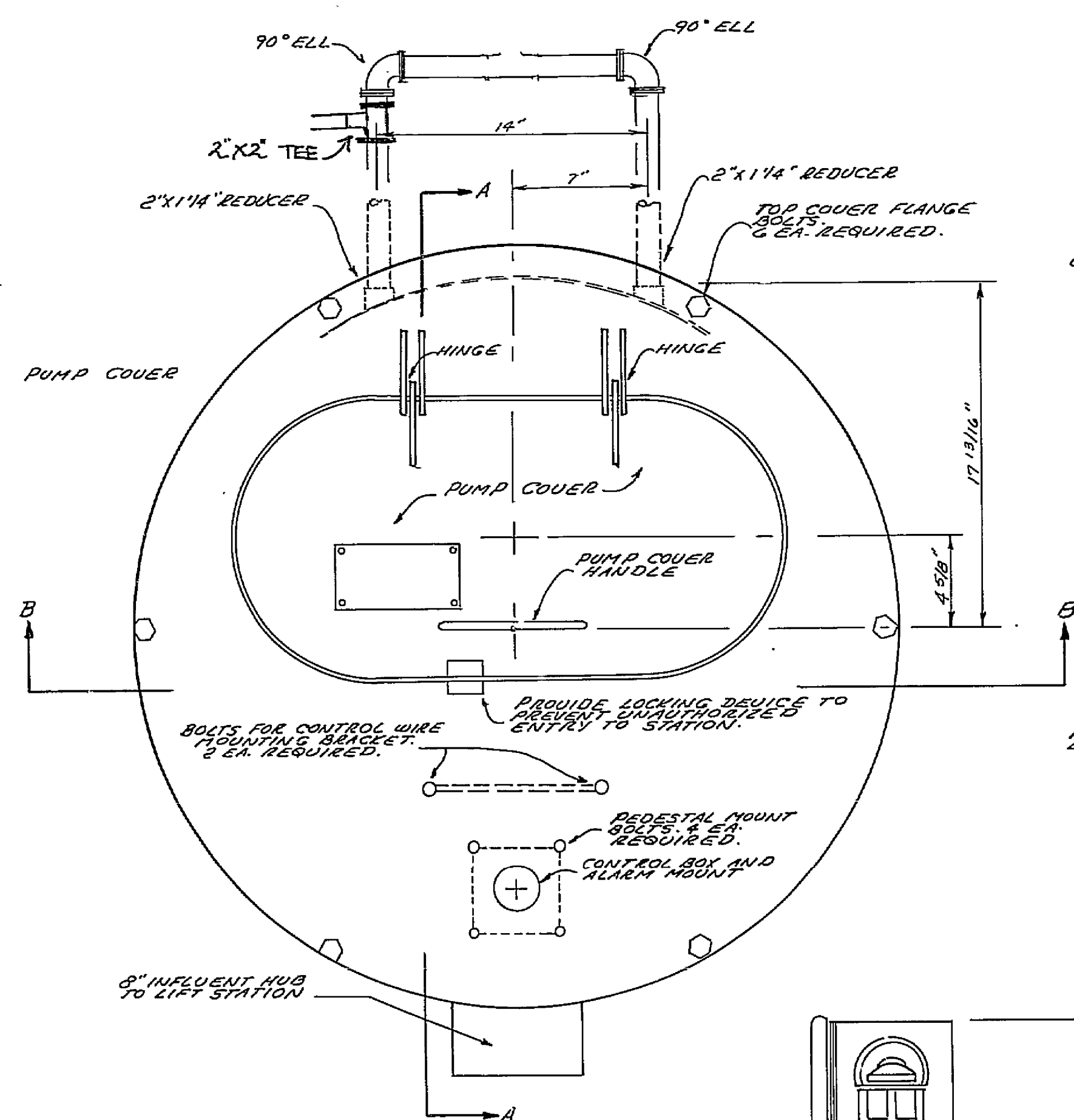
TOP VIEW - LIFT STATION COVER
