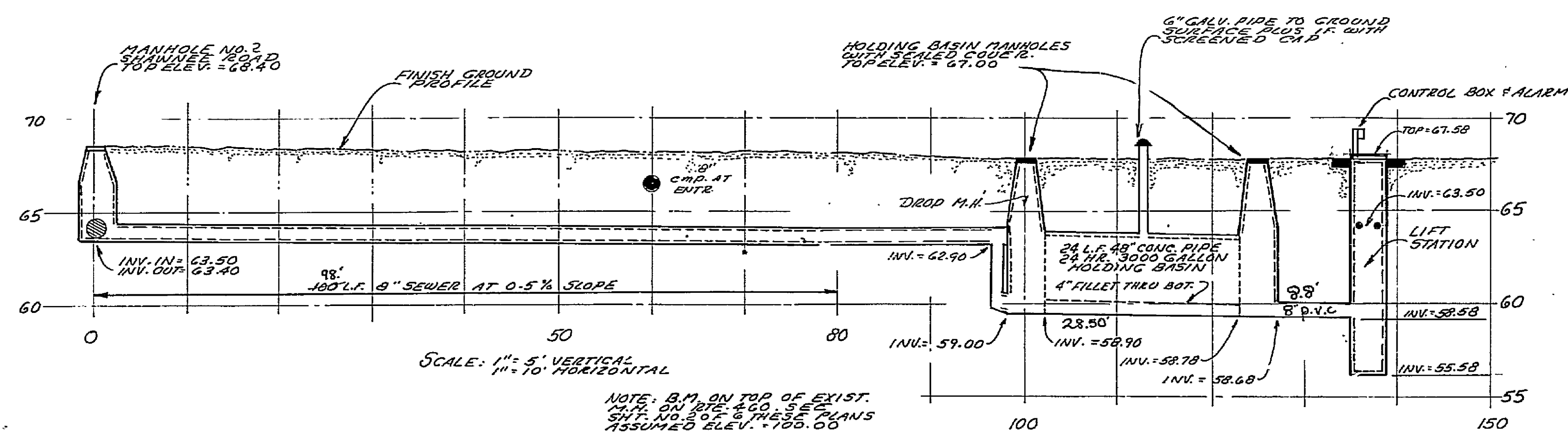
SEWER PROFILE - MANHOLE NO. 3 TO PUMP STATION
