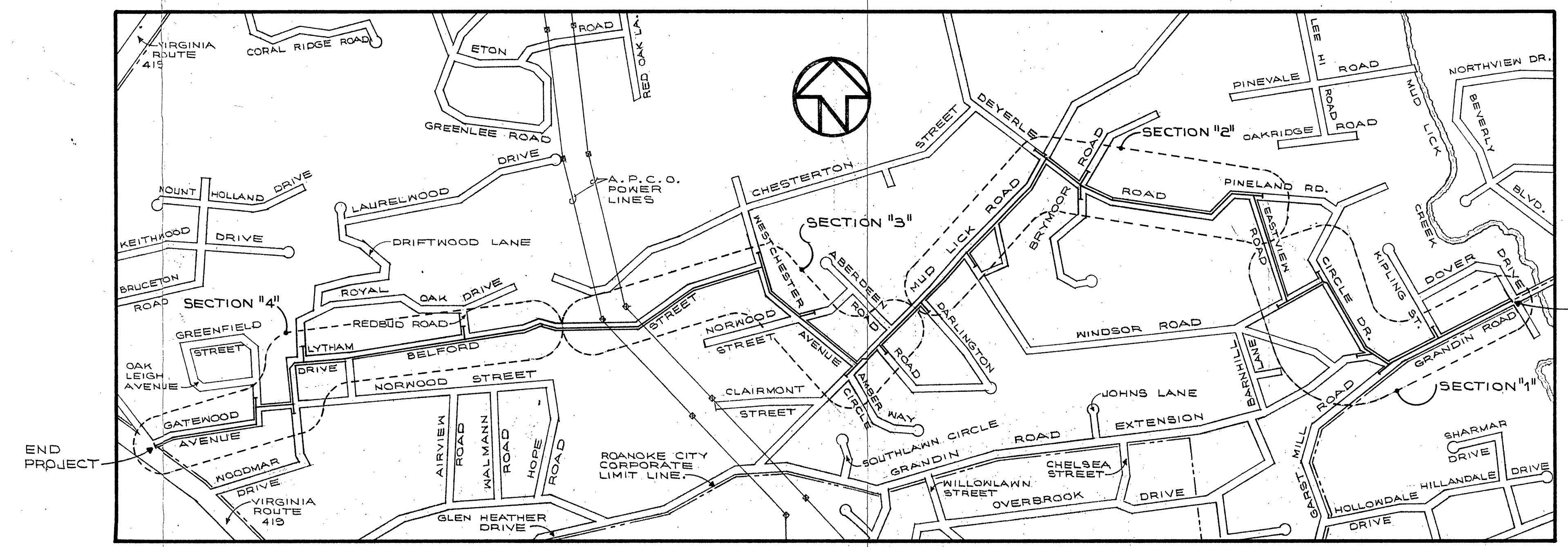
VICINITY MAP 500' 0' 500' 1000'
