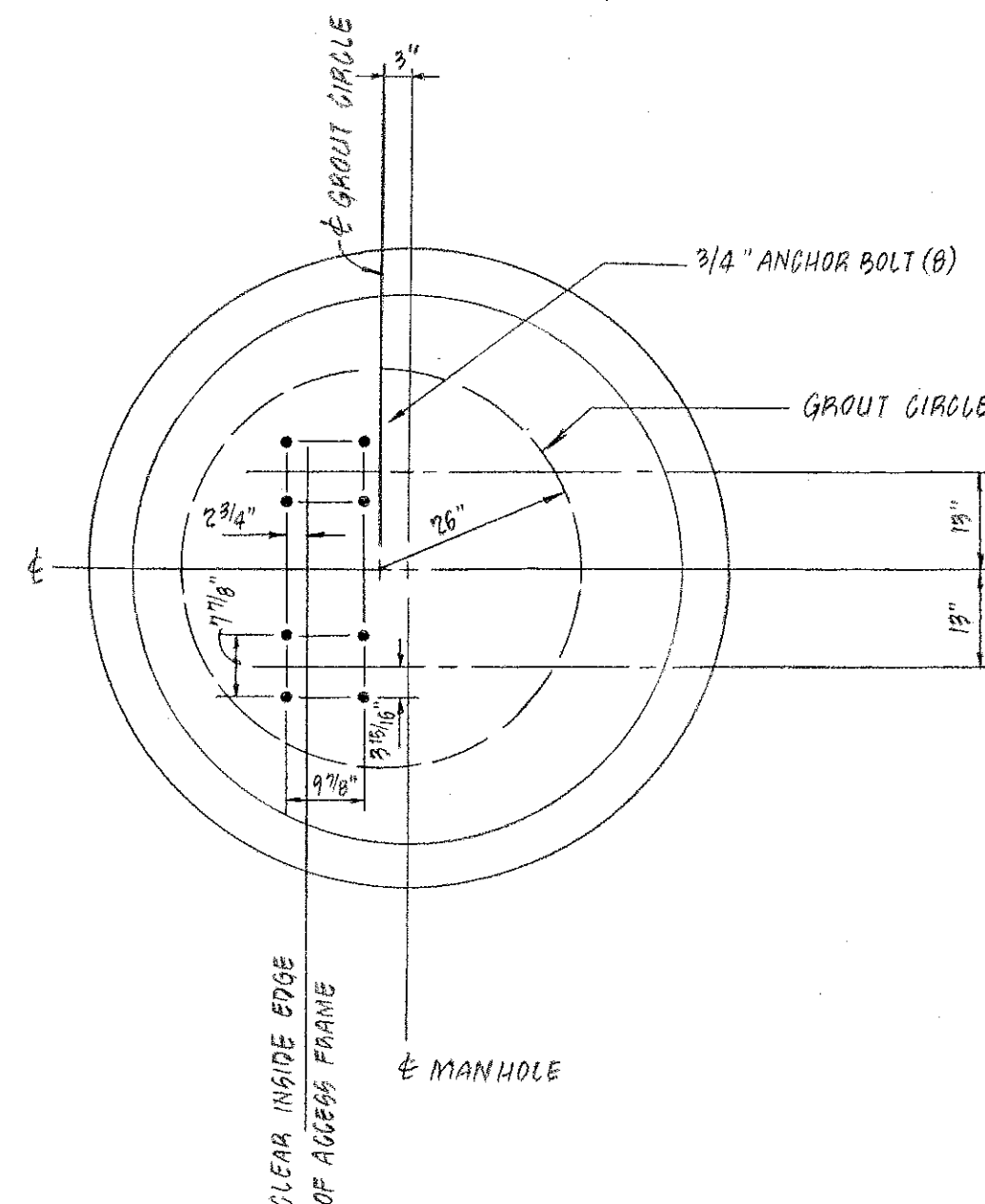
BASE DETAIL
