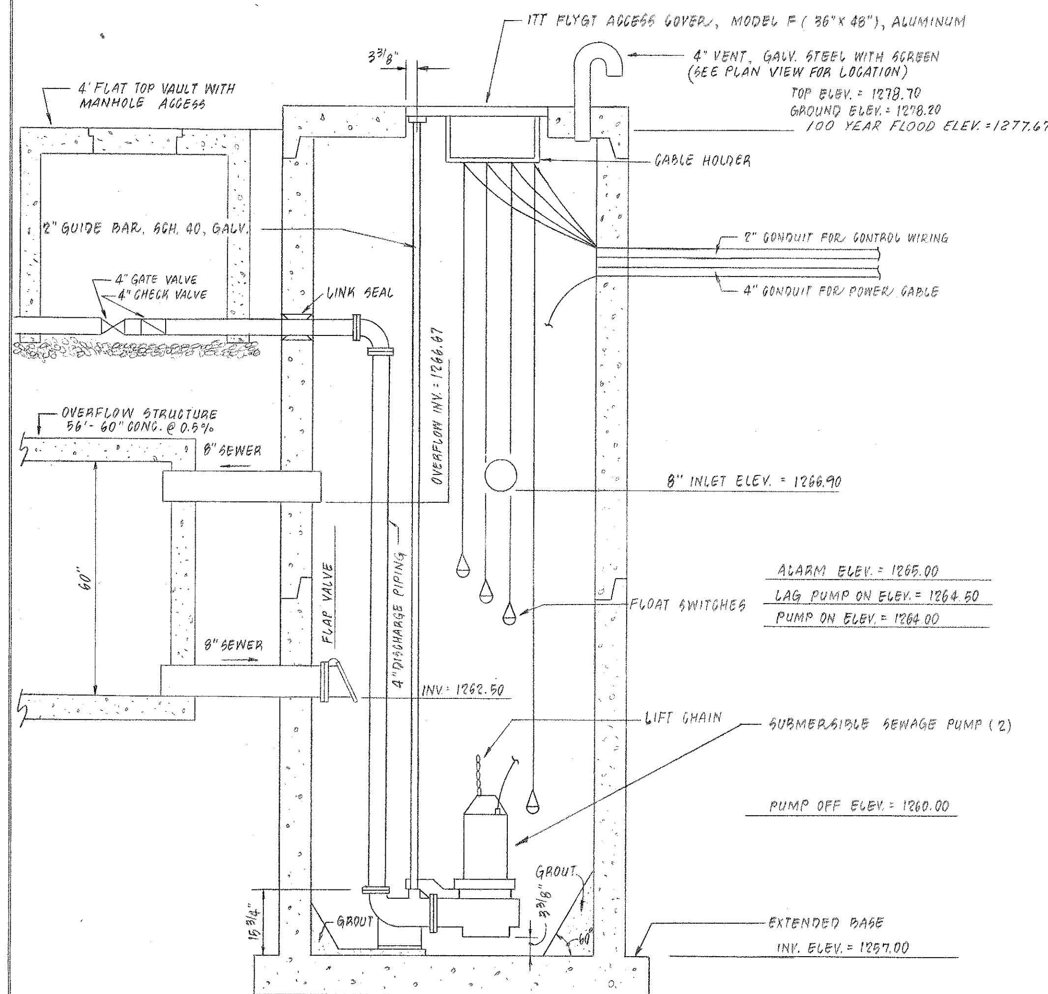
SECTION "A-A"
