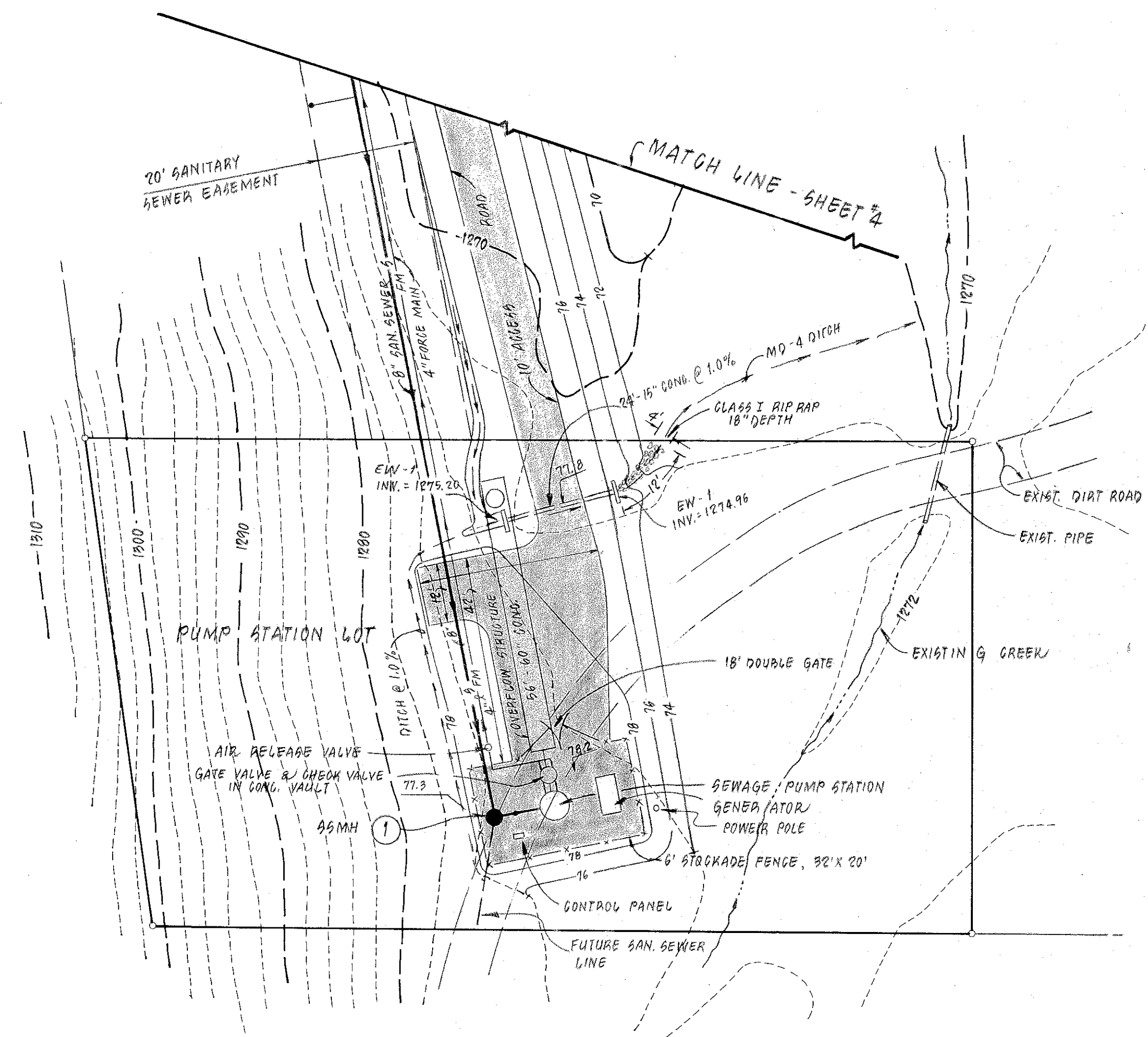
SITE PLAN
