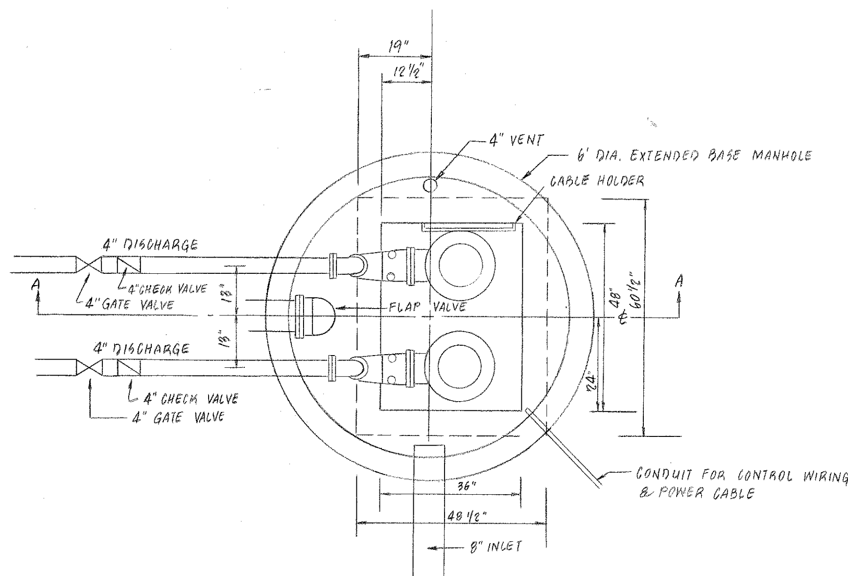
PLAN
