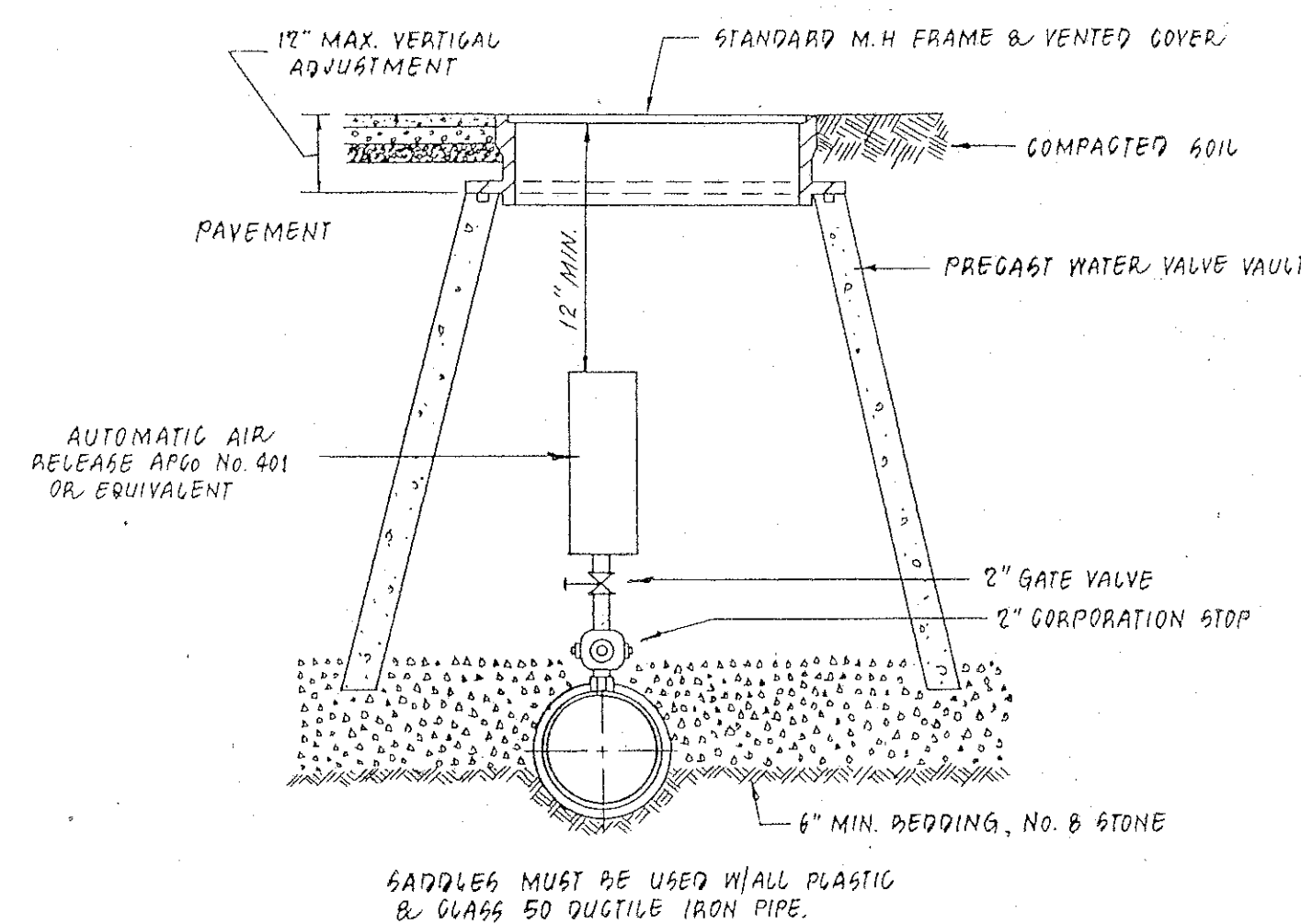
AUTOMATIC AIR RELEASE ASSEMBLY
