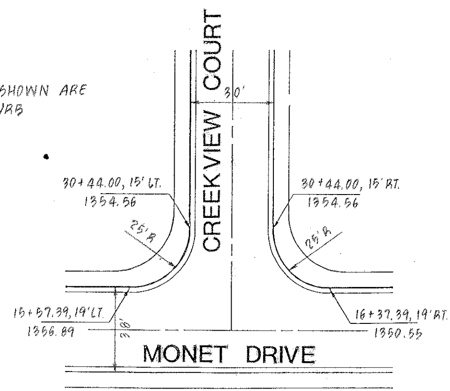
INTERSECTION DETAIL
