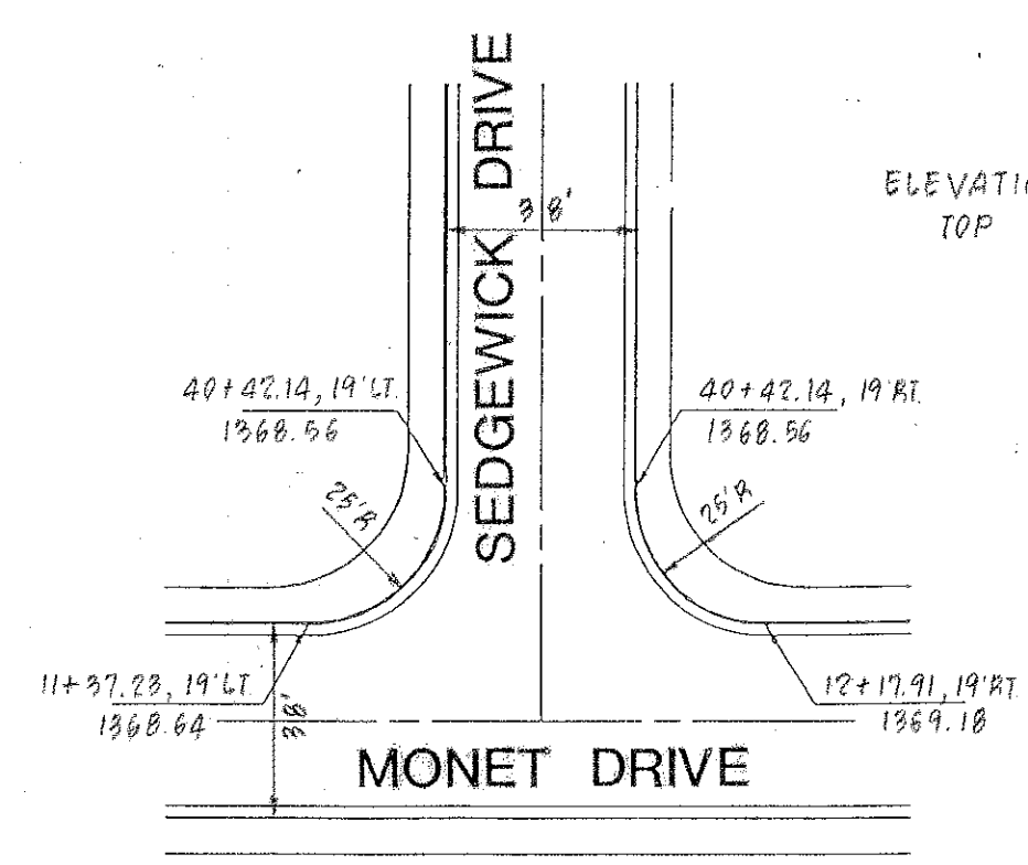
INTERSECTION DETAIL
