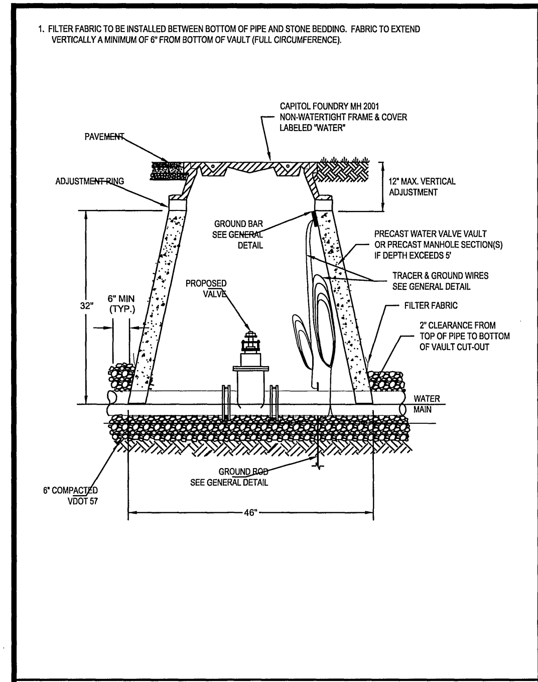
WESTERN VIRGINIA REGIONAL - CONSTRUCTION DETAIL WATER LINE VALVE & VAULT 01/01/12 W-9
