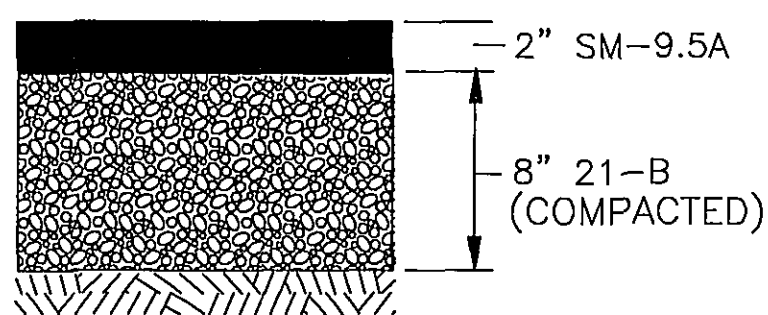
ASPHALT PAVEMENT SECTION NO SCALE
