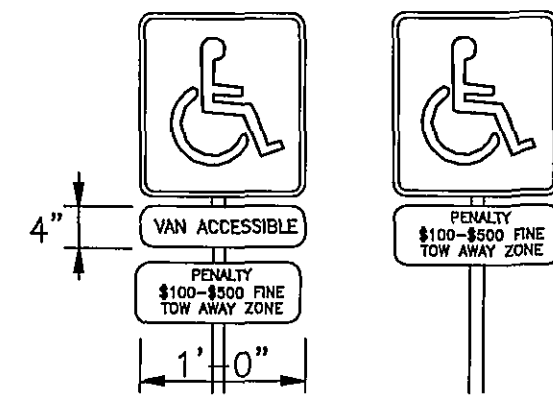
HANDICAP SIGN NOTES: 1. EACH SIGN SHALL BE POST MOUNTED TO A POLE WITH NO SIGN EDGE LOWER THAN 4' AND NO HIGHER THAN 7' TO THE FINISHED GRADE. 2. ALL SIGNS SHALL BE REFLECTORIZED. 3. ALL SIGNS SHALL BE SECURELY MOUNTED TO A GALVANIZED STEEL CHANNEL POST. HANDICAP SIGN DETAIL NO SCALE
