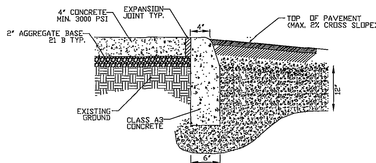
PARKING AREA SIDEWALK DETAIL NO SCALE
