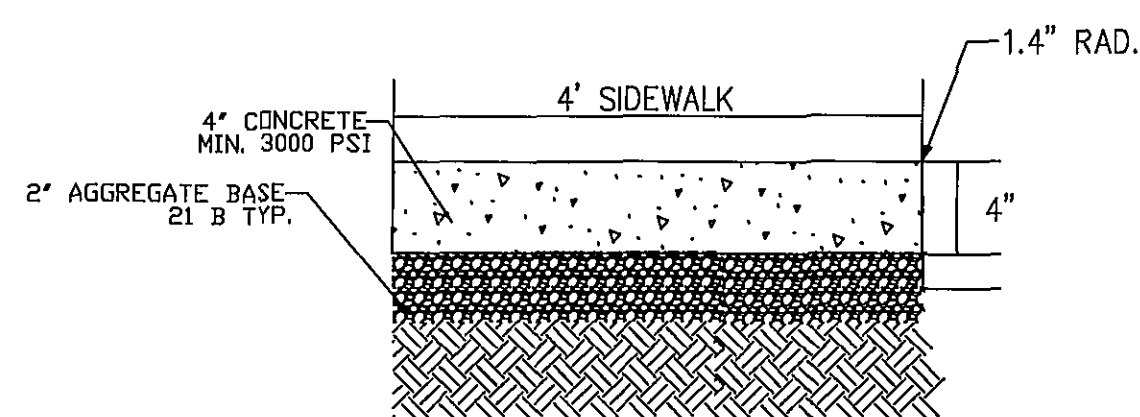
NOTE: FINISH - TROWELED EDGES, BROOM FINISH SCORING EVERY 6' EXPANSION JOINTS EVERY 30' MIN. NOTE: G.C. SHALL BE RESPONSIBLE FOR OBTAINING ADEQUATE SUB-GRADE COMPACTION. SIDEWALK DETAIL N.T.S.
