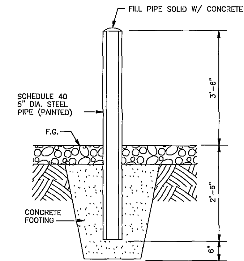
PIPE BOLLARD DETAIL NO SCALE
