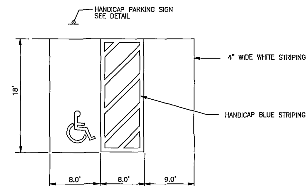
HANDICAPPED PARKING DETAIL N.T.S.
