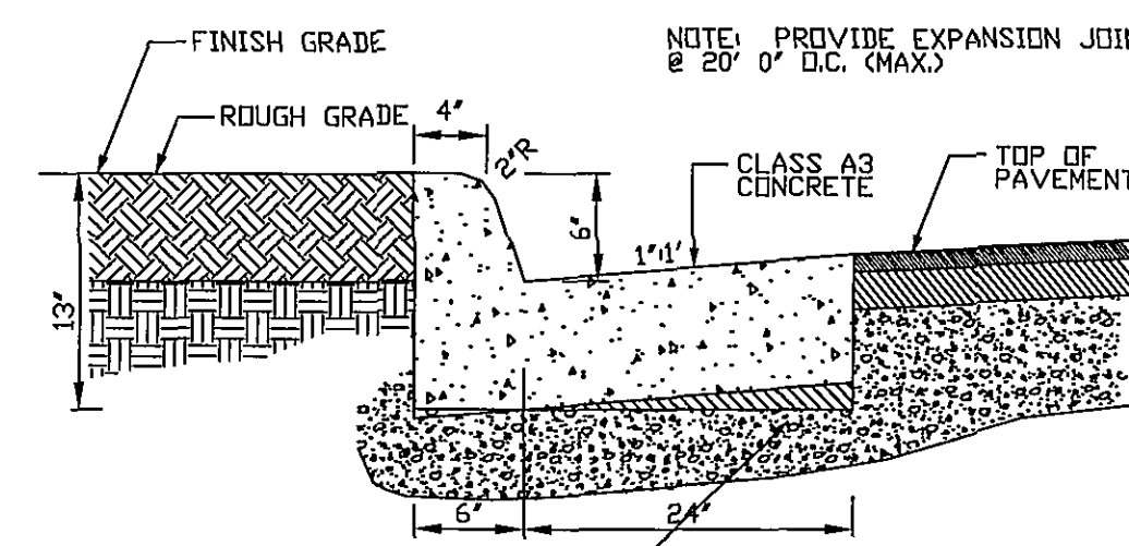
CG-6 (WET) DETAIL N.T.S.
