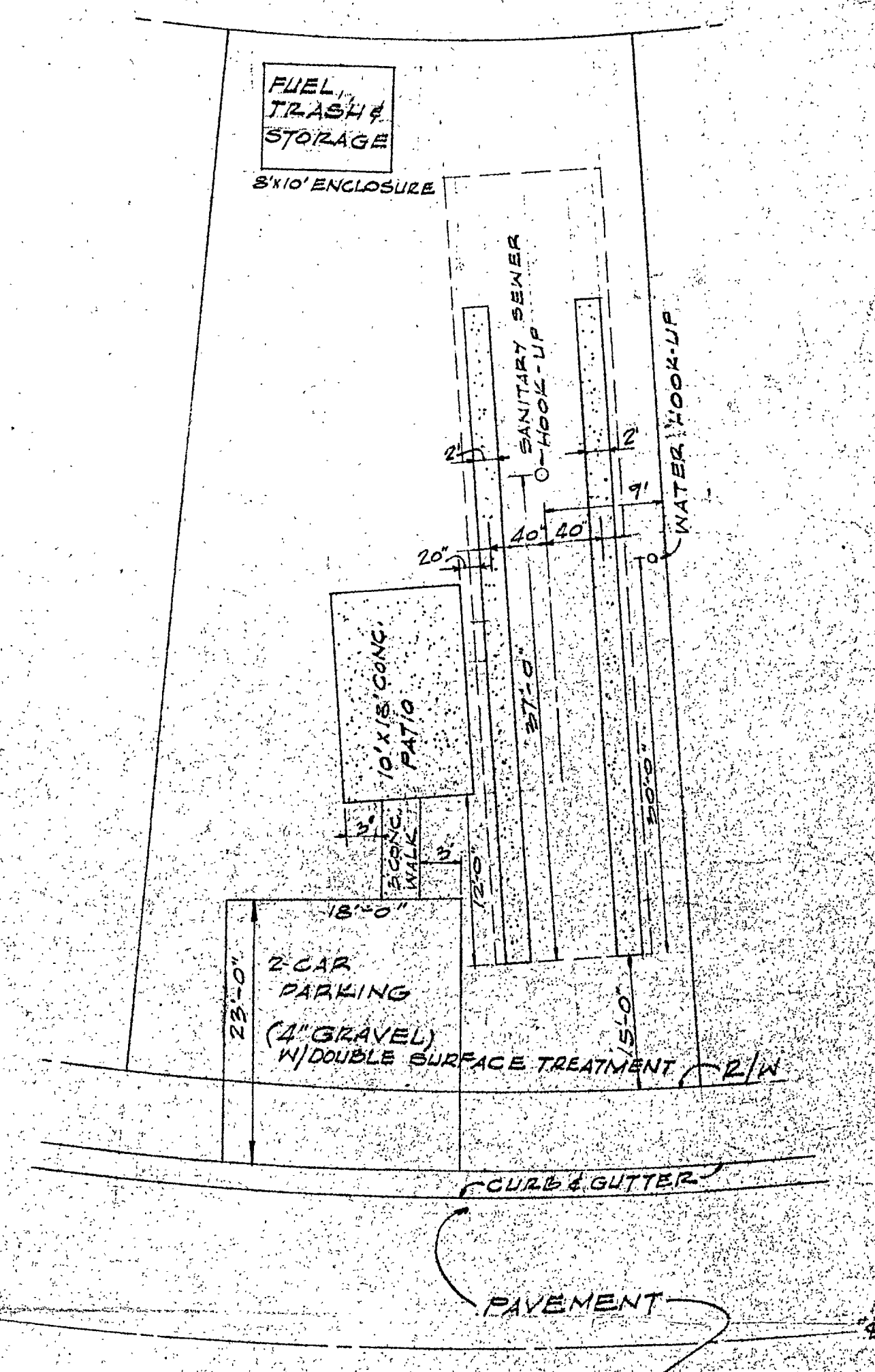
Typical Mobile Home Stand A SCALE: NONE
