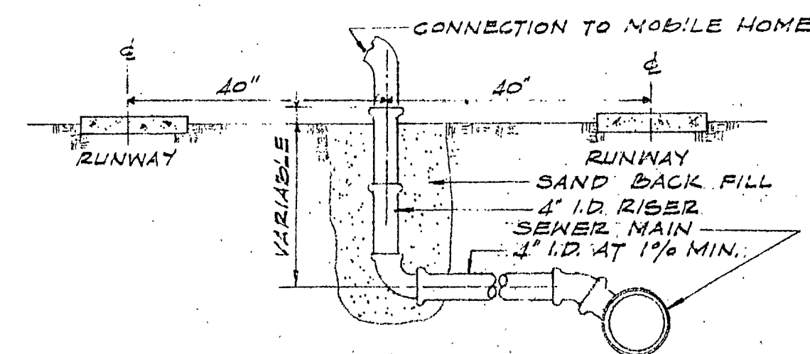
DETAIL OF SANITARY SERVICE CONNECTION SCALE: NONE
