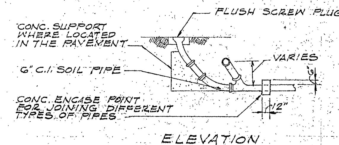
CLEANOUT & CONNECTION DIAGRAM NO SCALE
