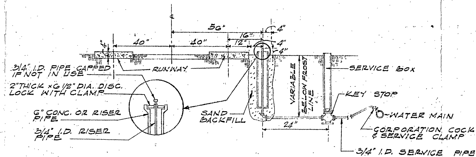
DETAIL OF WATER CONNECTION SCALE: NONE
