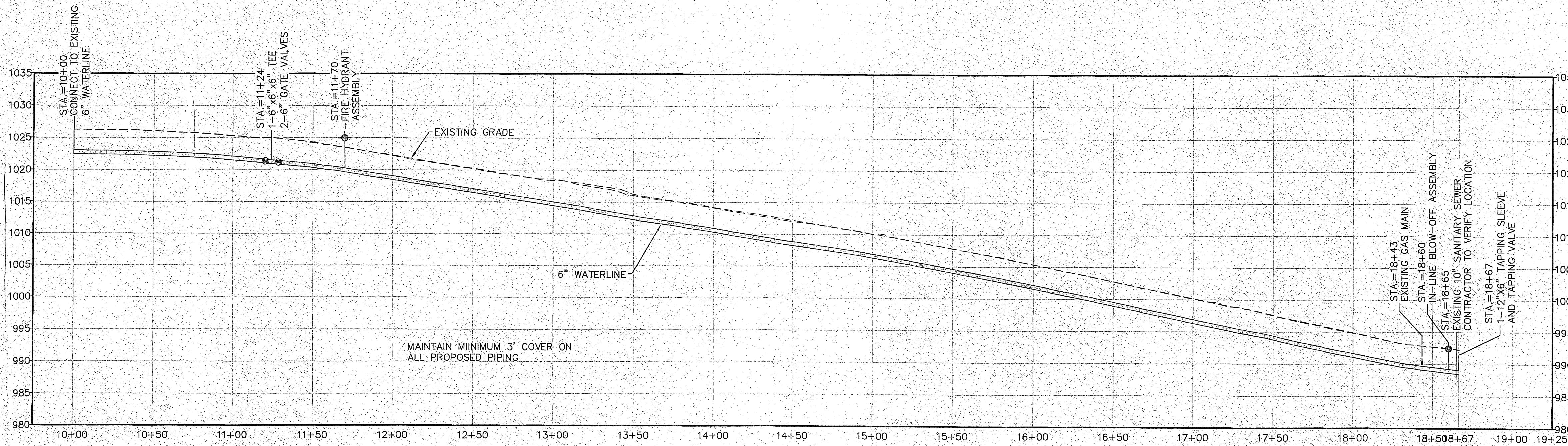
MCDOWELL AVENUE PROFILE SCALE: H: 1"=40', V: 1"=10'
