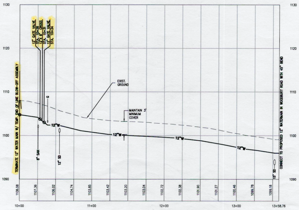
12 INCH WATERLINE - MAITLAND AVE. PROFILE
