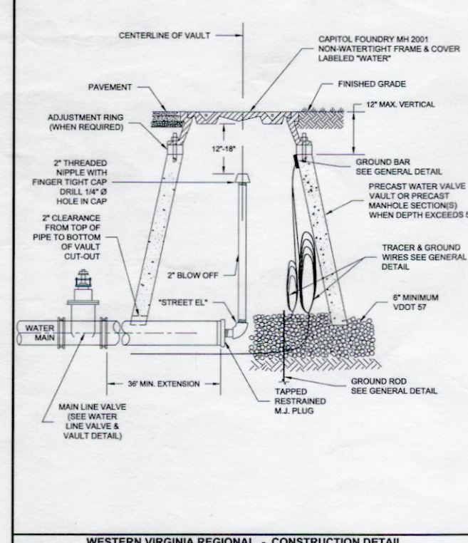
WESTERN VIRGINIA REGIONAL - CONSTRUCTION DETAIL TEMPORARY END OF LINE BLOW-OFF ASSEMBLY W-11
