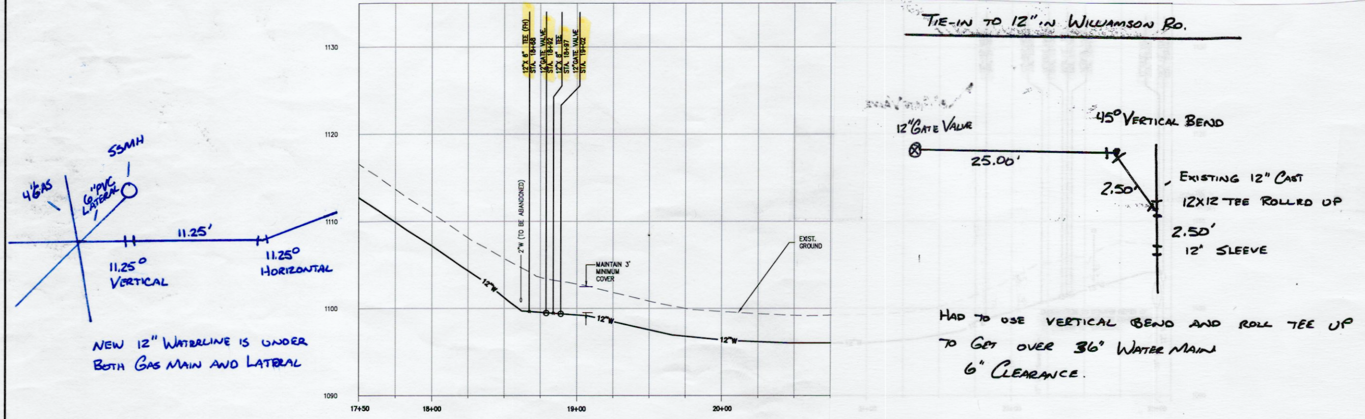
12 INCH WATERLINE - NELMS LANE PROFILE
