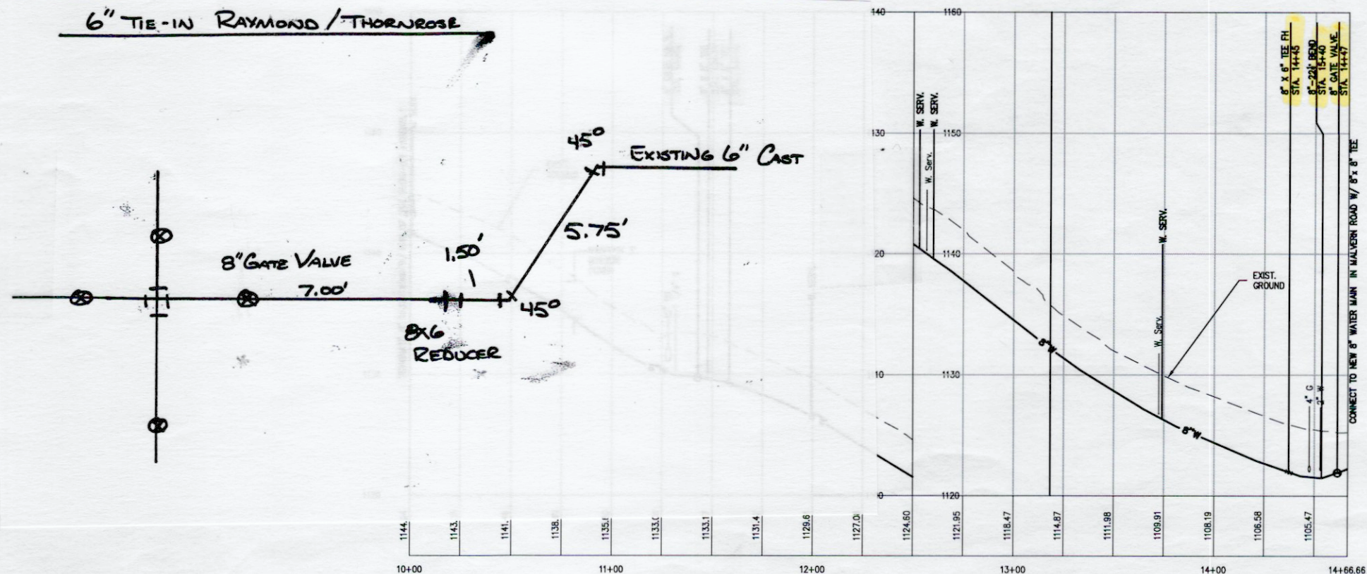
8 INCH WATERLINE - RAYMOND AVE. PROFILE
