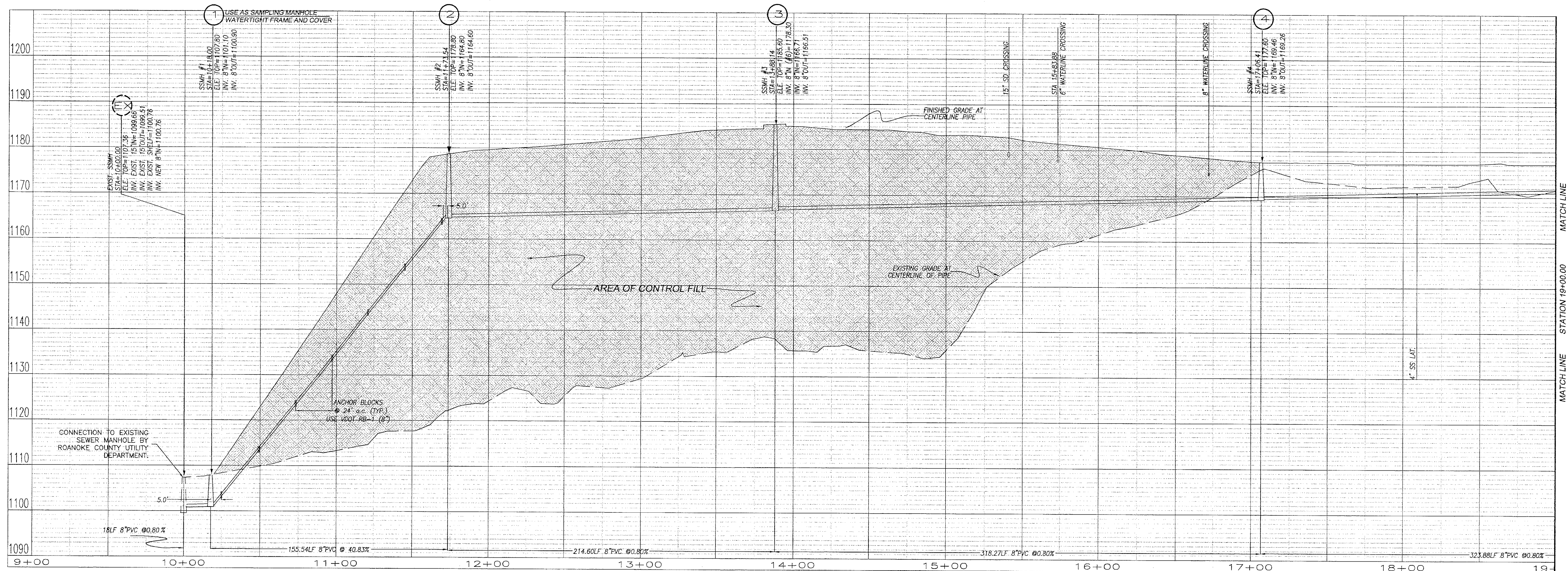
SANITARY SEWER PROFILES
