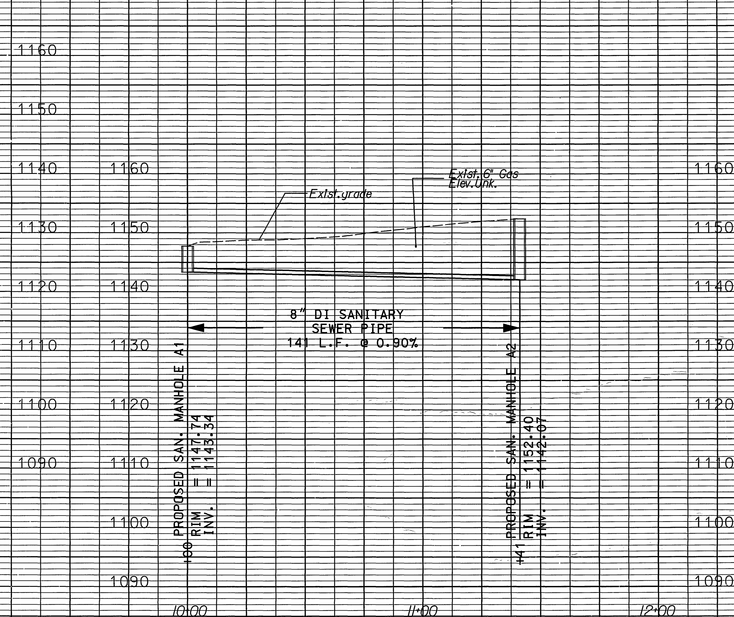
8" SANITARY SEWER PIPE, PLAN SHEET 10(7) APPROX. STA. 37+47, 71' RT. CONST. ON COLONIAL AVENUE TO APPROX. STA. 38+87, 87' RT. CONST. ON COLONIAL AVENUE
