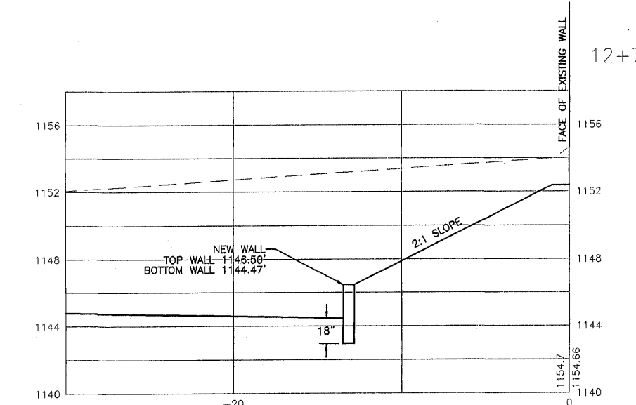
SECTIONS - WALL "D" SCALE: H: 1" = 4' V: 1" = 4'
