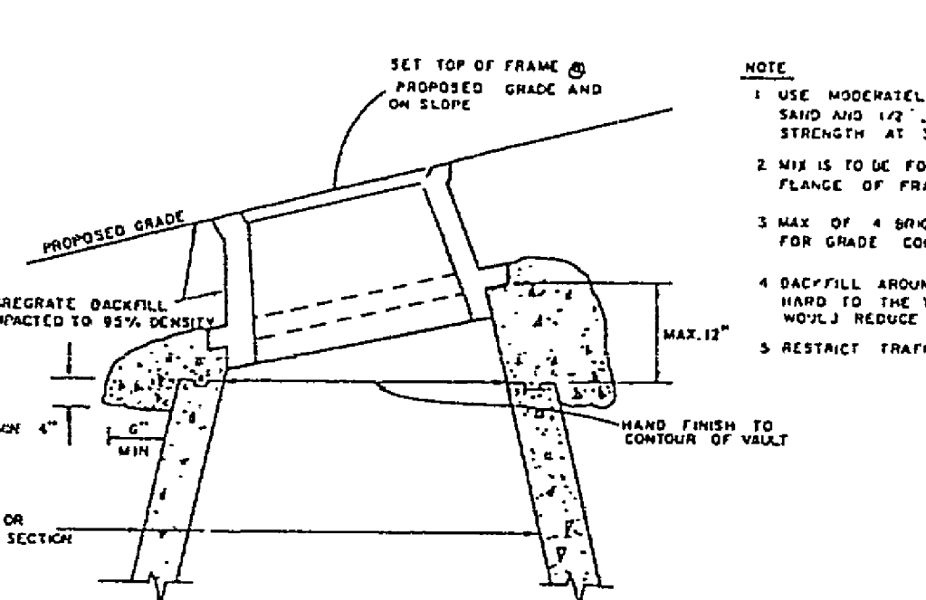
MANHOLE FRAME & COVER ADJUSTMENT
