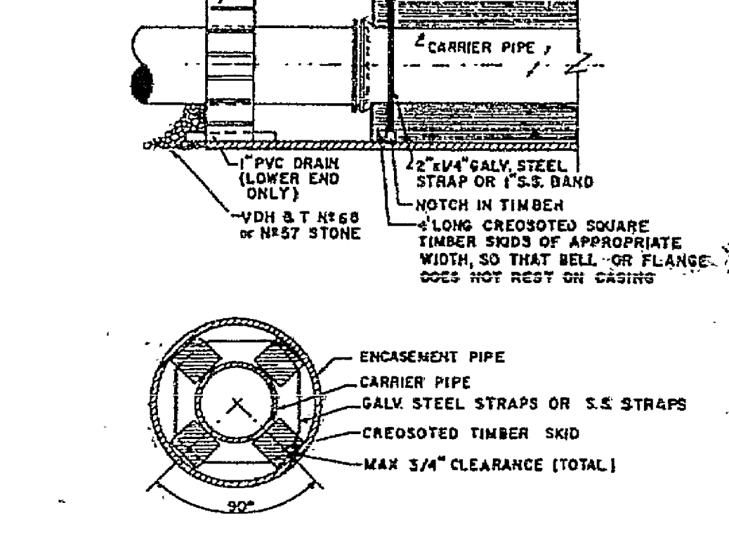
PIPE SUPPORT IN CASING PIPE
