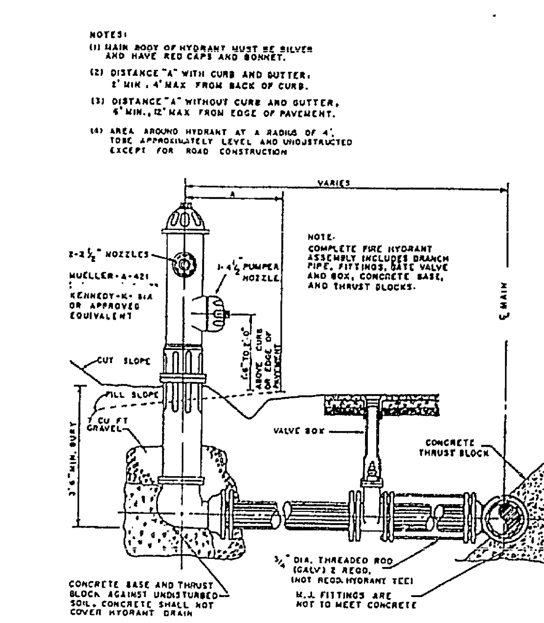
FIRE HYDRANT SETTING
