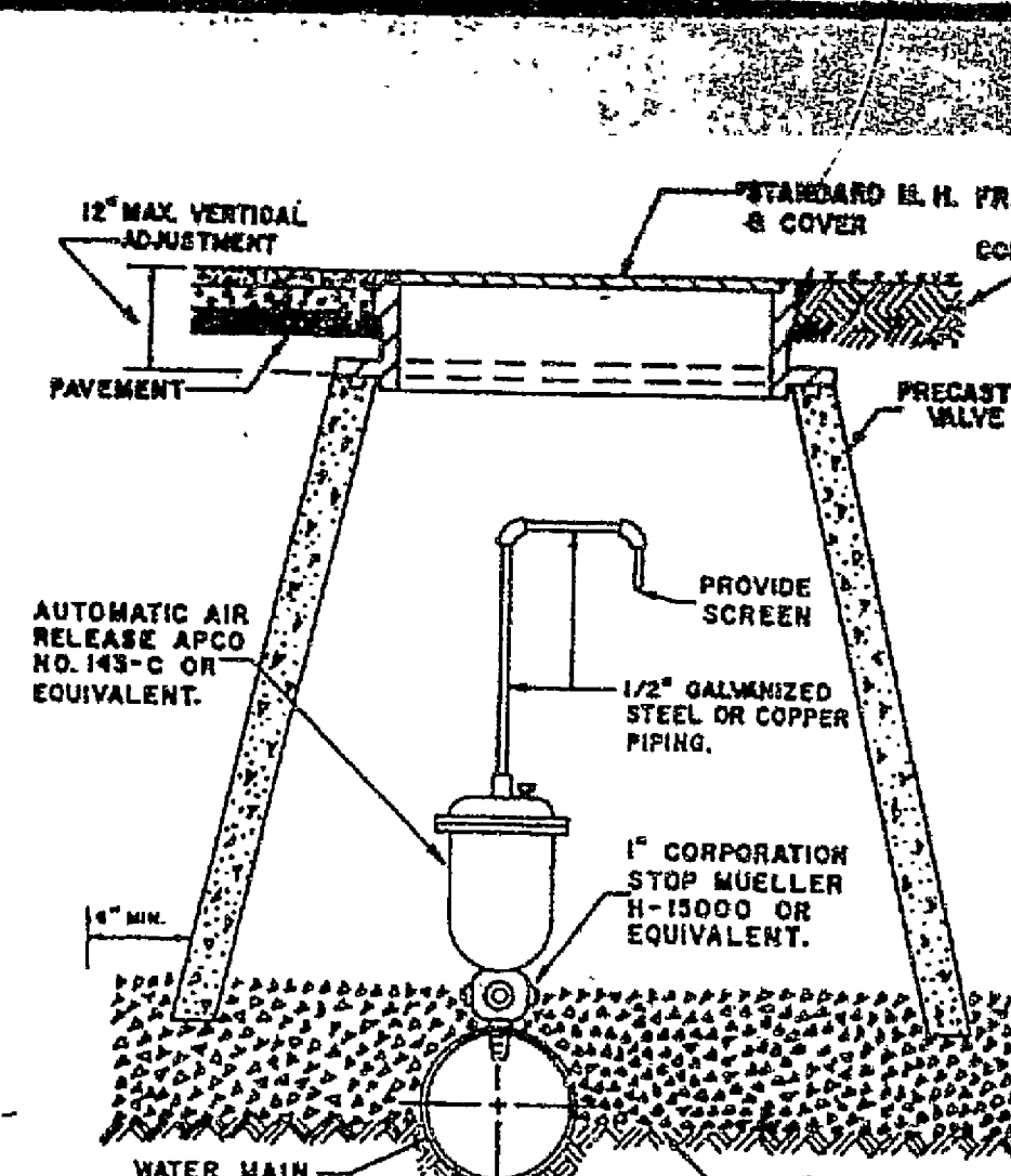
AUTOMATIC AIR RELEASE ASSEMBLY
