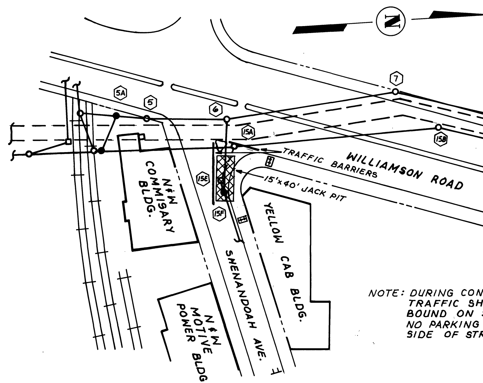
TRAFFIC CONTROL SCALE: 1" = 50'
