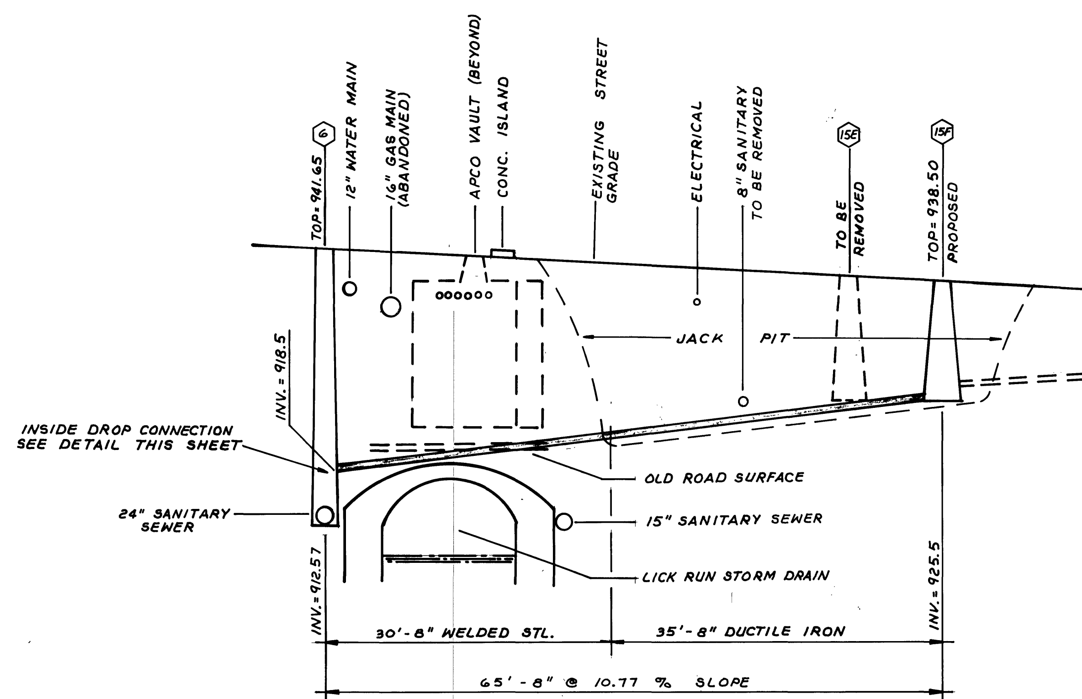
CROSS-SECTION SCALE: 1" = 10'
