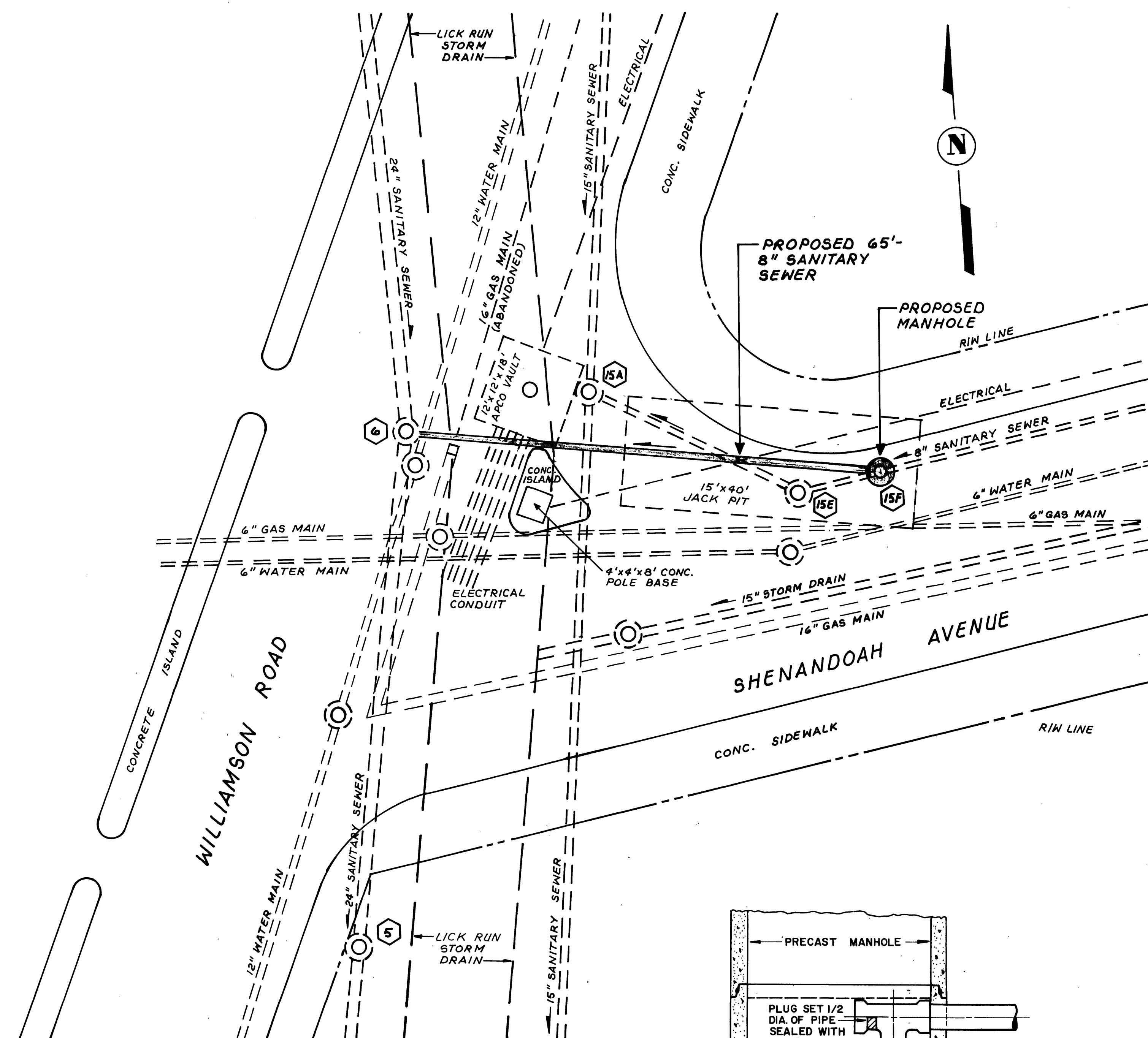
LOCATION OF UTILITIES SCALE: 1" = 10'
