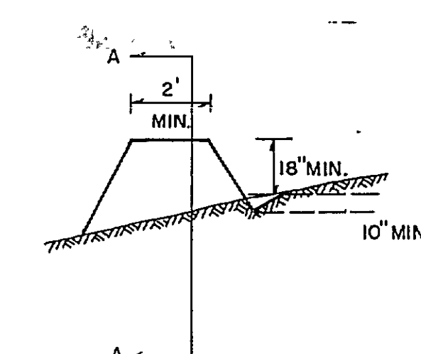
EARTH BERM & GRAVEL FILTER
