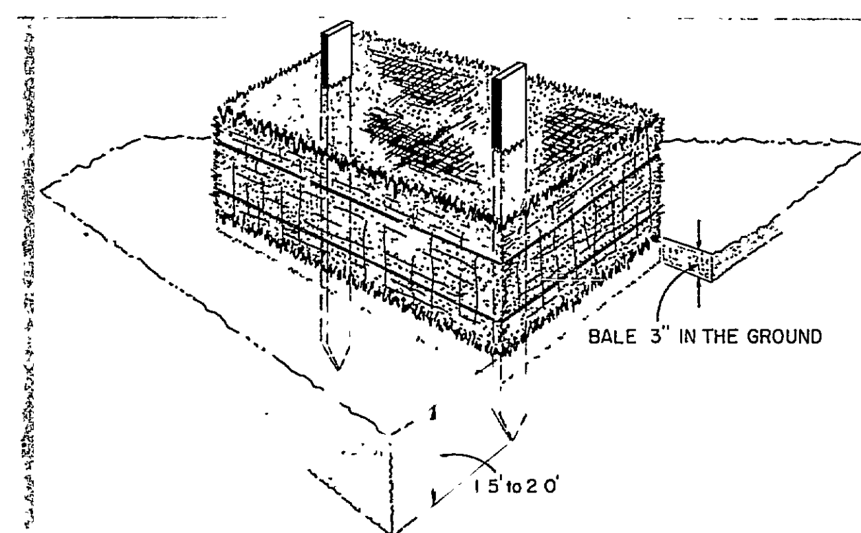
TEMPORARY STRAW BALE SEDIMENT BARRIER
