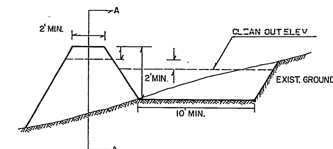
EARTH BERM WITH SILT BASIN & GRAVEL FILTER
