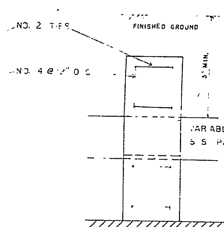
ANCHOR DETAIL
