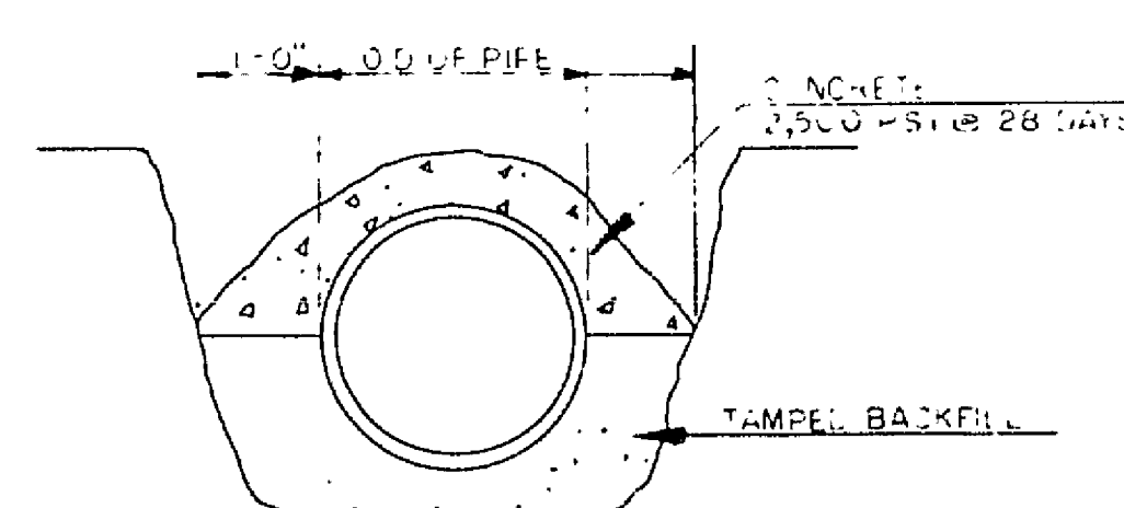
CONCRETE CAP
