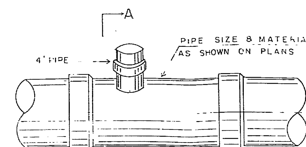
SERVICE CONNECTION "T"
