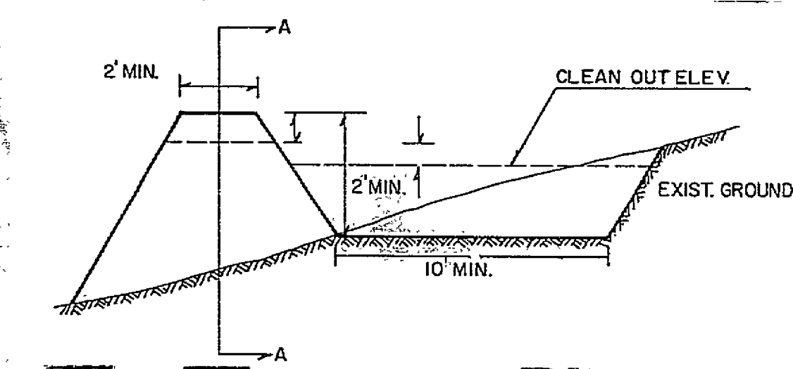
EARTH BERM WITH SILT BASIN & GRAVEL FILTER
