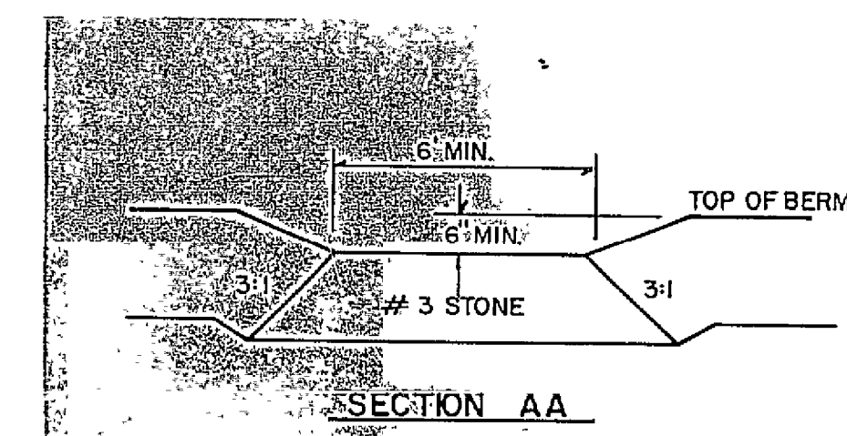
EARTH BERM WITH SILT BASIN & GRAVEL FILTER
