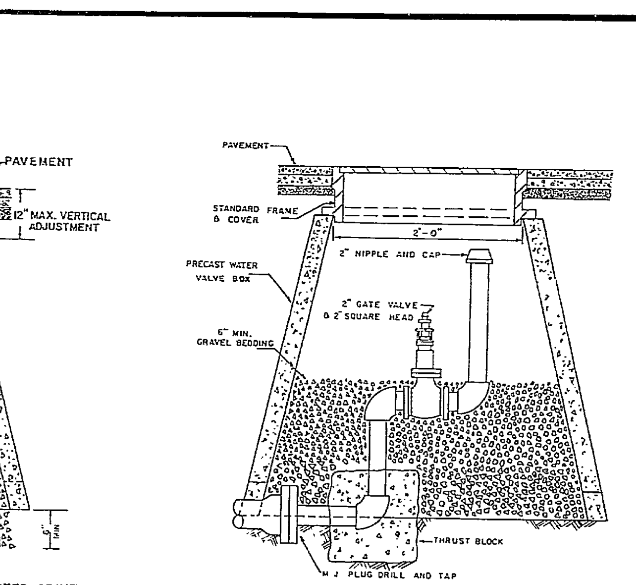
PERMANENT END OF LINE
