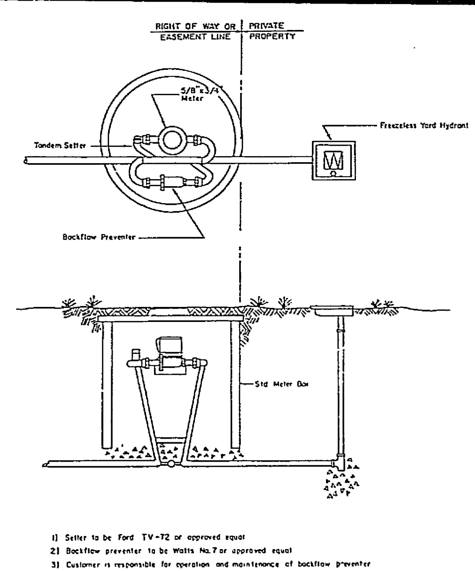
TYPICAL SPRINKLER SERVICE
