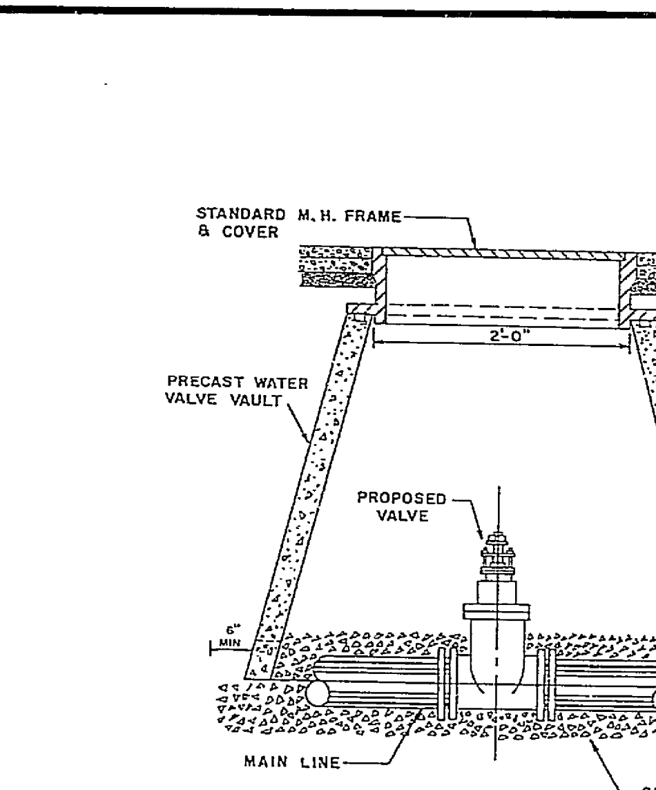
WATER LINE VALVE INSTALLATION
