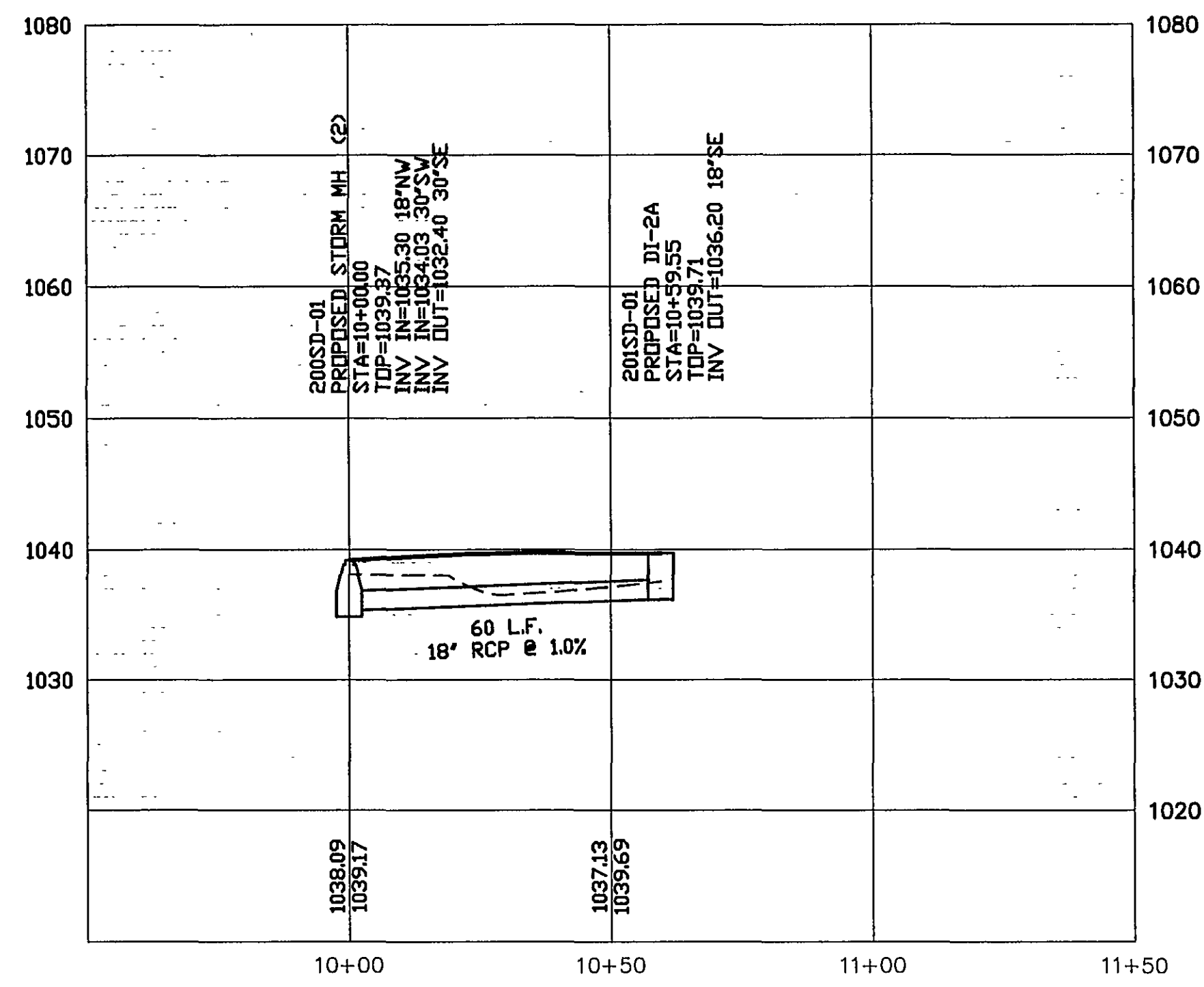
STORM SEWER LINE 201 SCALE = 1"=25'H, 1"=10'V
