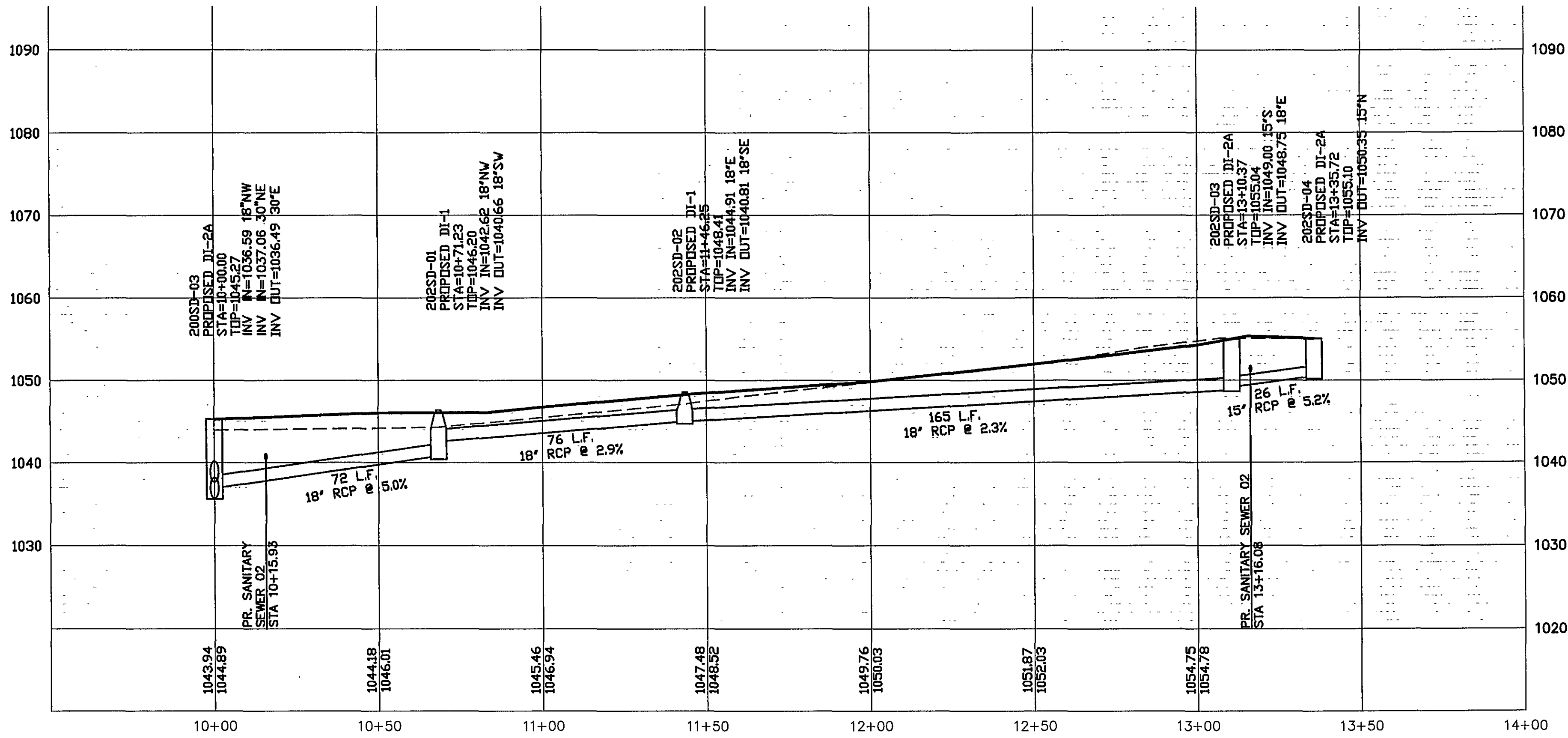
STORM SEWER LINE 202 SCALE = 1"=25'H, 1"=10'V
