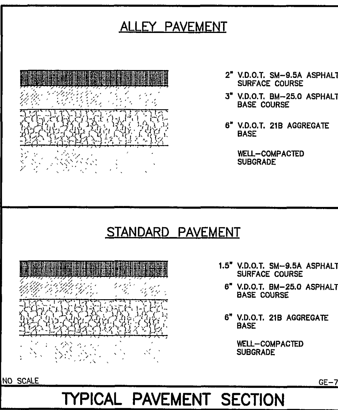
NO SCALE GE-70 TYPICAL PAVEMENT SECTION
