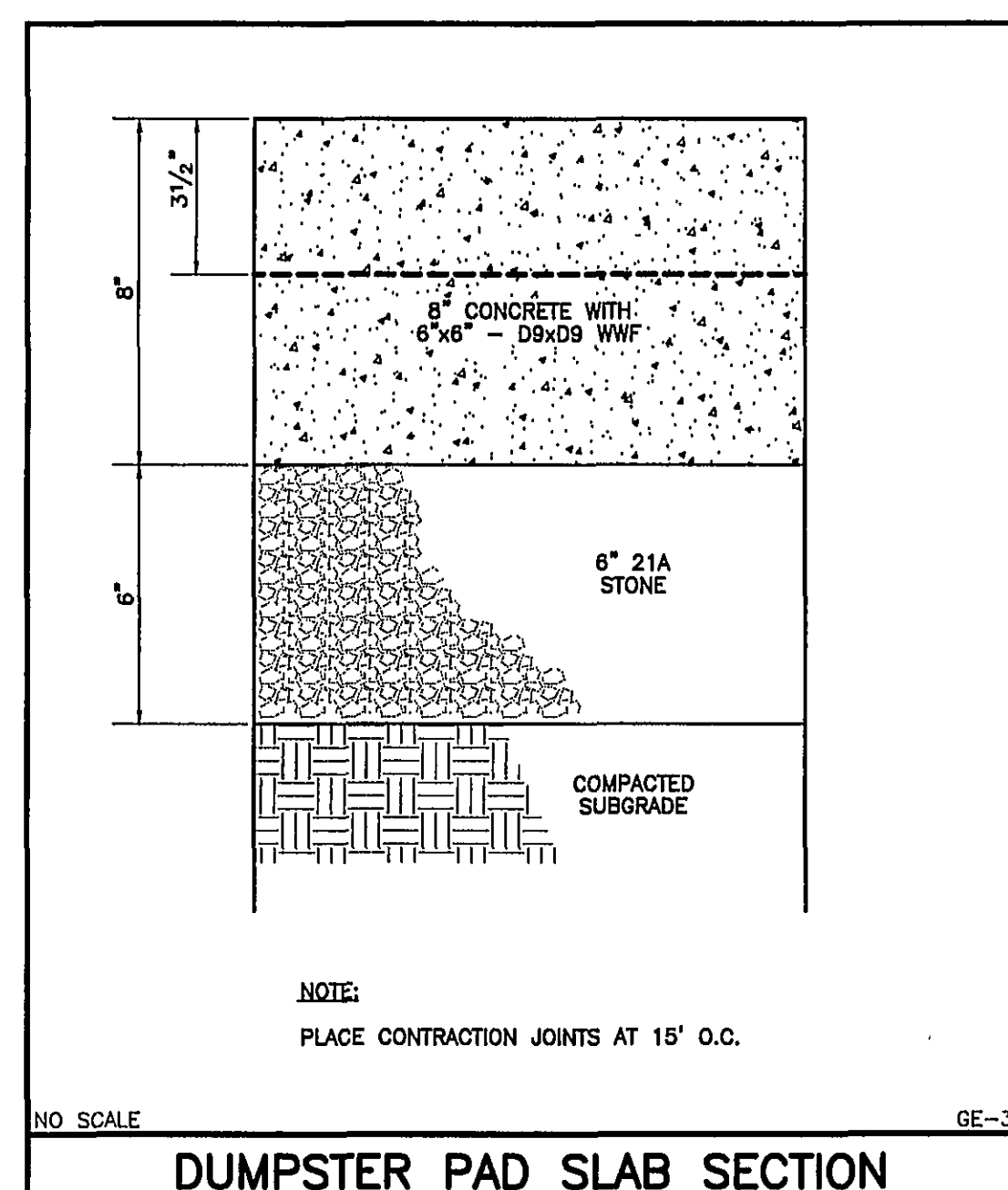
NO SCALE GE-35 DUMPSTER PAD SLAB SECTION
