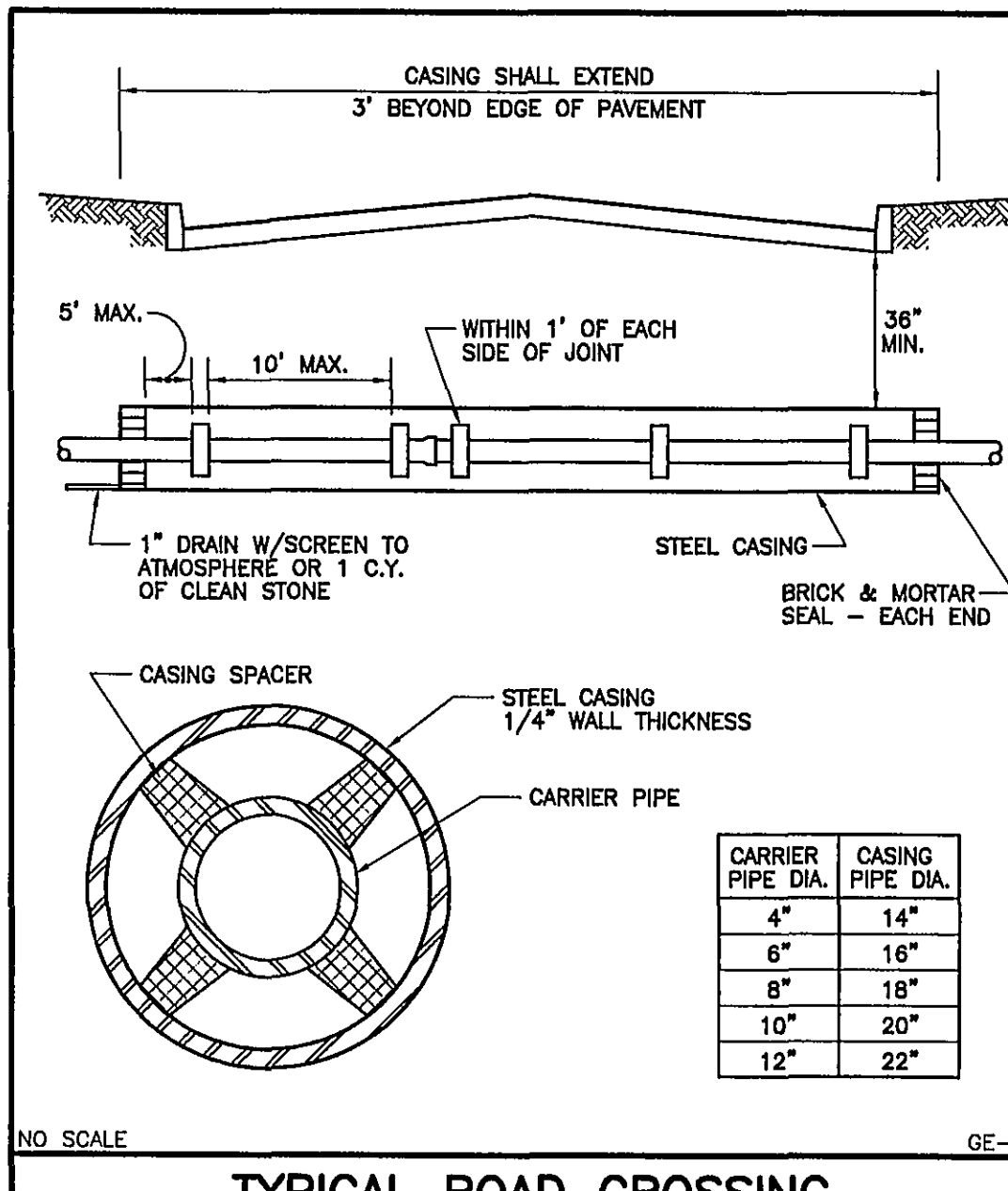
NO SCALE GE-15 TYPICAL ROAD CROSSING
