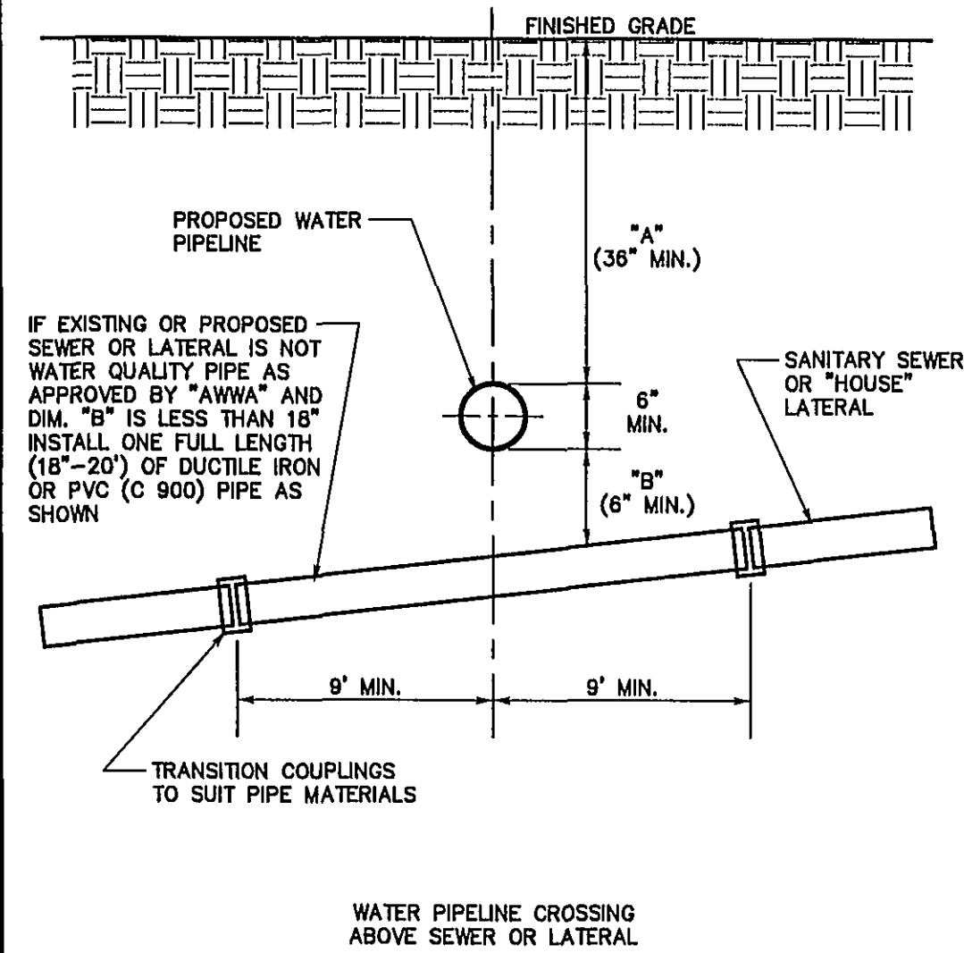
NO SCALE GE-51 WATERLINE CROSSING SANITARY SEWER
