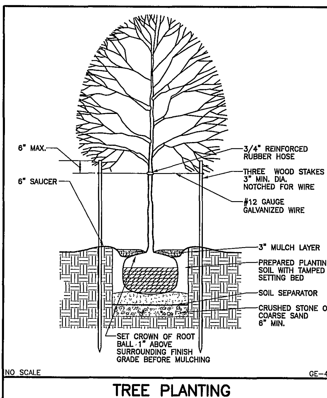
NO SCALE GE-41A TREE PLANTING
