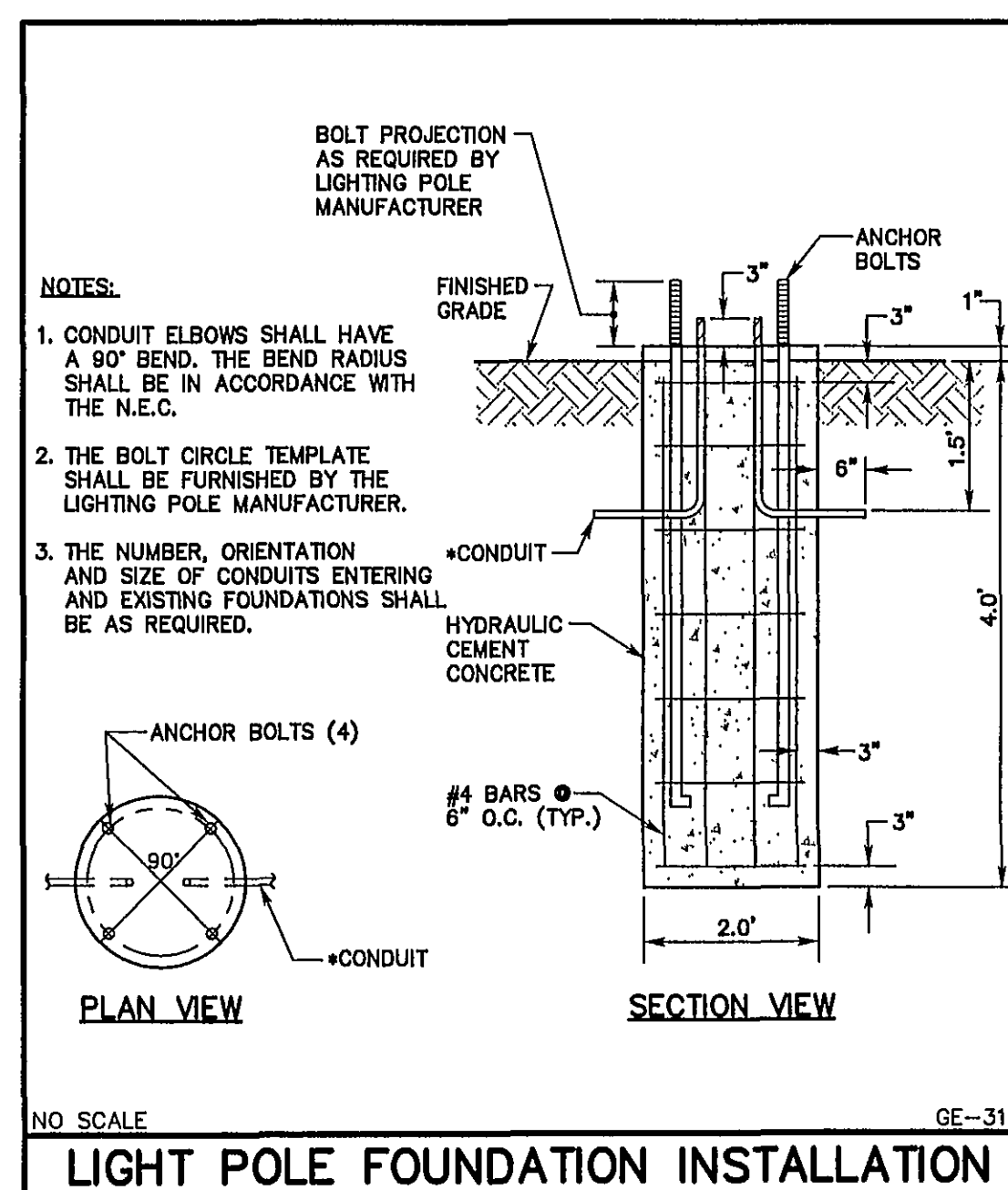
NO SCALE GE-31A LIGHT POLE FOUNDATION INSTALLATION
