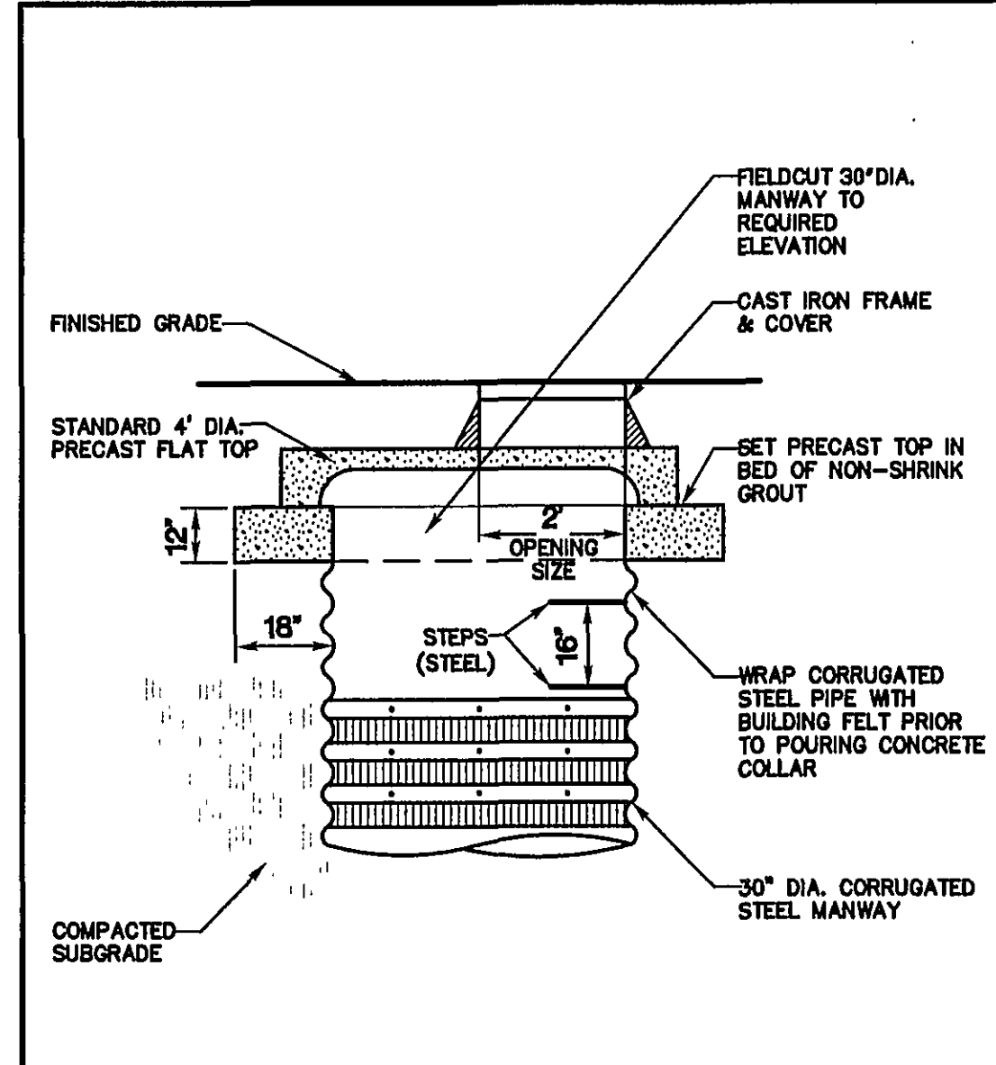
NO SCALE GE-78 UNDERGROUND DETENTION ACCESS DETAIL
