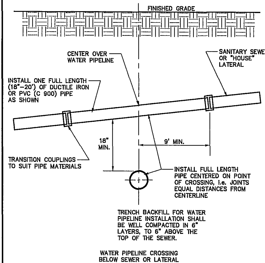
NO SCALE GE-52 SANITARY SEWER CROSSING WATERLINE
