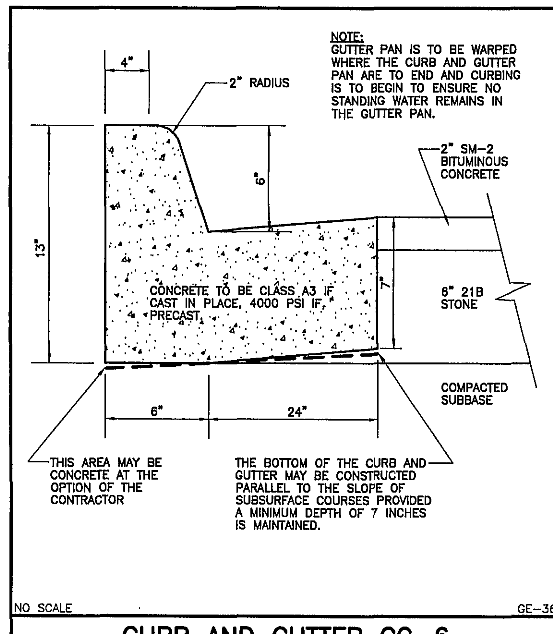
NO SCALE GE-36 CURB AND GUTTER CG-6
