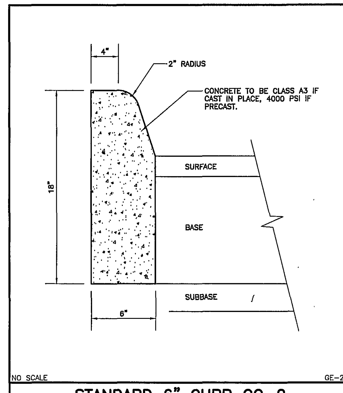
NO SCALE GE-28 STANDARD 6" CURB CG-2
