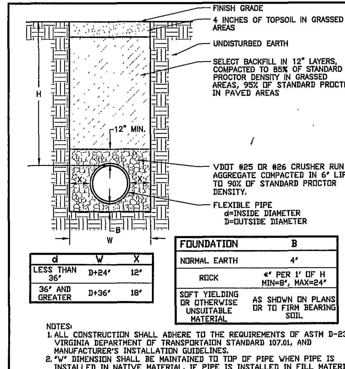
NO SCALE GE-72 STORM SEWER TRENCH (FLEXIBLE PIPE)
