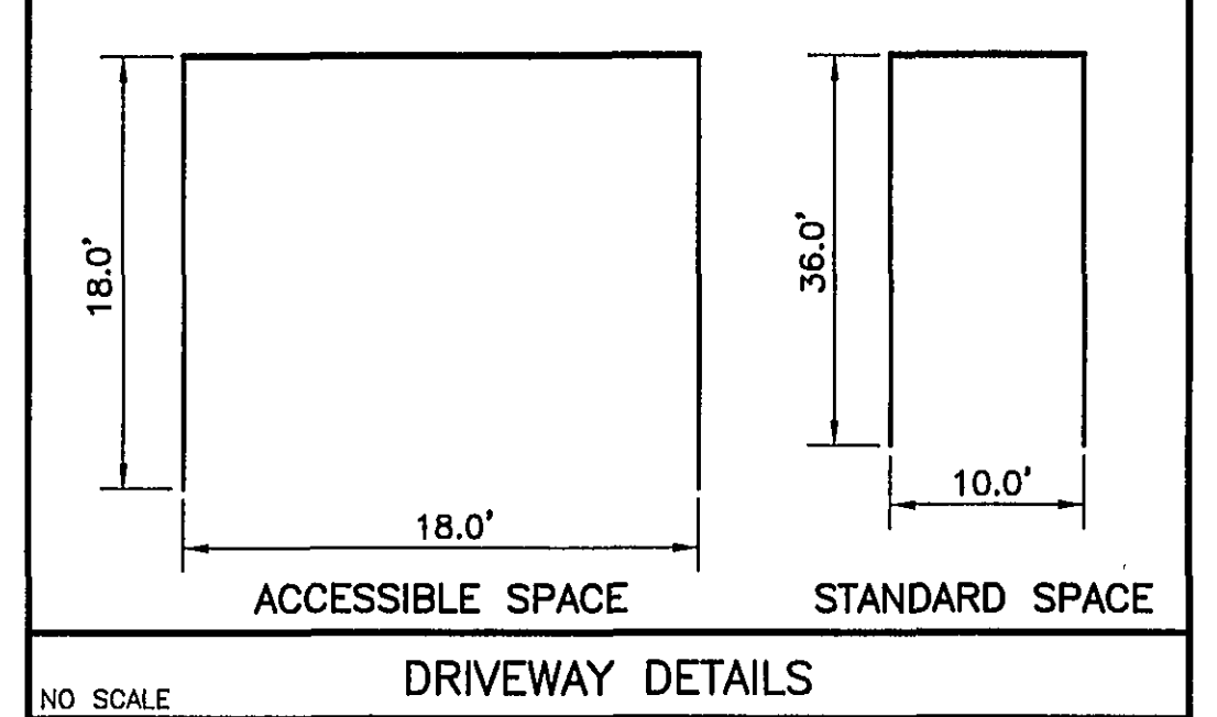
NO SCALE DRIVEWAY DETAILS
