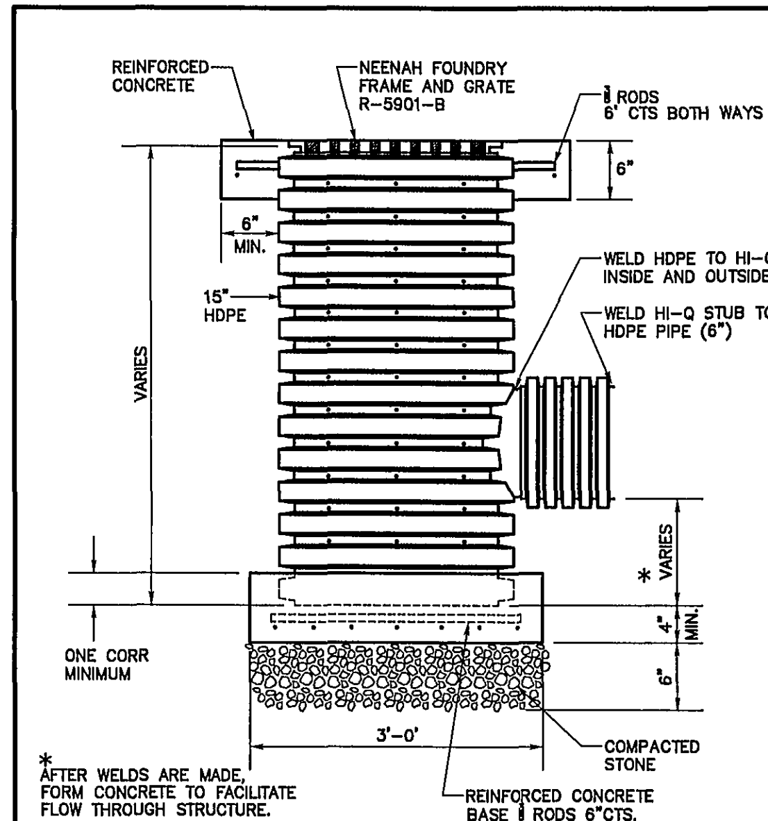
NO SCALE GE-50 TYPICAL YARD DRAIN SECTION
