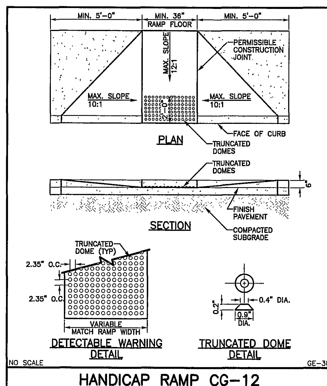
NO SCALE GE-30 HANDICAP RAMP CG-12
