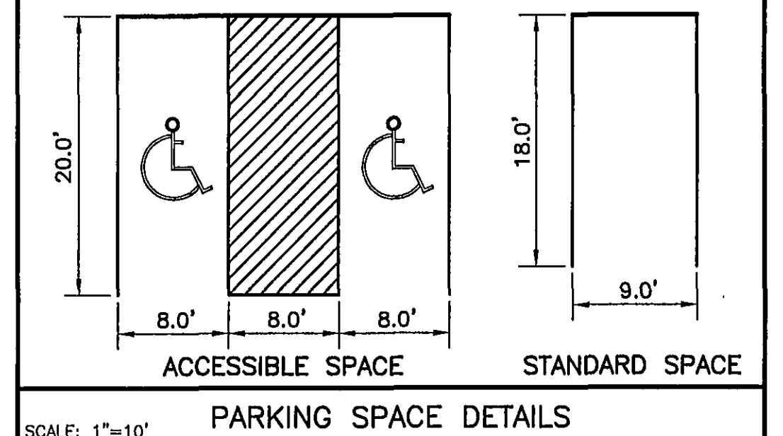
NO SCALE PARKING SPACE DETAILS
