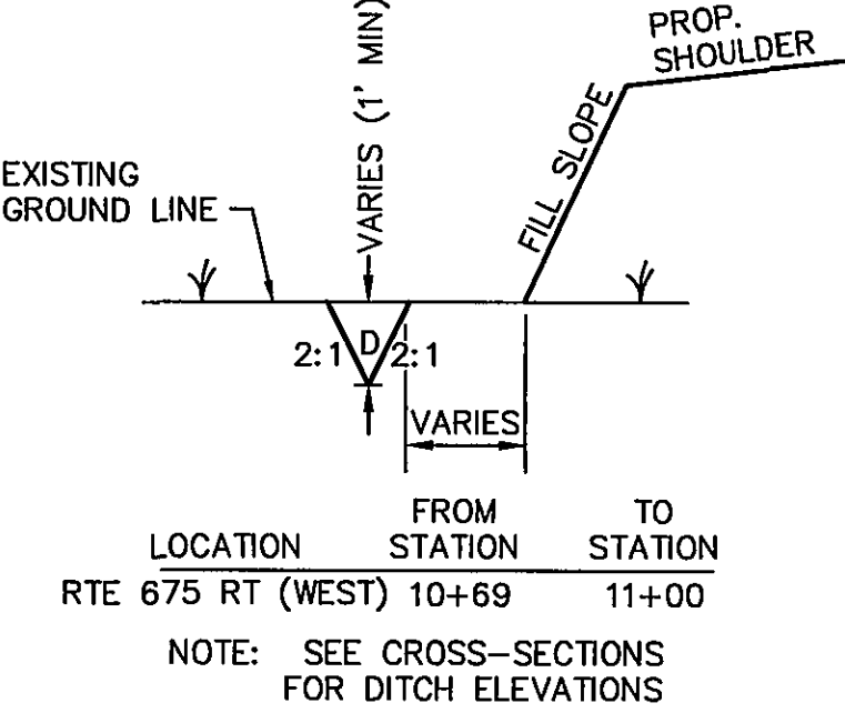
PROPOSED TOE DITCH
