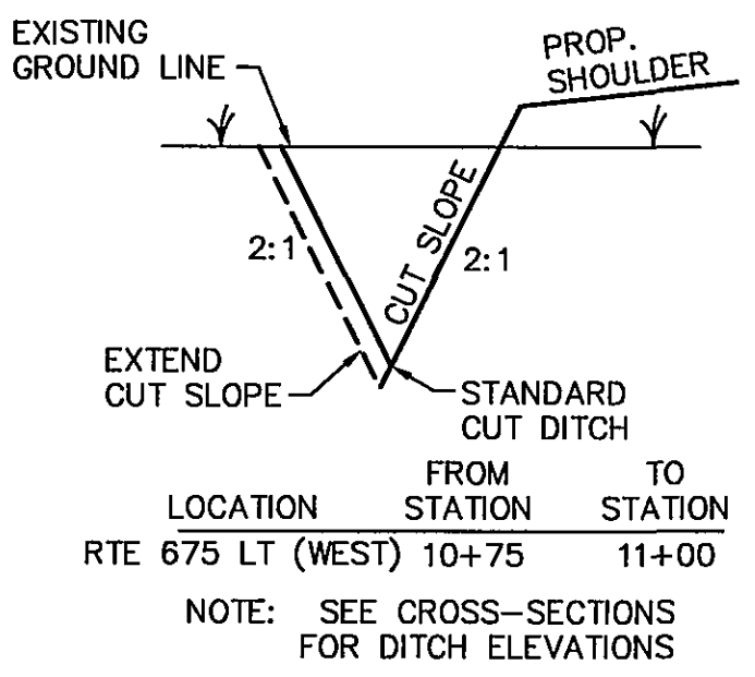
PROPOSED TOE DITCH
