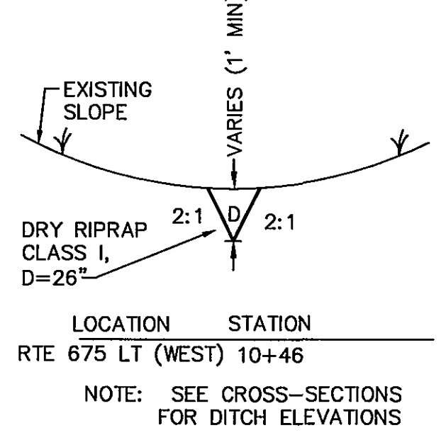
PROPOSED DITCH
