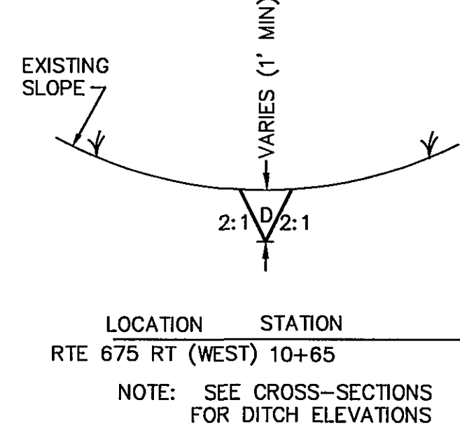
PROPOSED DITCH
