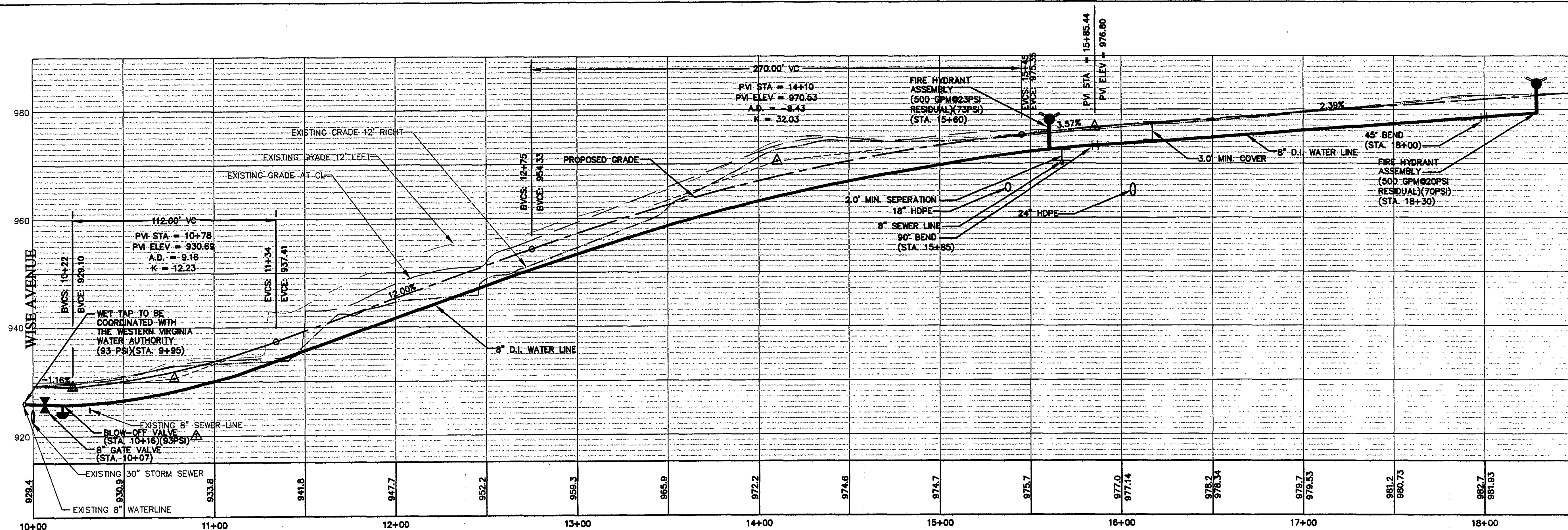
Δ DRIVEWAY AND WATERLINE PROFILE HORIZ. SCALE: 1" = 30' VERT. SCALE: 1" = 10'
