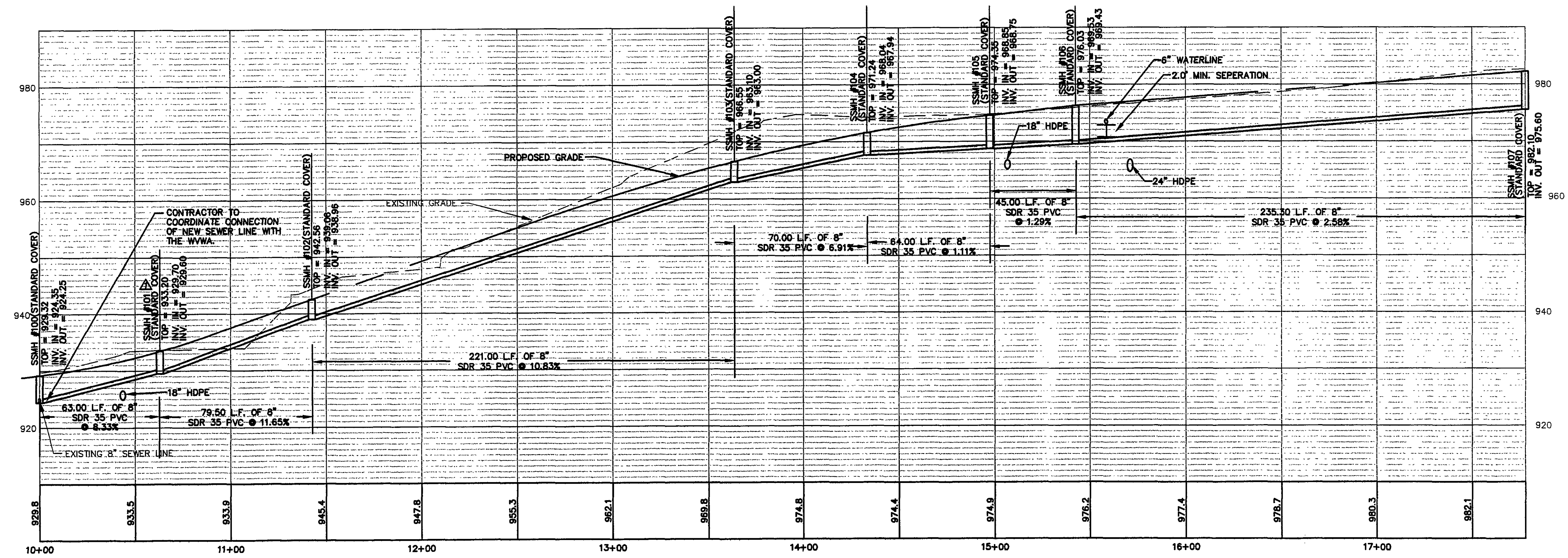
SANITARY SEWER PROFILE HORIZ. SCALE: 1" = 30' VERT. SCALE: 1" = 10'
