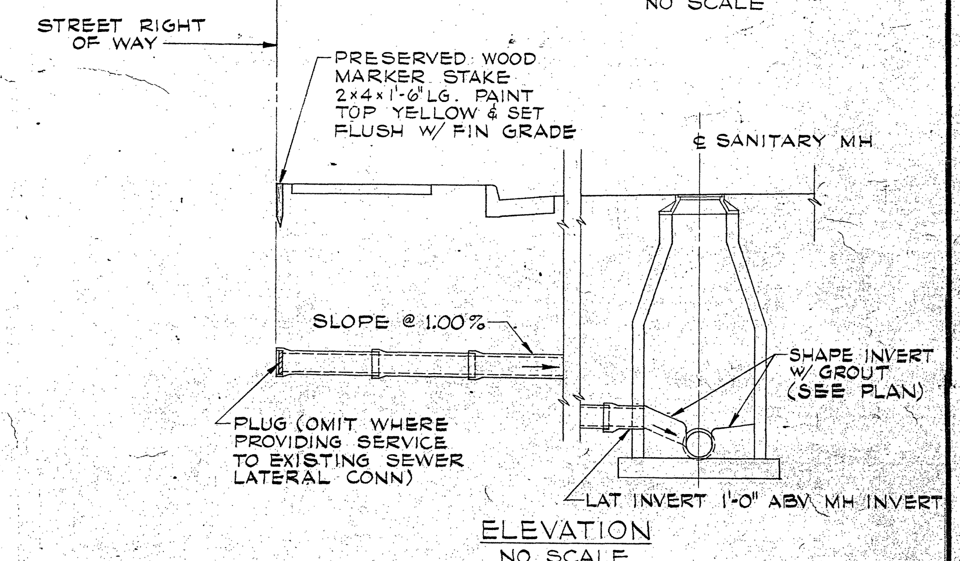
SANITARY SEWER LATERAL CONNECTIONS
