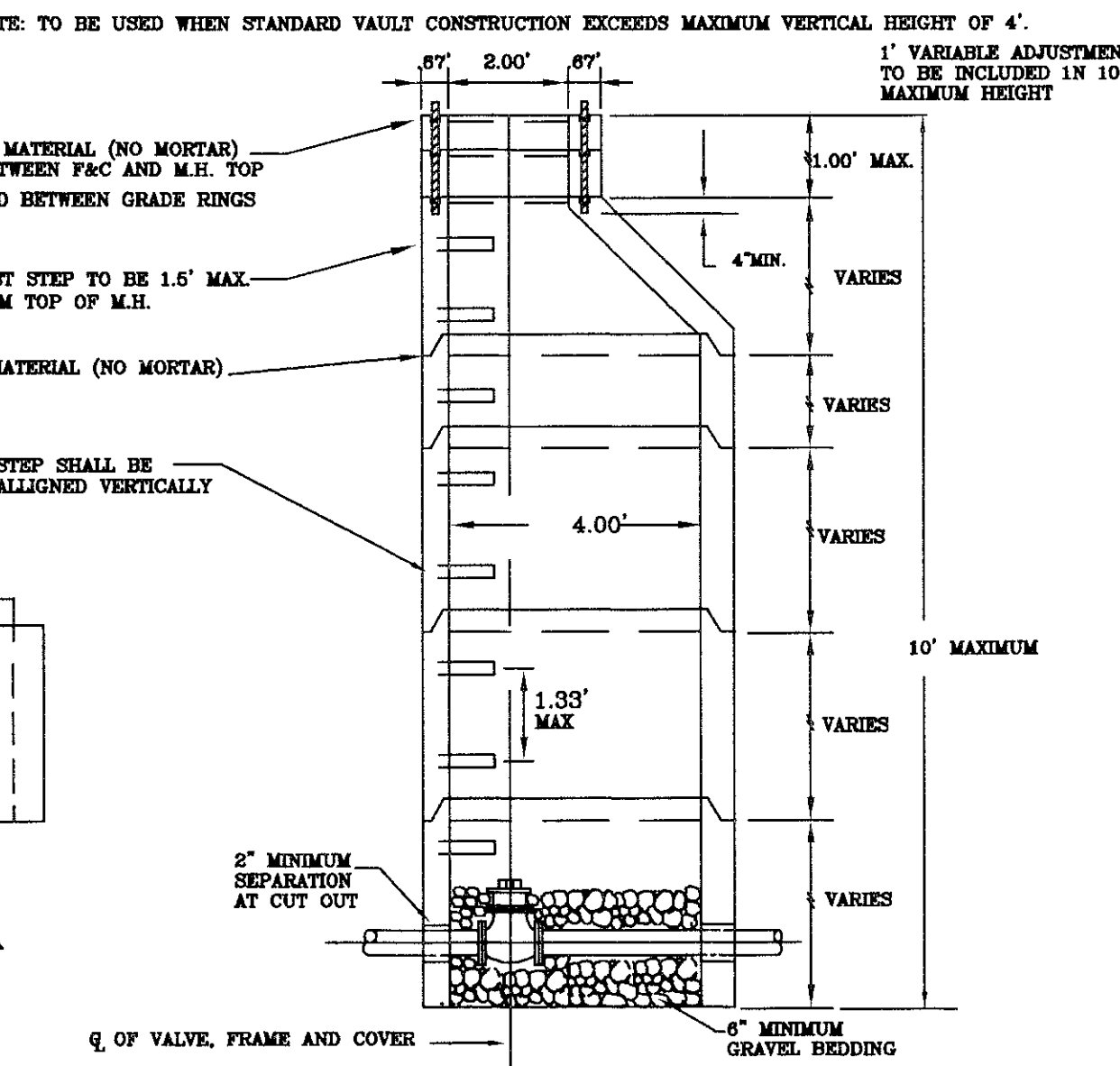
ALTERNATE VALVE VAULT (MANHOLE)
