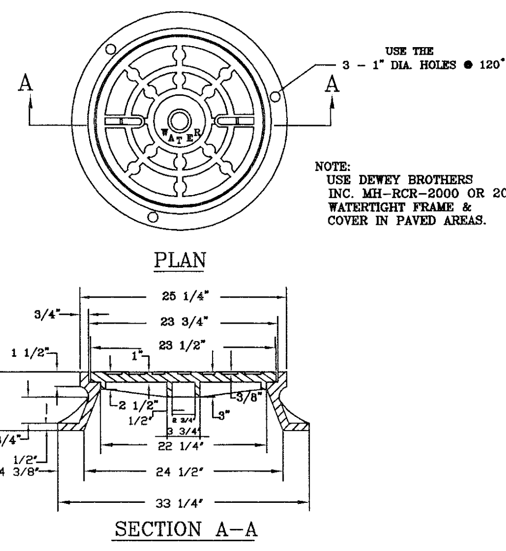
MANHOLE FRAME AND COVER PAVED 2001EC UNPAVED 2001(ABOVE)
