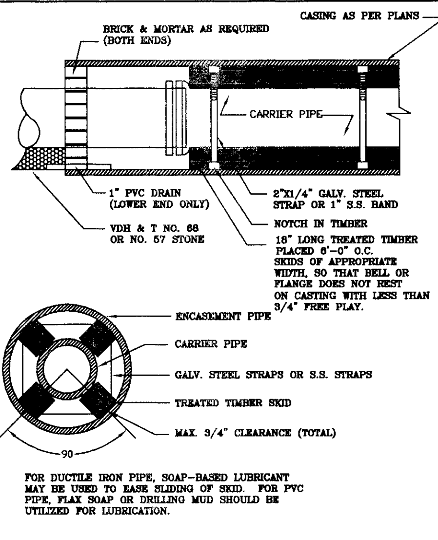
PIPE SUPPORT IN CASING PIPE
