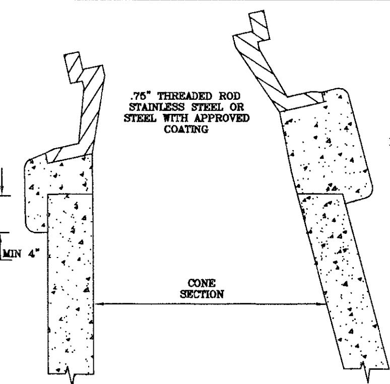
INSTALLATION DETAIL FOR ALL FRAMES AND COVERS
