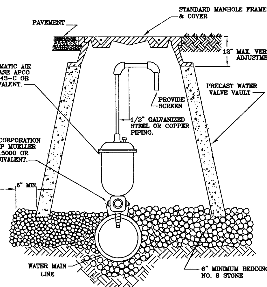
AUTOMATIC AIR RELEASE ASSEMBLY
