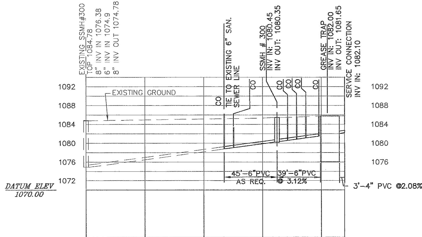
SD-200 PROFILE SCALE: 1" = 40' HORIZONTAL 1" = 10' VERTICAL
