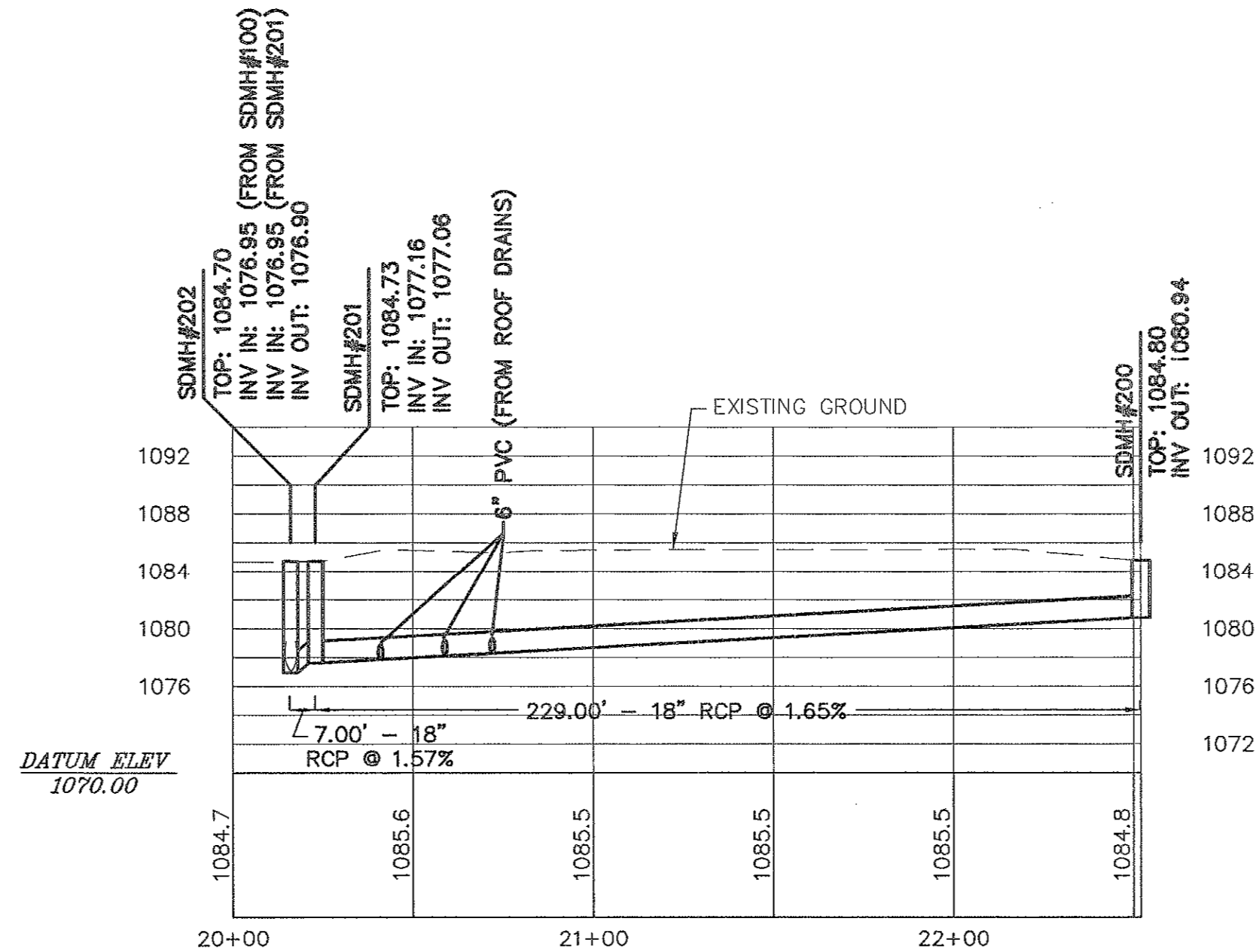
SD-200 PROFILE SCALE: 1" = 40' HORIZONTAL 1" = 10' VERTICAL
