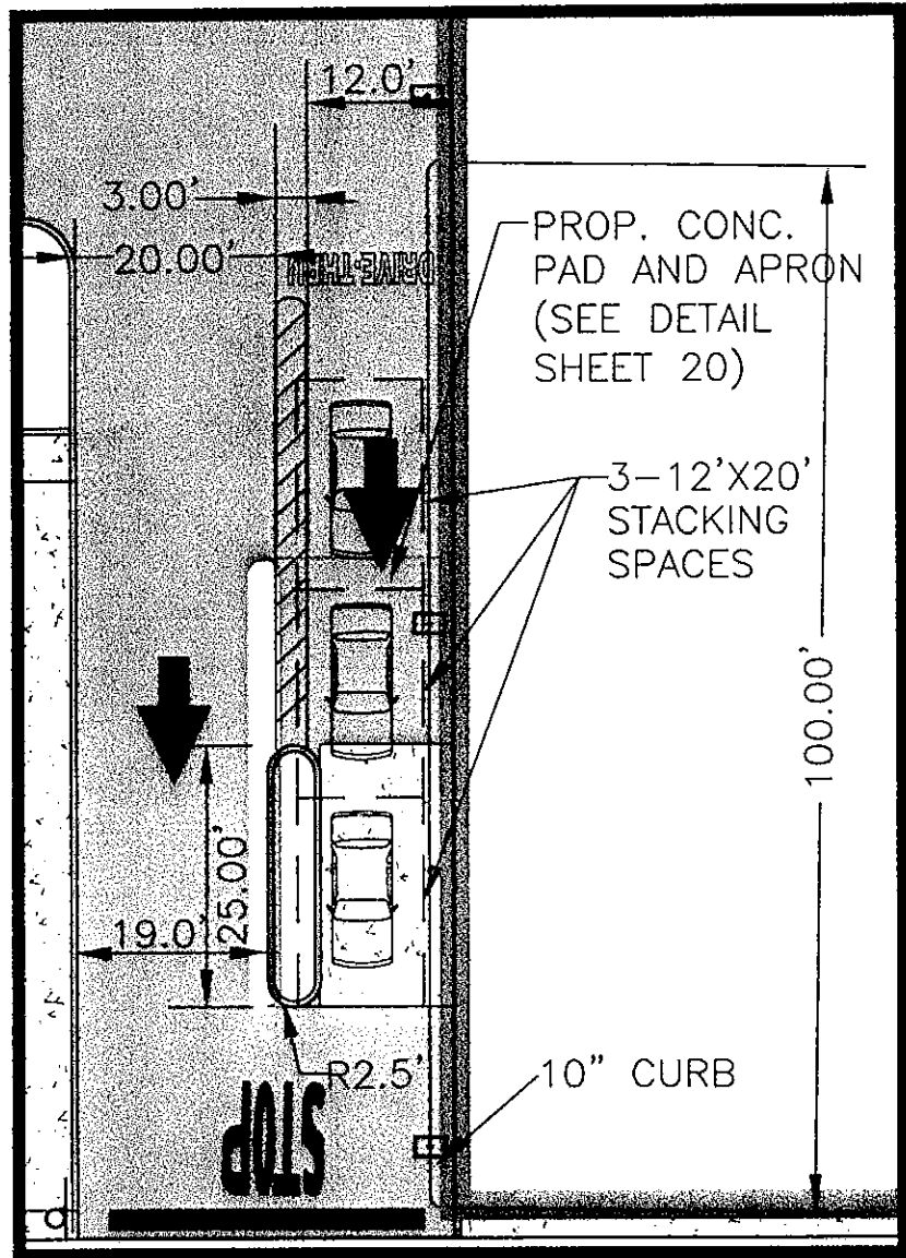
DRIVE-THRU DETAIL NOT IN CONTRACT SCALE 1"=20'
