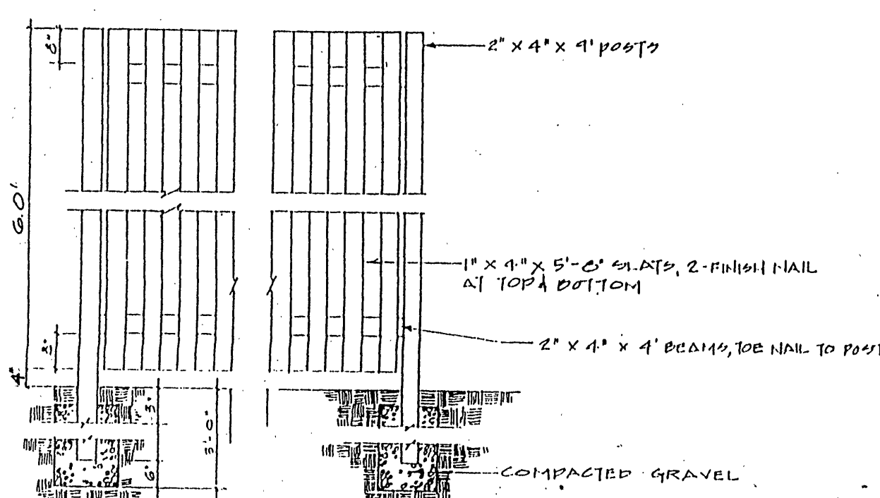
STOCKADE FENCE DETAIL NO SCALE
