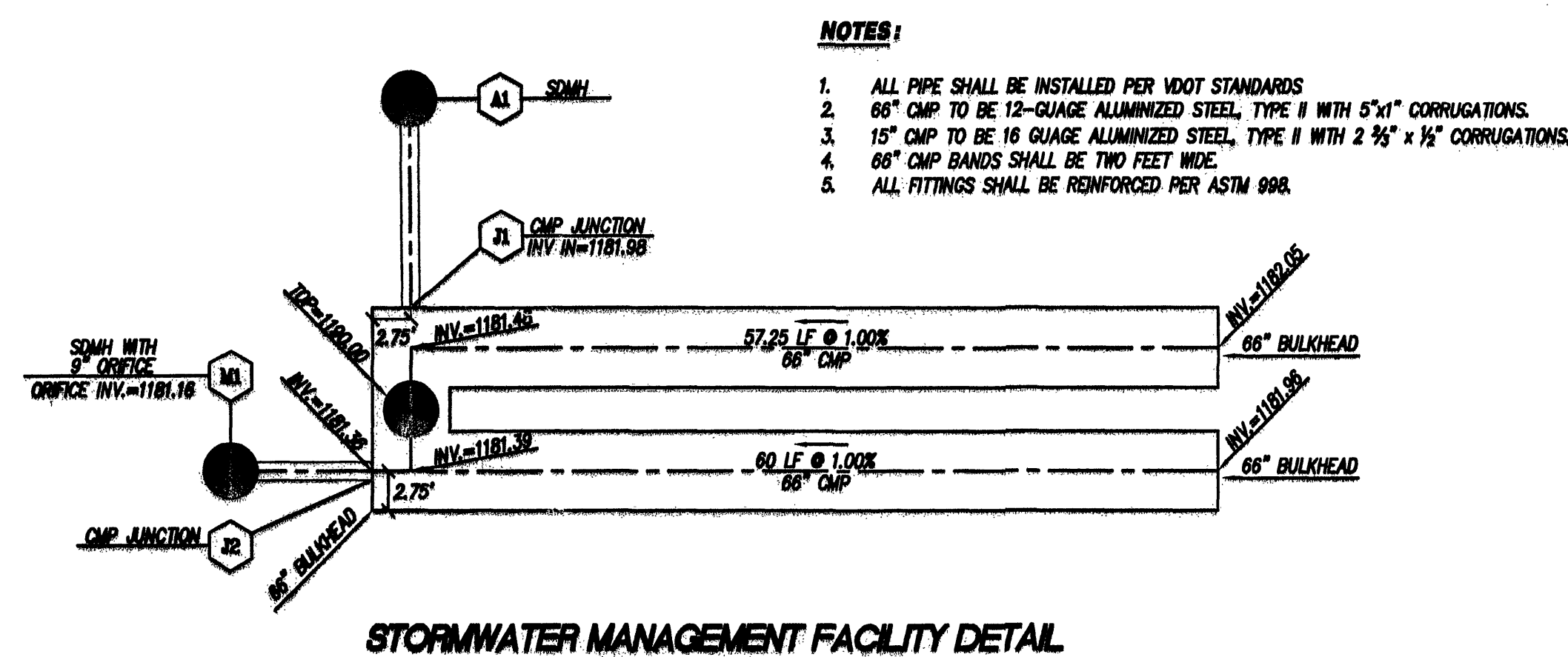
STORMWATER MANAGEMENT FACILITY DETAIL
