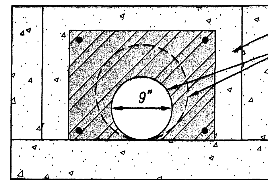
SDMH 'M1' WITH RESTRICTOR PLATE
