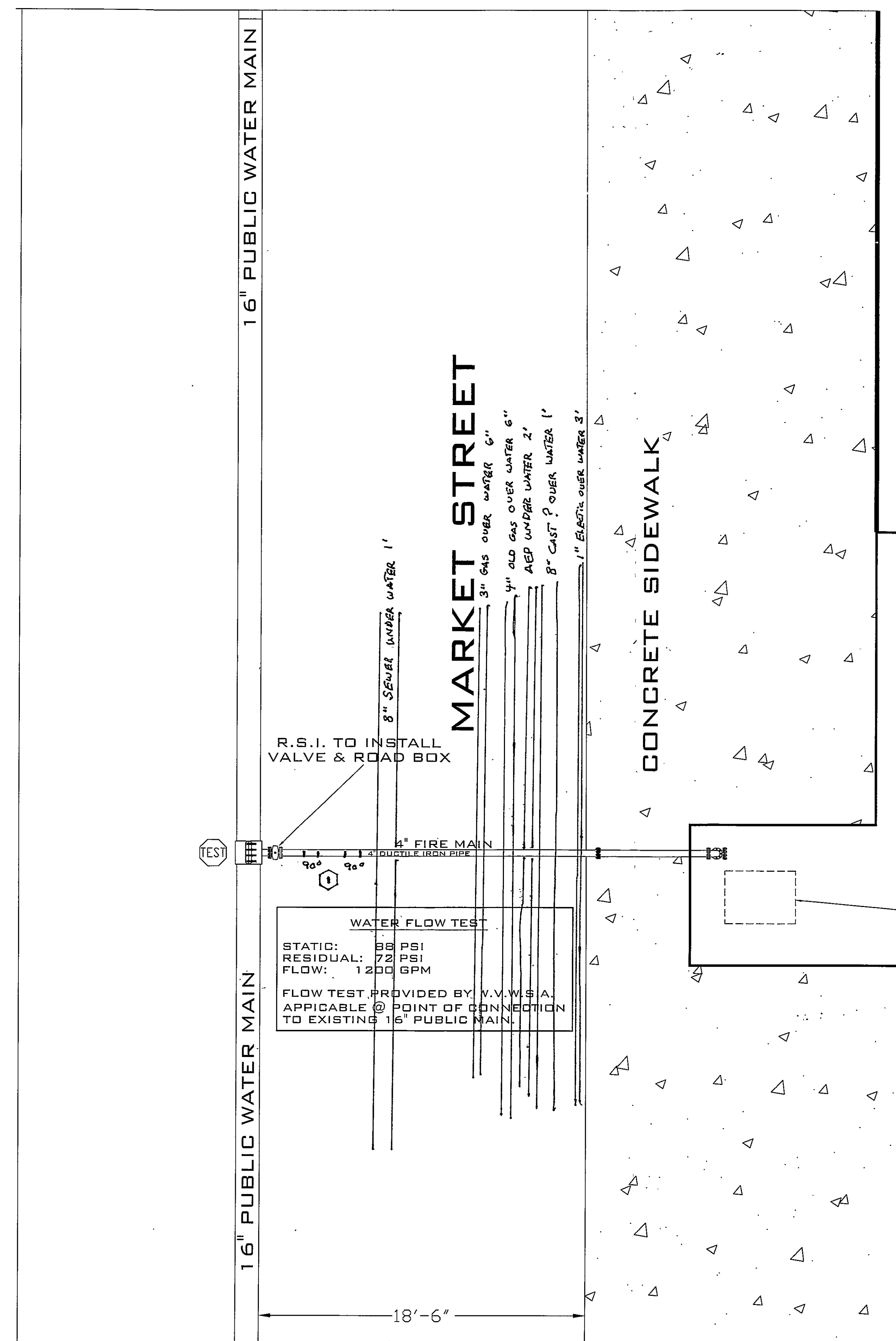
OVERALL UNDERGROUND PLAN 1/4" = 1'-0"
