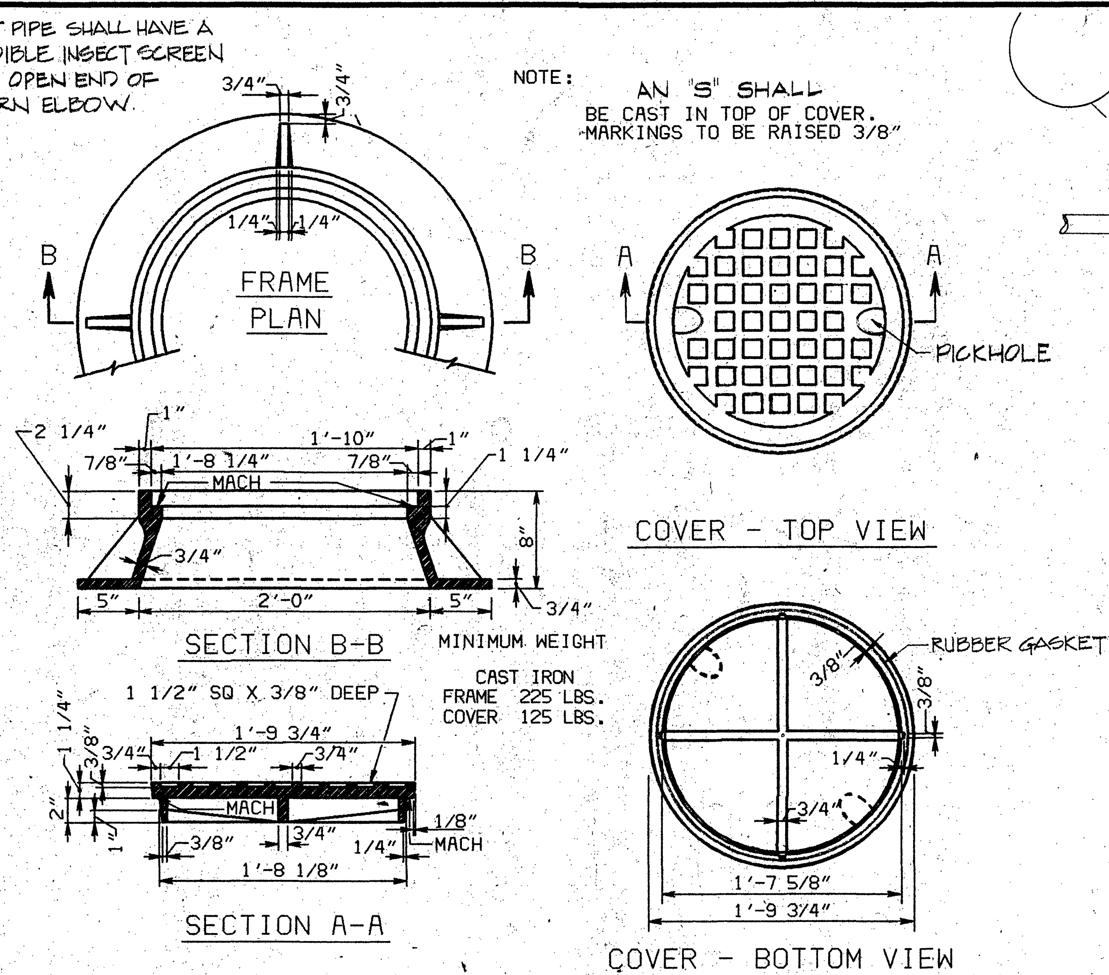
WATERTIGHT MANHOLE FRAME & COVER
