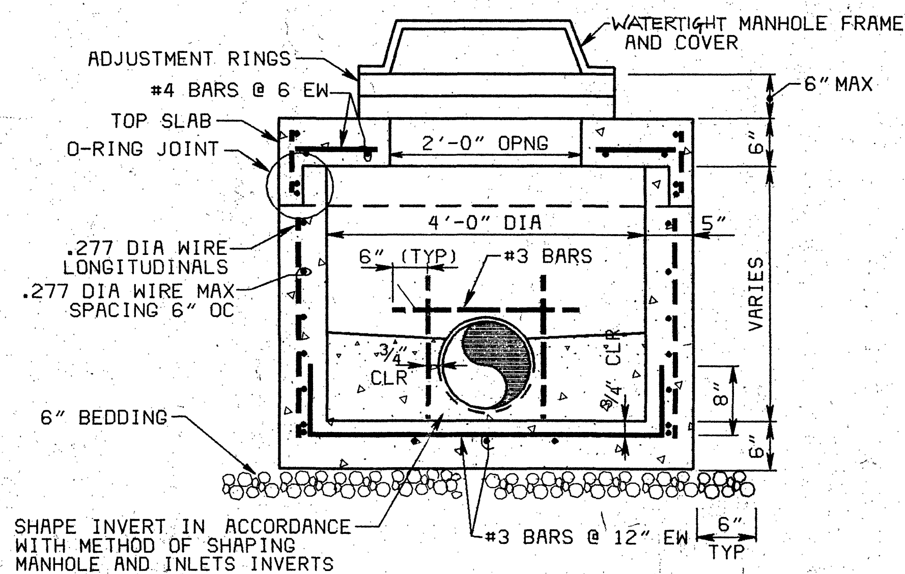
SECTION MANHOLE WITH STANDARD FRAME AND COVER
