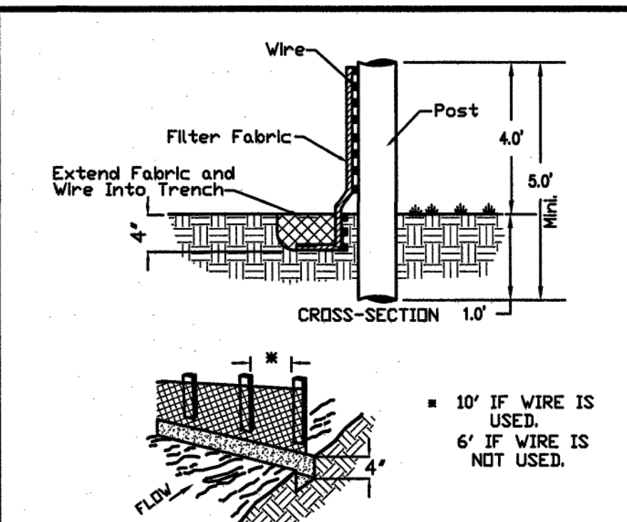
CONSTRUCTION OF A SILT FENCE
