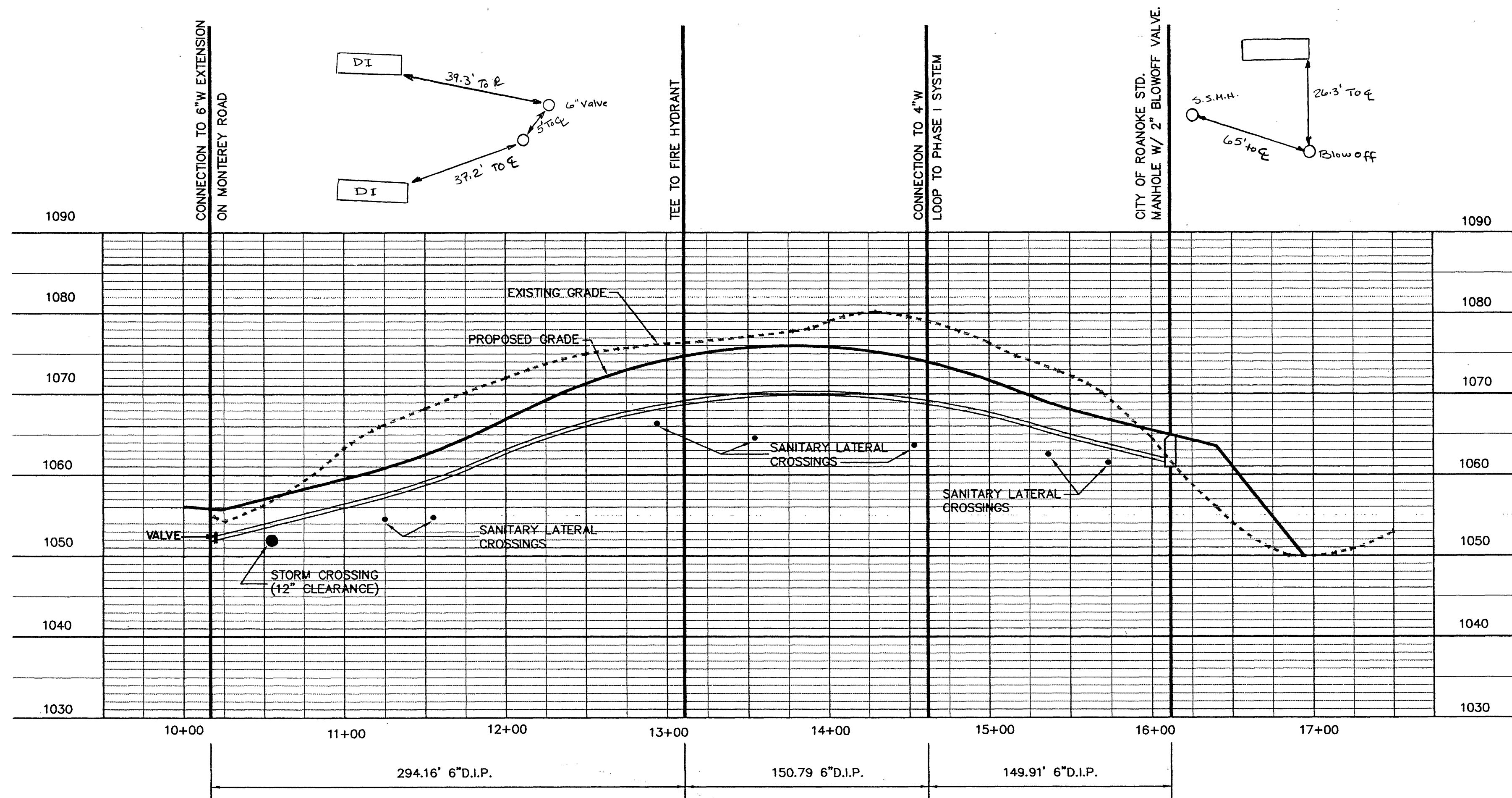
6" WATER MAIN PROFILE (JOHNSBURY COURT) SCALE: HORZ: 1" = 50' VERT: 1" = 10'
