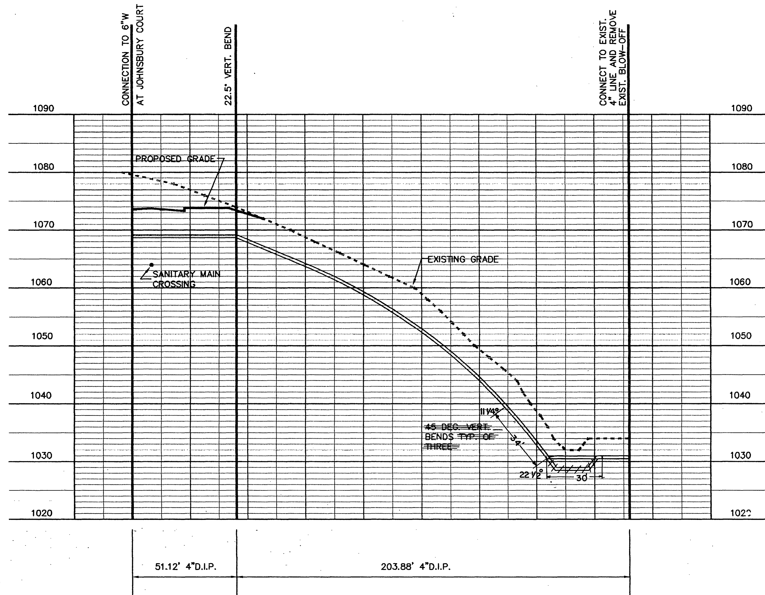
4" WATER MAIN PROFILE (LOOP TO EXIST.) SCALE: HORZ: 1" = 30' VERT: 1" = 10'
