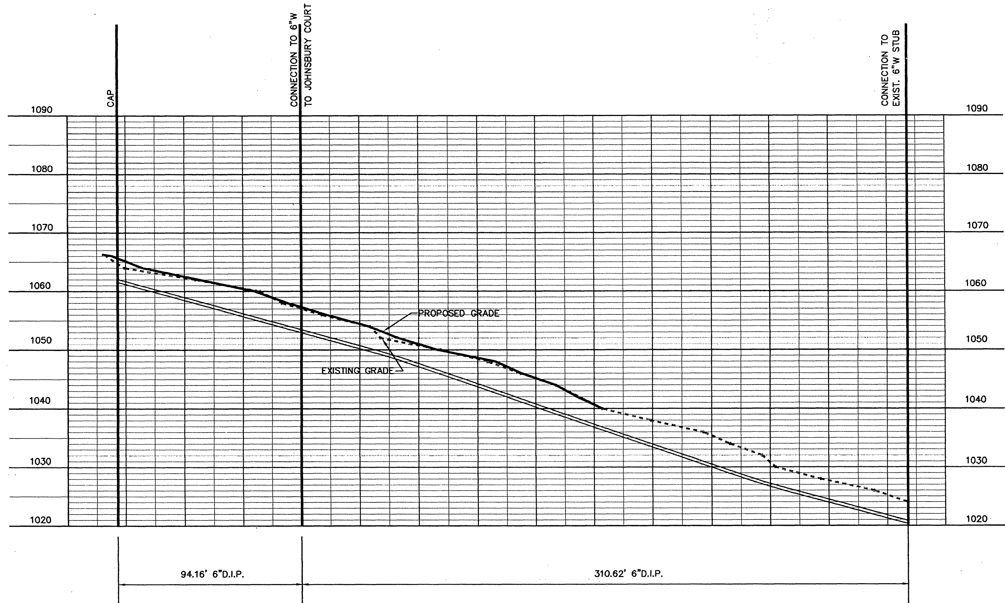
6" WATER EXTENSION PROFILE (MONTEREY ROAD) SCALE: HORZ: 1" = 30' VERT: 1" = 10'
