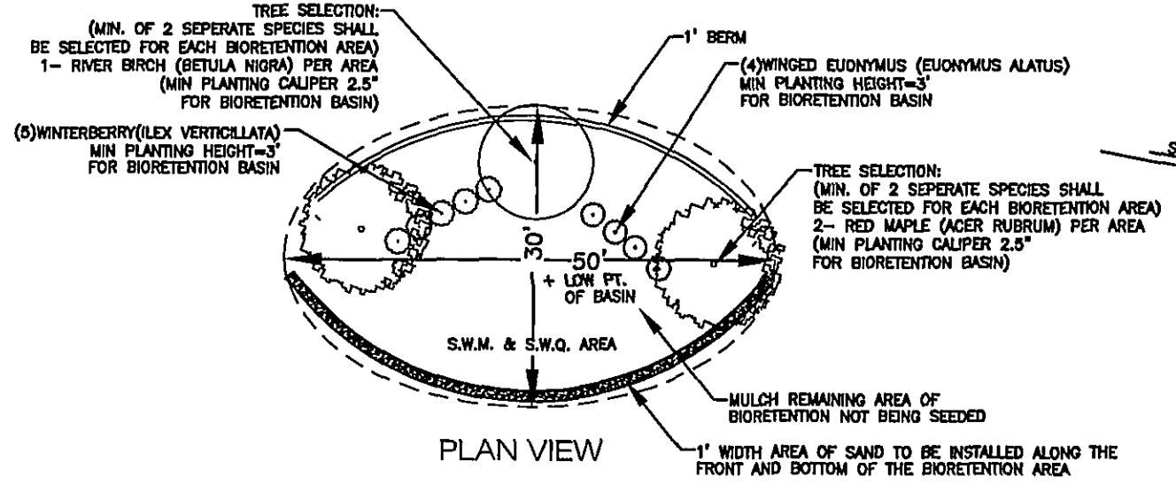
BIOTENTION DETAIL (TYP. LANDSCAPE & CONSTRUCTION DETAILS)
