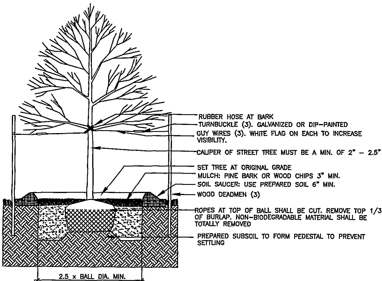
PLANTING DETAIL
