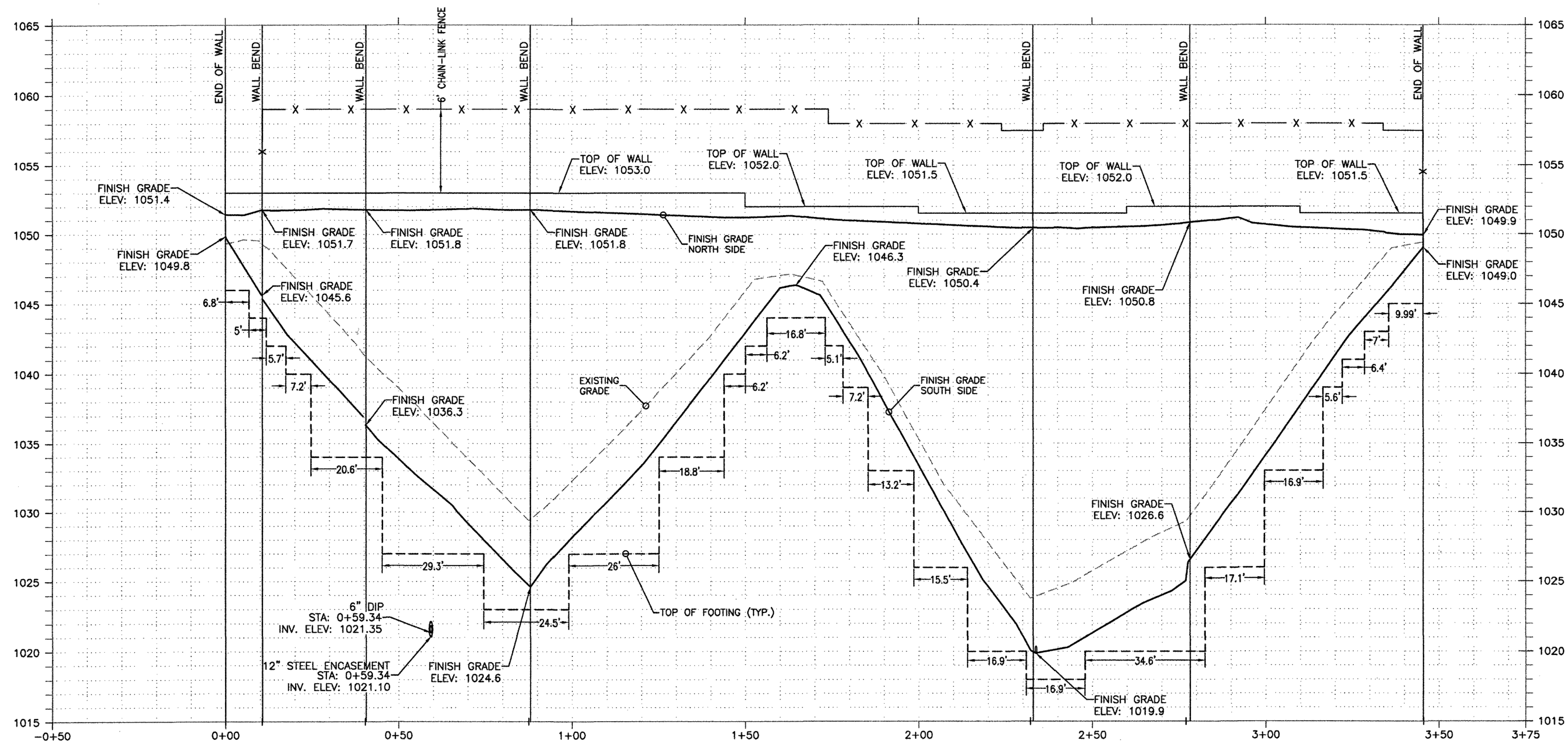
RETAINING WALL 1 VERTICAL SCALE: 1"=5' HORIZONTAL SCALE: 1"=20'
