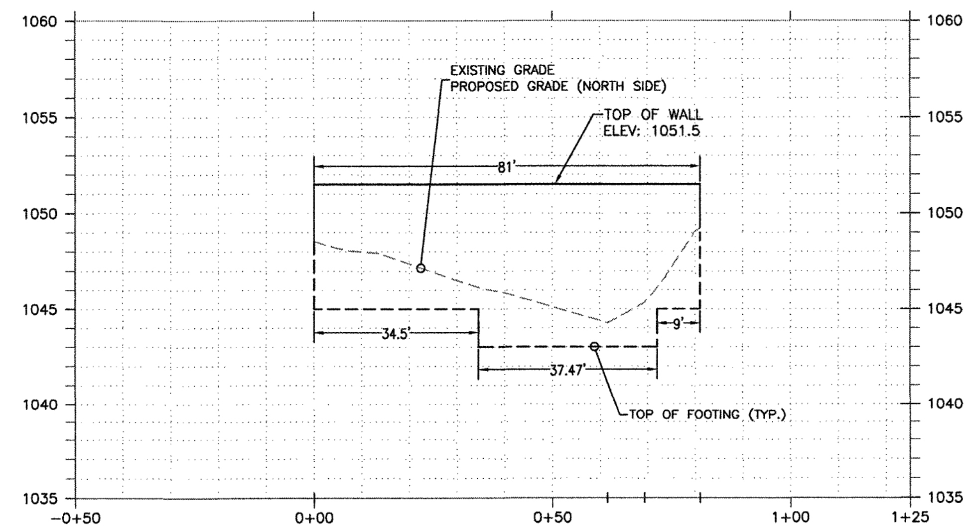
RETAINING WALL 2 VERTICAL SCALE: 1"=5' HORIZONTAL SCALE: 1"=20'
