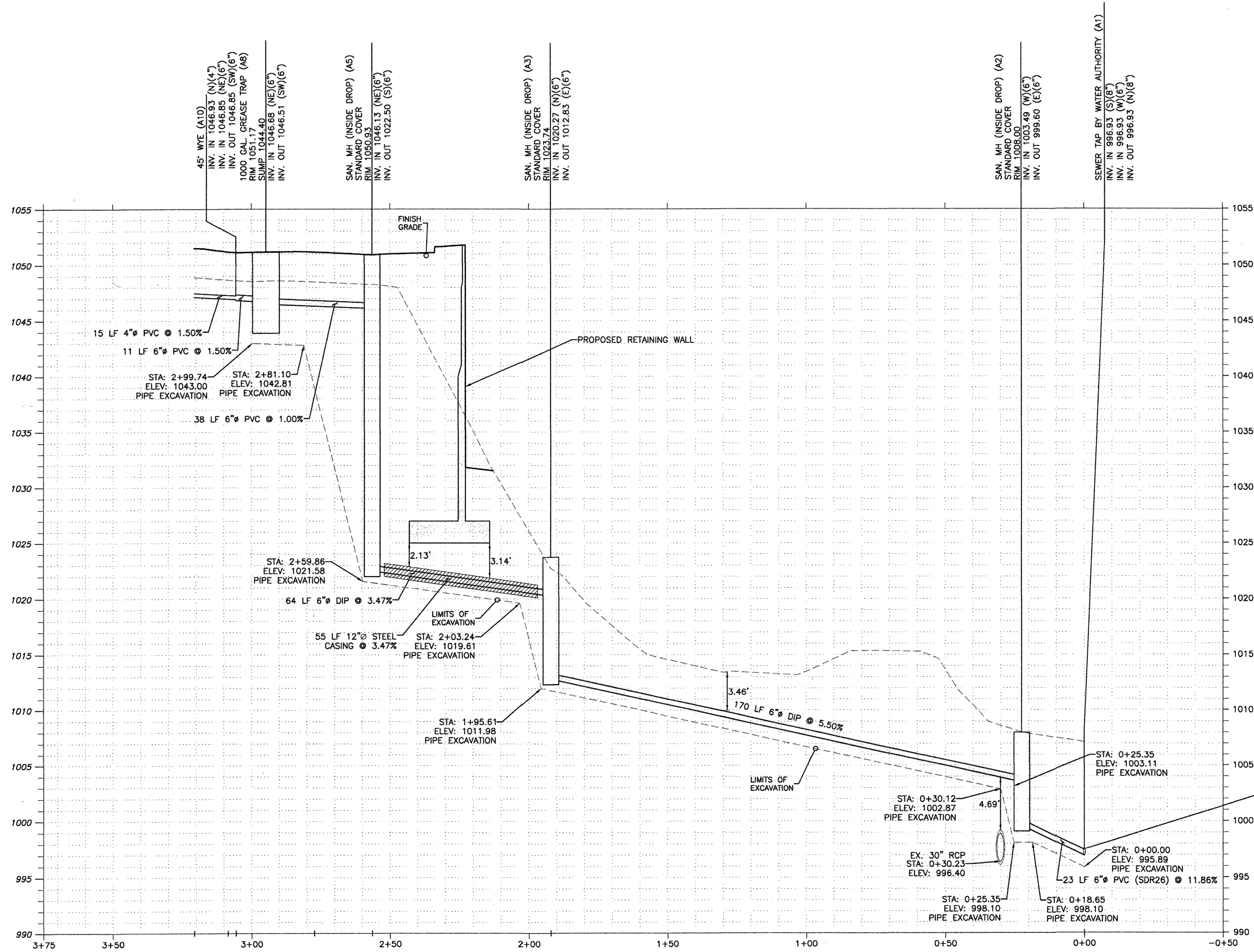
SANITARY SEWER PROFILE A VERTICAL SCALE: 1"=5' HORIZONTAL SCALE: 1"=20'
