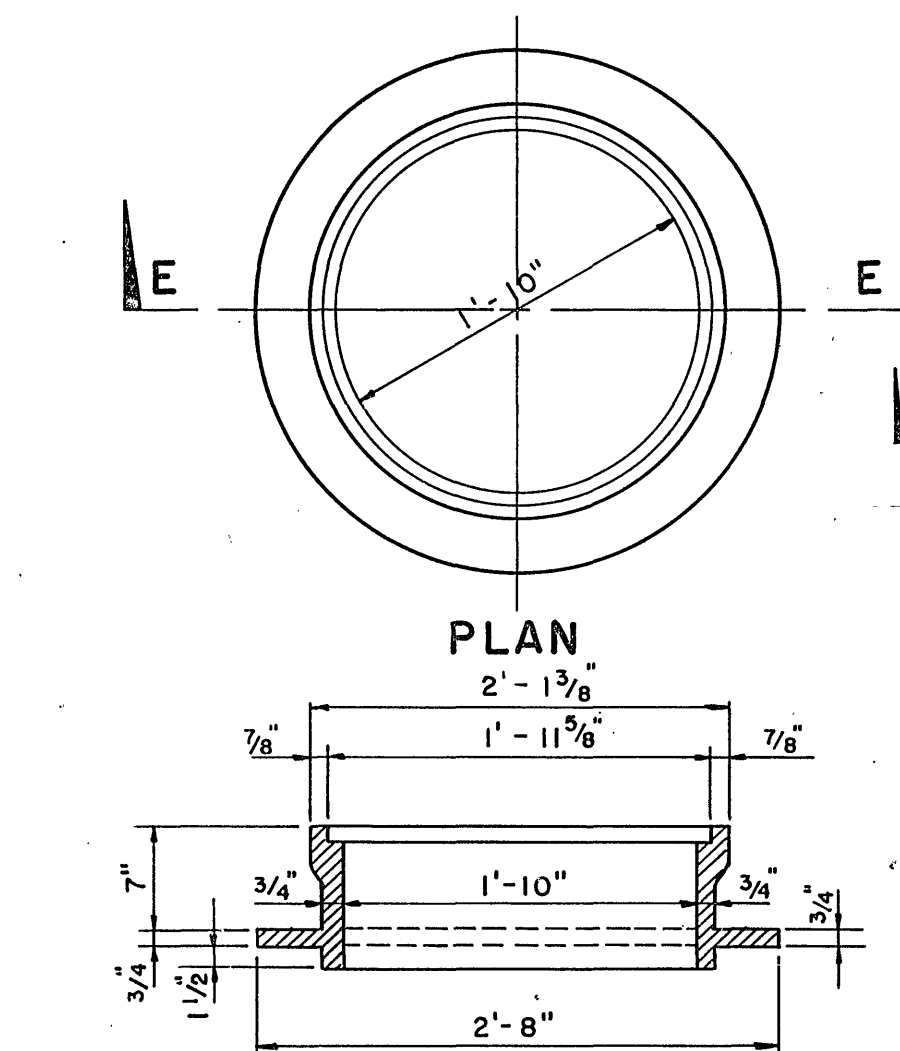
SECTION E-E STANDARD MANHOLE FRAME & COVER SCALE: 1" = 1'-0"
