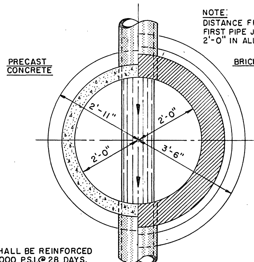
MANHOLE OVER 10' TYPE "A" MANHOLE DETAILS SCALE 1/2" = 1'-0"
