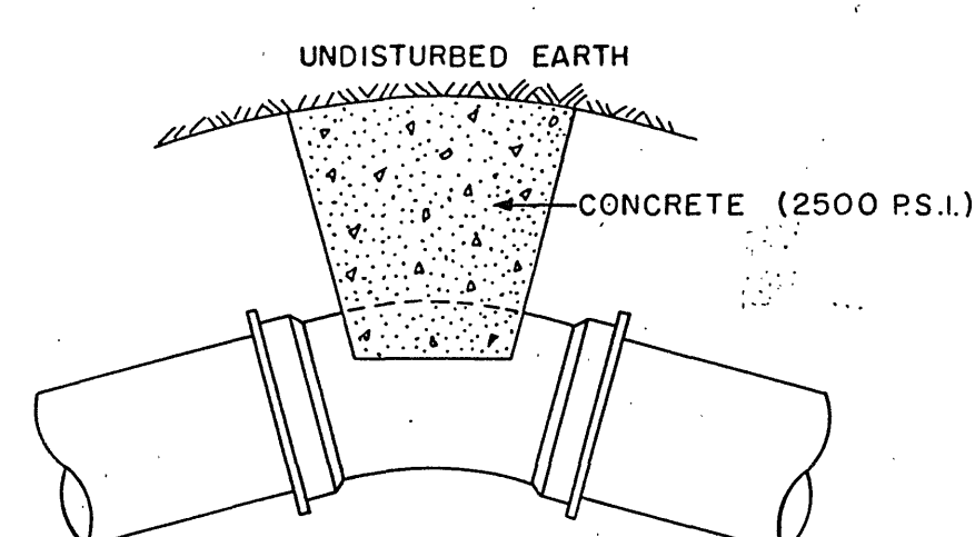
THRUST BLOCK
