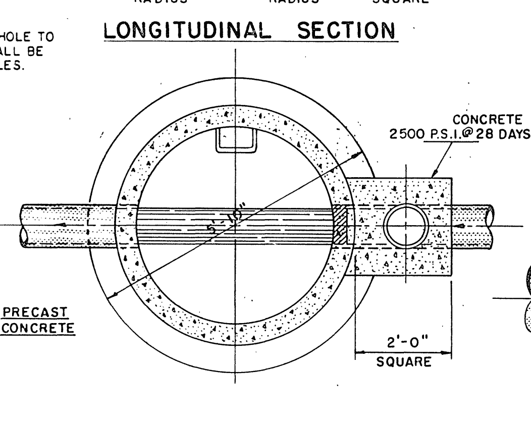
DROP MANHOLE TYPE "B"
