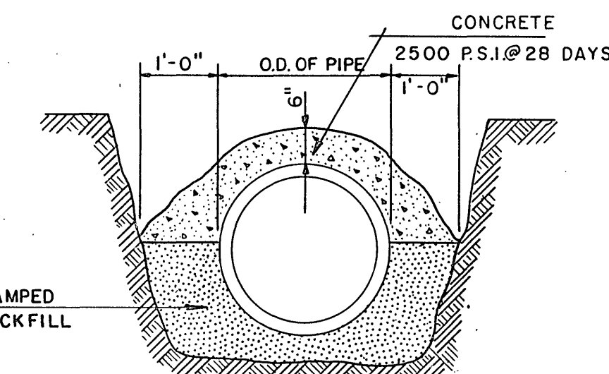
CONCRETE CAP
