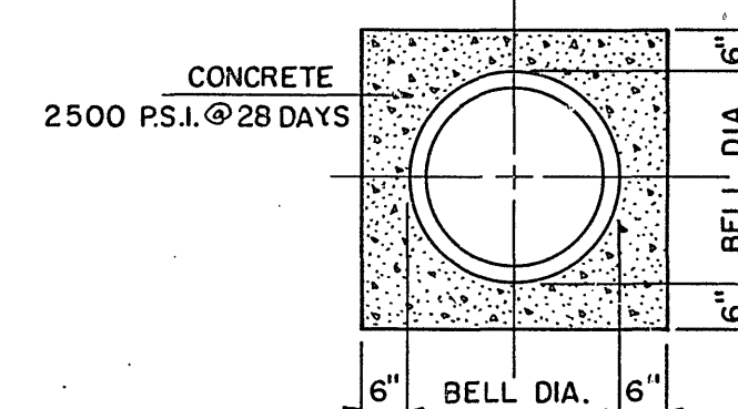
SECTION D-D CONCRETE ENCASUREMENT NOT TO SCALE USE FOR JOINING DIFFERENT TYPES OF PIPE
