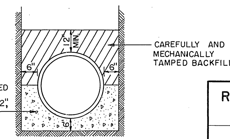
STANDARD GRAVEL BEDDING
