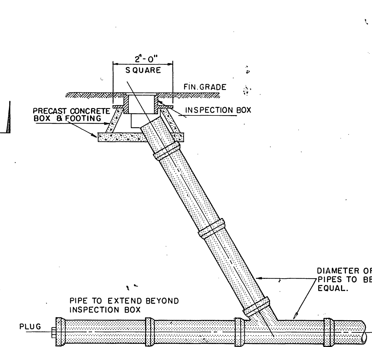
CLEANOUT CONNECTION DETAIL NOT TO SCALE
