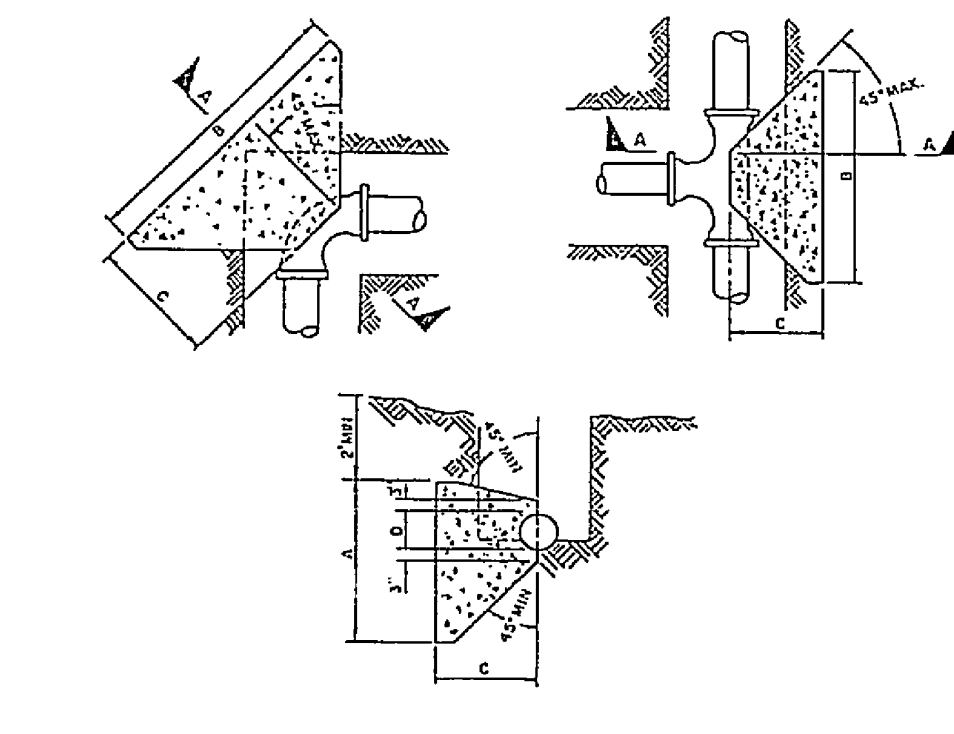
SINGLE RESIDENTIAL WATER SERVICE
