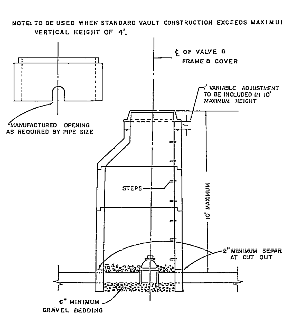
ALTERNATE VALVE VAULT (MANHOLE)
