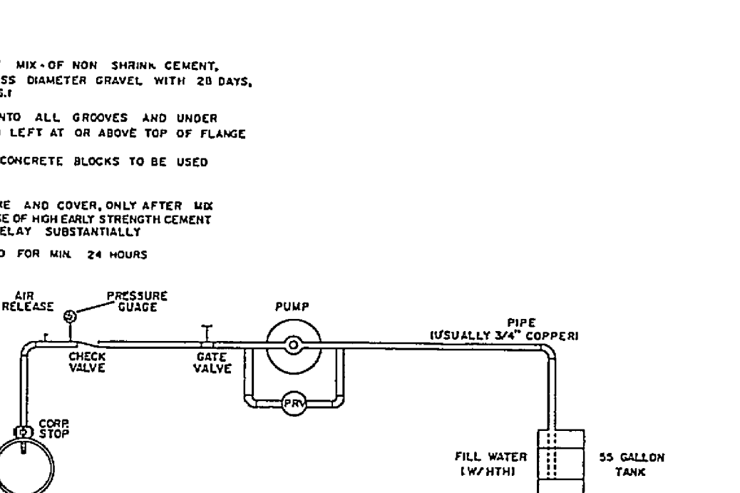
TYPICAL WATER PRESSURE TEST RIG
