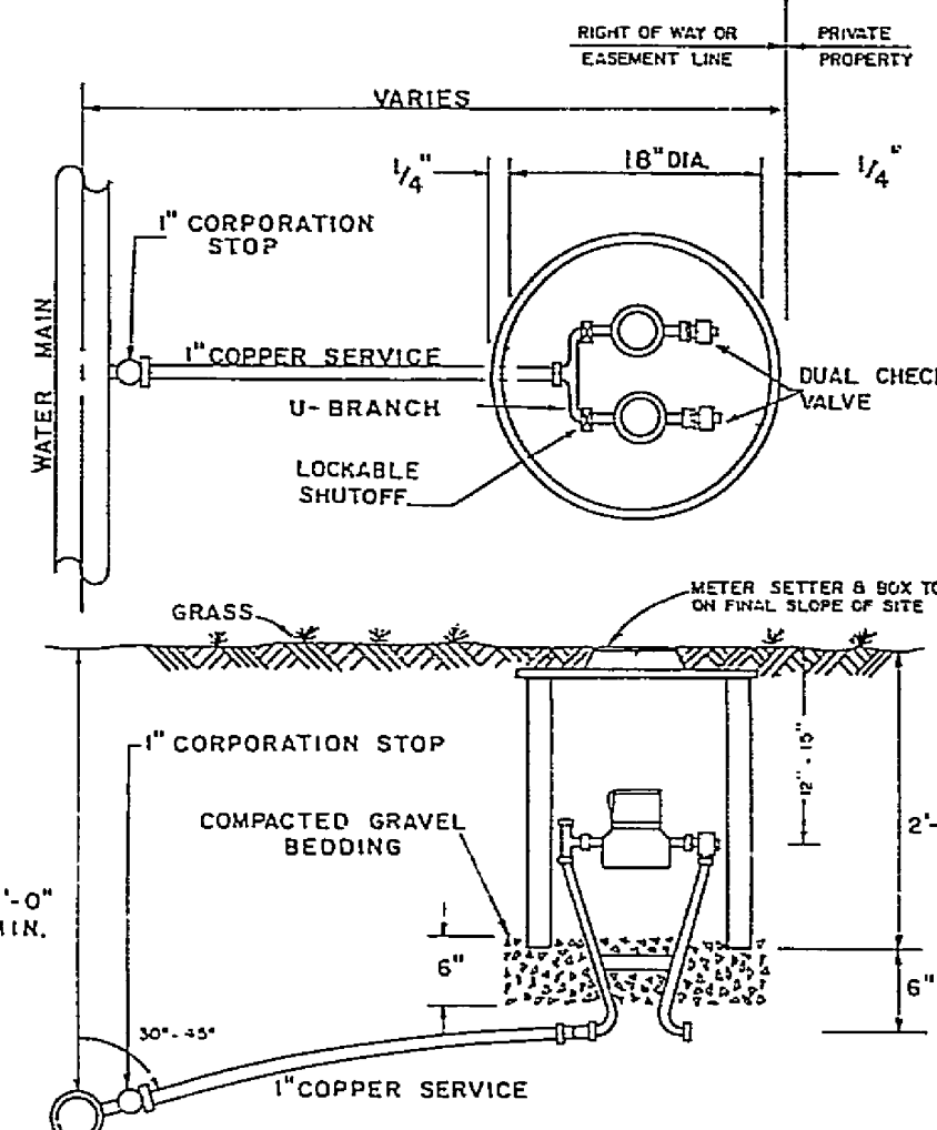
DOUBLE RESIDENTIAL WATER SERVICE
