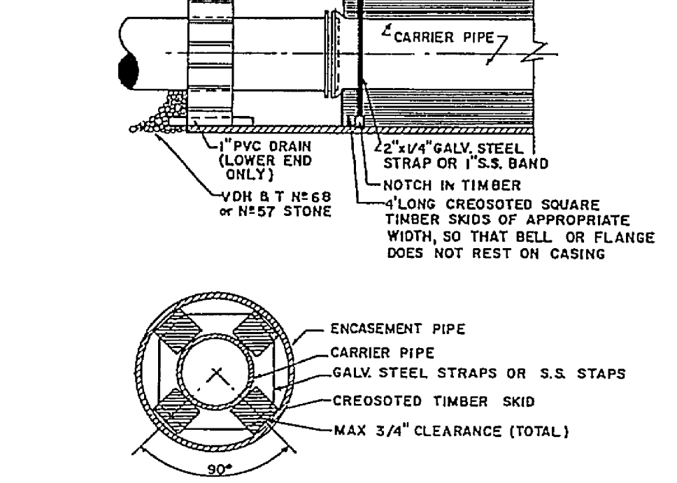
PIPE SUPPORT IN CASING PIPE
