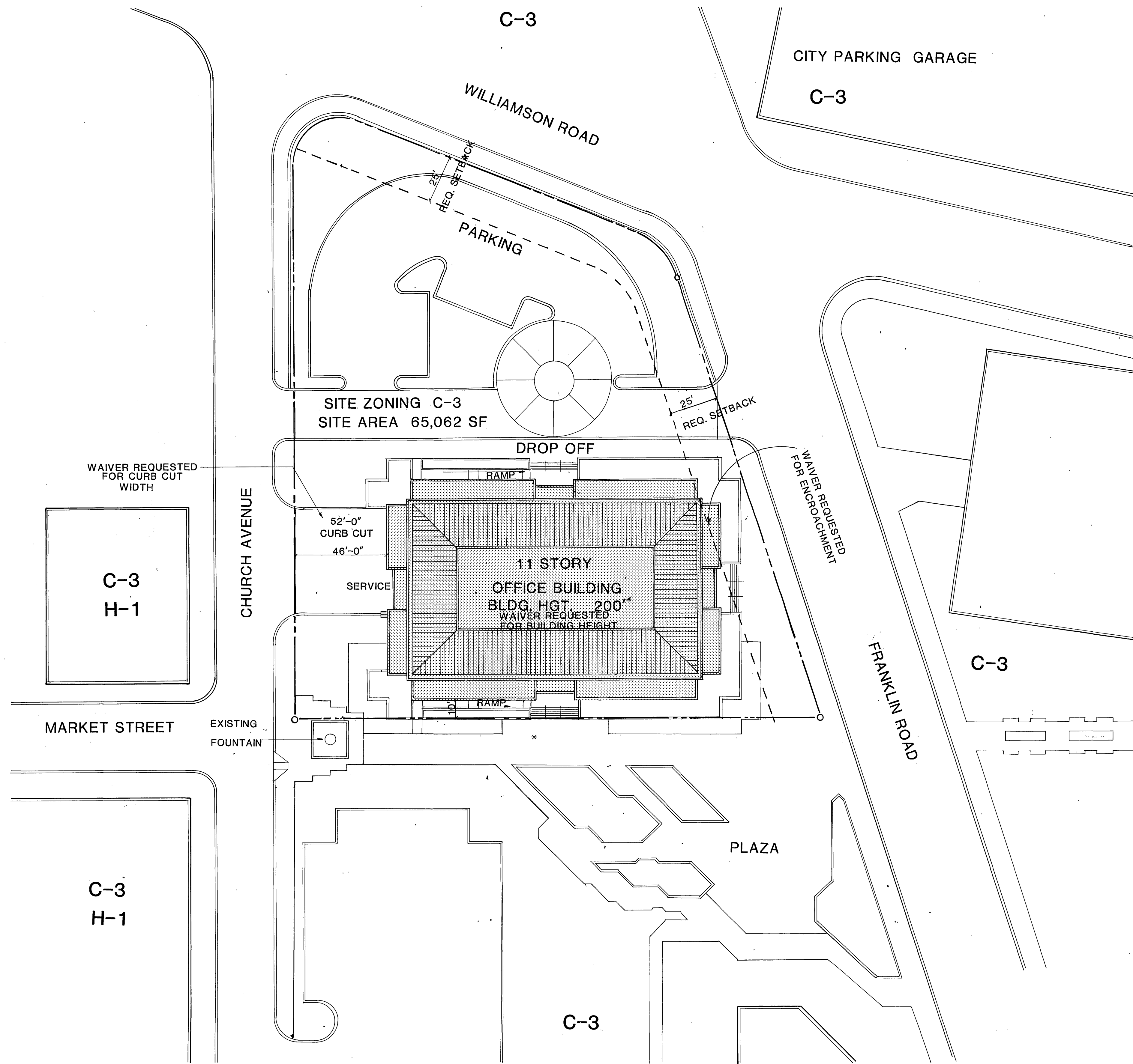
ARCHITECTURAL SITE PLAN
