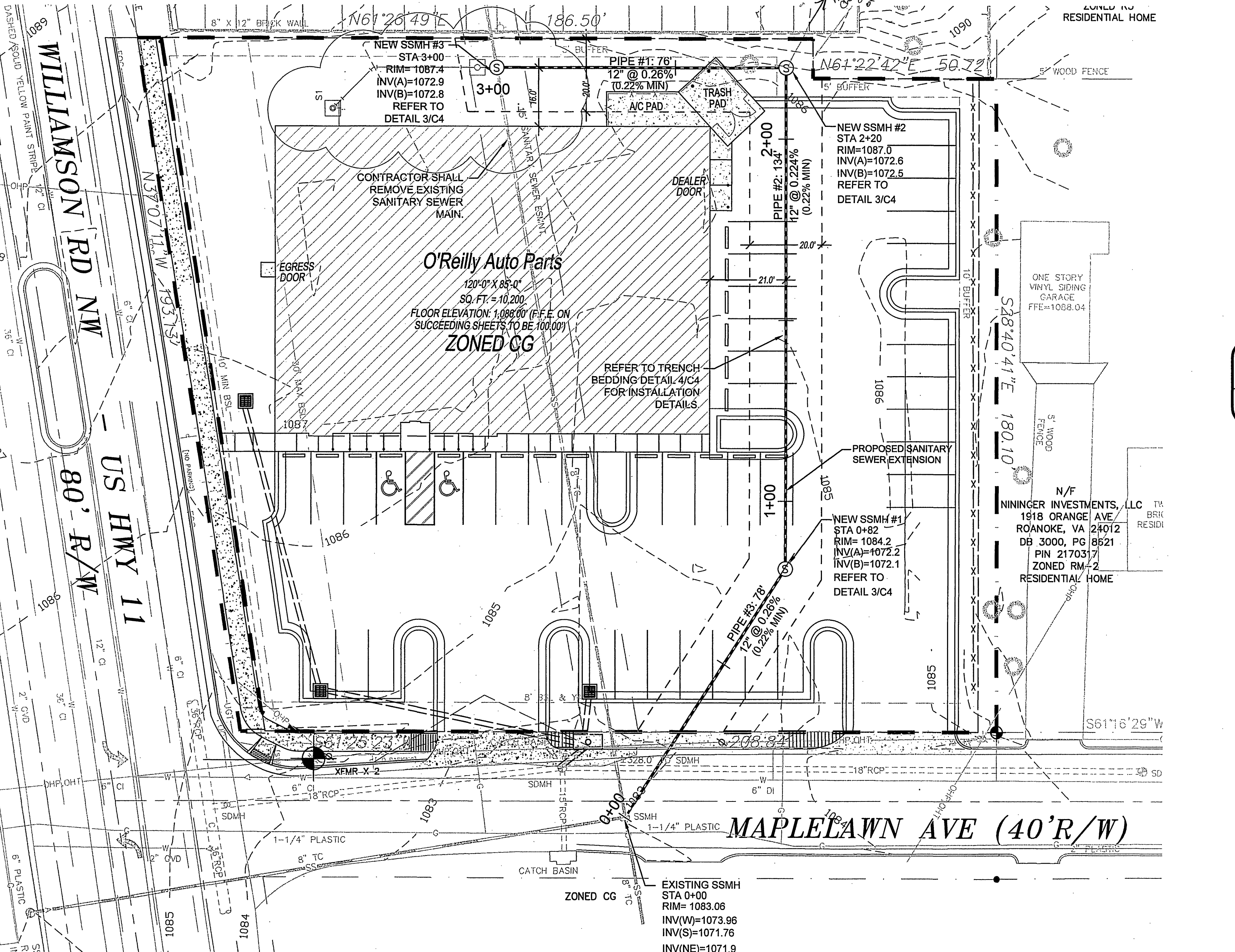
1 SEWER RELOCATION PLAN C4 SCALE: 1" = 20'
