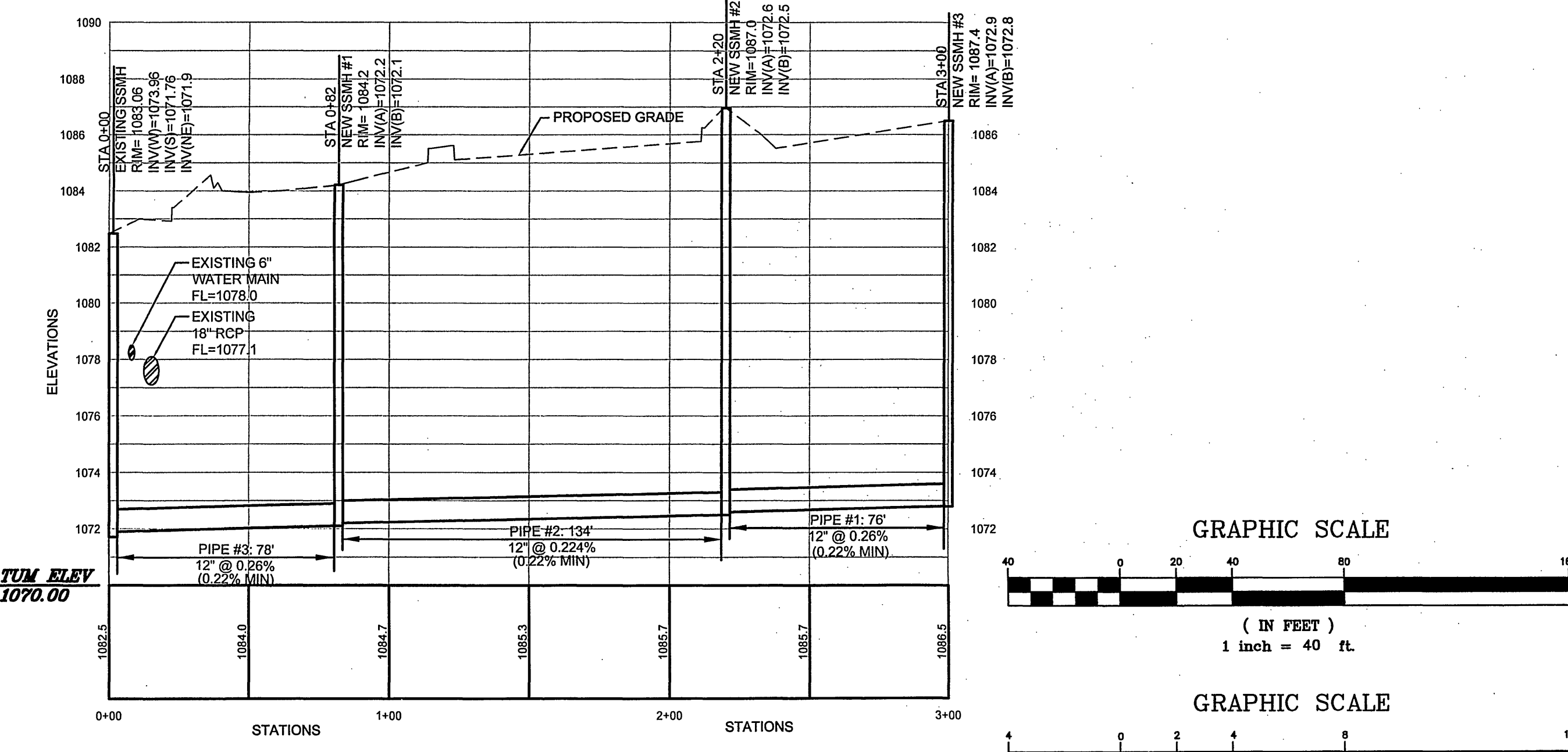
2 SEWER RELOCATION PROFILE C4 SCALE: HORIZONTAL: 1" = 40'; VERTICAL 1" = 4'
