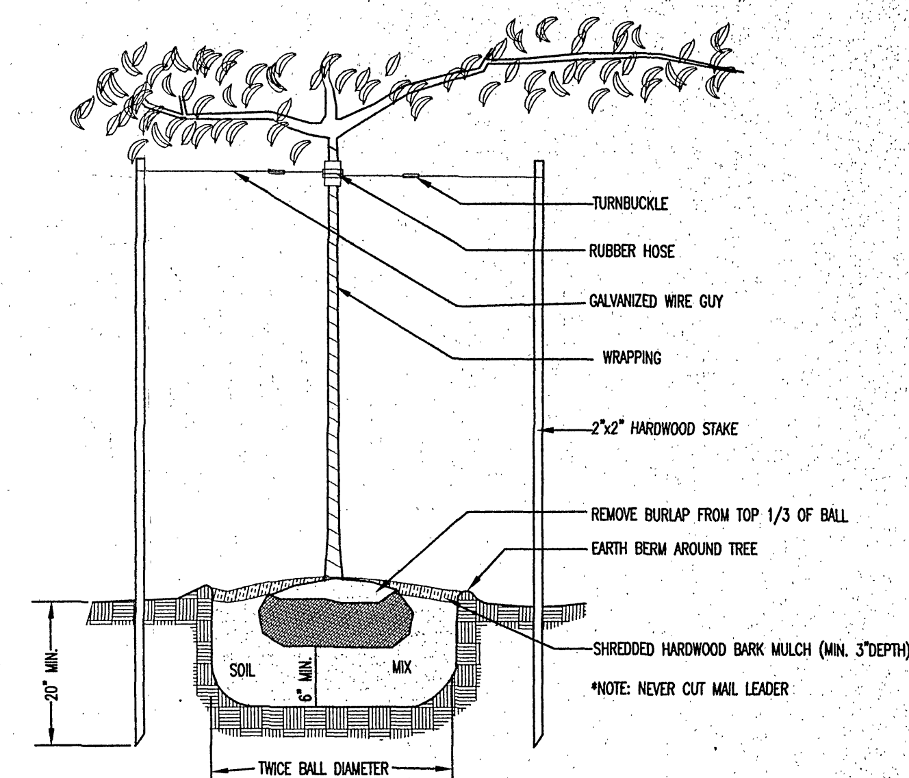
TREE PLANTING DETAIL NOT TO SCALE
