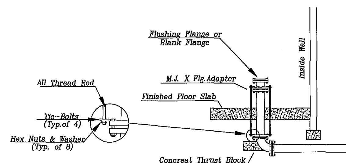
TYPICAL STUB-IN DETAIL
