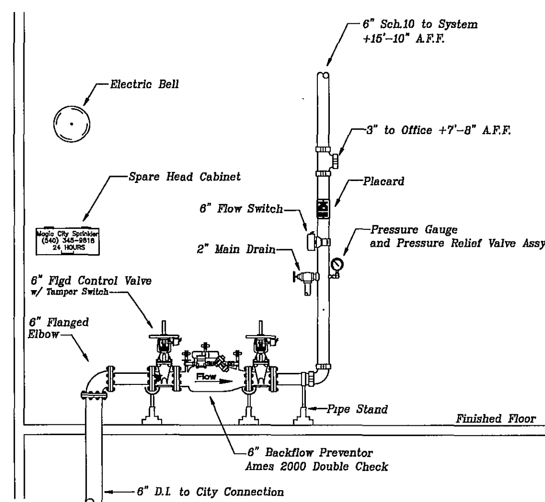
RISER DETAIL
